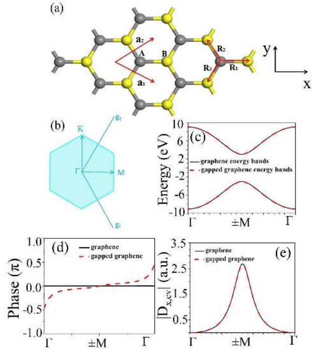
FIG. 1. (a) Hexagonal lattice structure of 2D graphene or gapped graphene. \mathbf{a}_i is the unit vector in real space. The unit cell contains two atoms labeled by “A” and “B”. If both of these two sites are occupied with carbon, the system is graphene. If these two sites are inequivalent, the system becomes gapped graphene. The x and y axes are also indicated. (b) The first Brillouin zone of graphene or gapped graphene. \mathbf{g}_i is the reciprocal lattice vector. High symmetry points, \Gamma , M and K , are labeled. (c) Energy bands of graphene (black solid lines) and gapped graphene (red dashed lines) along the direction of \Gamma -M. The band structures for graphene and gapped graphene are nearly the same. Note that the band structure was presented using the M point at the center. (d) Transition dipole phases (TDP) of graphene (black solid line) and gapped graphene (red dashed line) in the direction of \Gamma -M. The TDP of graphene is zero for all crystal momentum due to the inversion symmetry. In contrast, there exists a non-zero TDP for gapped graphene along the x -axis. (e) Absolute values of transition dipole moments along \Gamma -M direction for graphene (black solid line) and gapped graphene (red dashed line). The behavior of band structure and transition dipole along the y -axis is explained in the text.
