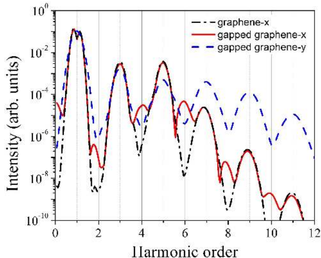
FIG. 2. Calculated HHG spectra for graphene with laser polarized along the x direction (black dash-dotted line), gapped graphene with laser polarized along the x direction (red solid line), and gapped graphene with laser polarized along the y direction (dashed blue line). Laser parameters are 10 fs in FWHM duration, 800 nm in wavelength and 2 \times 10^{12} W/cm 2 in peak intensity.
