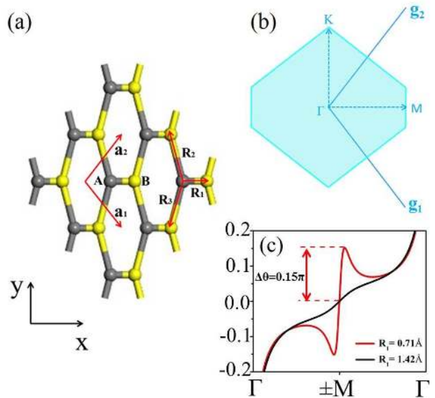
FIG. 5. (a) The real space structure of a deformed gapped graphene with |\mathbf{R}_1|=0.71 Å and |\mathbf{R}_2|=|\mathbf{R}_3|=1.42 Å. (b) The reciprocal space of the deformed gapped graphene. \mathbf{g}_i is the reciprocal lattice vector. High symmetry points, \Gamma , M and K , are labeled. (c) Comparison between the TDP for normal gapped graphene ( |\mathbf{R}_1|=1.42 Å) and deformed gapped graphene ( |\mathbf{R}_1|=0.71 Å).
