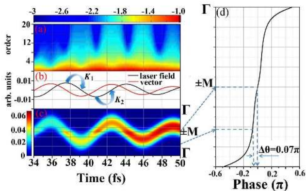
FIG. 4. (a) Time-frequency analysis of HHG from gapped graphene with laser polarized along the x direction. The HHG intensities are depicted on logarithmic scale. (b) The black solid line is the electric field, and the red solid line is the vector potential of the laser field, each is relatively normalized. The two arrows indicate two symmetric electron orbits K_1 and K_2 , see Eq. (30). Electrons are excited into the conduction band at the starting point of the arrow, and recombine to the valence band at the ending point of the arrow with a photon emitted. (c) The time-dependent electron density in the conduction band \rho_c(k, t) . \Gamma and \pm M points are indicated on the right-hand vertical axis. The density is in linear scale shown along the vertical axis on the left. (d) The k -dependent TDP along the \Gamma - M direction ( x direction). The largest difference in TDP ( \Delta\theta ) that an electron orbit can yield is about 0.07\pi . The laser parameters are 2000 nm in wavelength, 25 fs in FWHM and 2 \times 10^{12} W/cm 2 in intensity.
