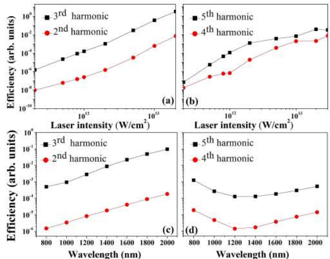
FIG. 3. Dependence of the efficiency of the 2 nd to 5 th harmonic from gapped graphene on laser parameters. The laser is polarized along the x direction (without symmetry). In (a) and (b), the laser wavelength is fixed to be 800 nm while the intensity is tuned from 1 \times 10^{12} to 3 \times 10^{13} W/cm 2 . In (c) and (d), the laser intensity is fixed to be 2 \times 10^{12} W/cm 2 while the wavelength is tuned from 800 nm to 2000 nm.
