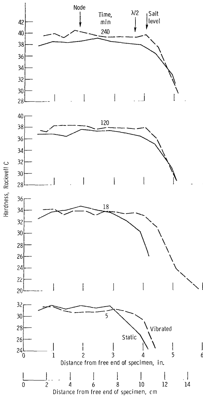
(b) Ultrasonic vibration at 1 mil ( 2.5 \times 10^{-2} mm). Hardness at 0 time: RC 20.0 to 21.8.
