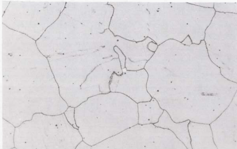
(c) Vibrated at 1.4 mils ( 3.6 \times 10^{-2} mm) for 10 minutes and statically aged for 10 hours at 1600° F (1144 K).
