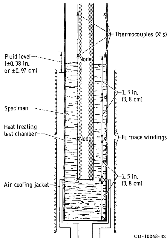
Figure 5. - Schematic diagram showing relative positions of test components, specimen, and thermocouples.
