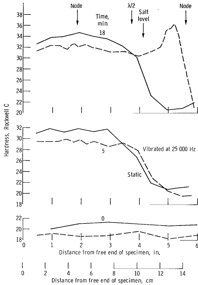
(a) Ultrasonic vibration at 2 mils ( 5.1 \times 10^{-2} mm).
