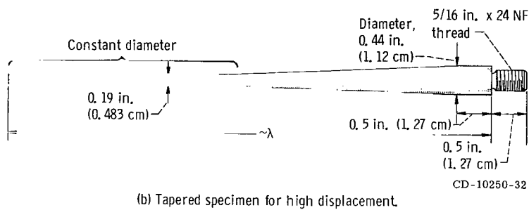
Figure 7. - Specimen designs used for ultrasonic vibration aging studies.
