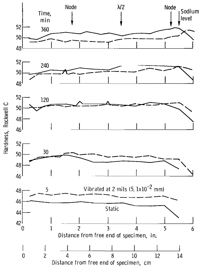
(c) Temperature, 1000° F (811 K). Hardness at 0 time: RC 27.2 to 29.1.
