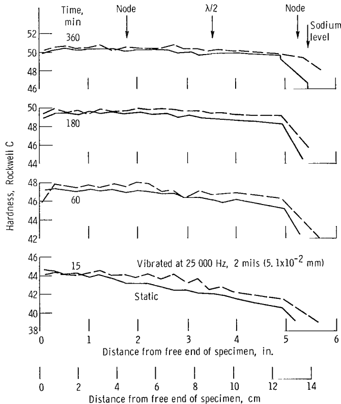
(a) Temperature, 800° F (700 K). Hardness at 0 time: RC 29.6 to 30.8.
