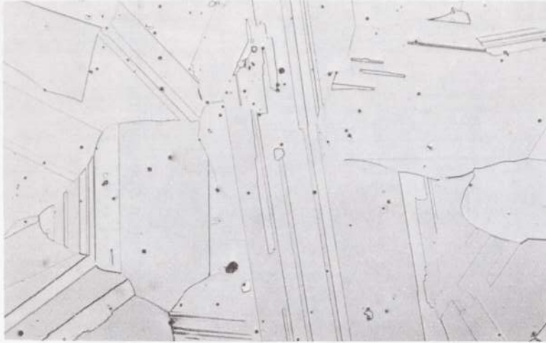
(a) L-605 as received.
