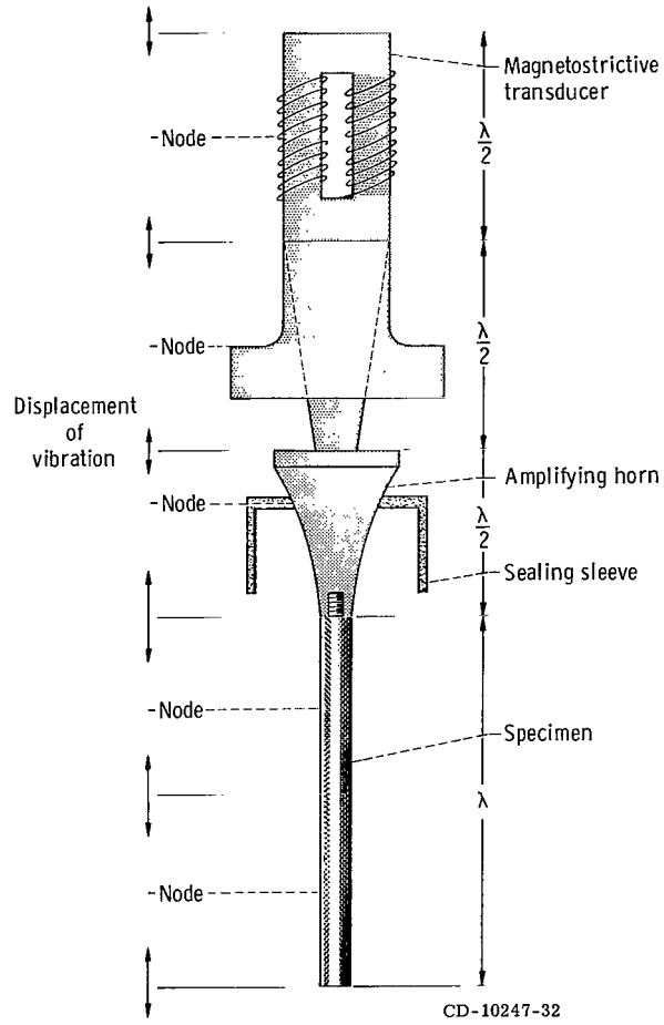
Figure 3. - Schematic diagram of transducer assembly.
