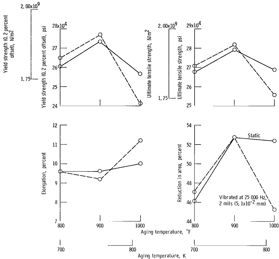
Figure 18. - Room temperature tensile property data of 300 grade maraging steel after aging for 6 hours. Heat treating medium, sodium.
