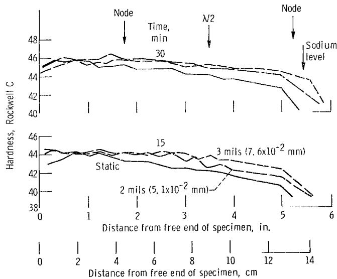
Figure 15. - Comparison of hardness results between static aging and ultrasonic vibration aging at various times at 800° F (700 K) for 300 grade maraging steel. Heat treating medium, sodium. Hardness at 0 time: RC 29.6 to 30.8.
