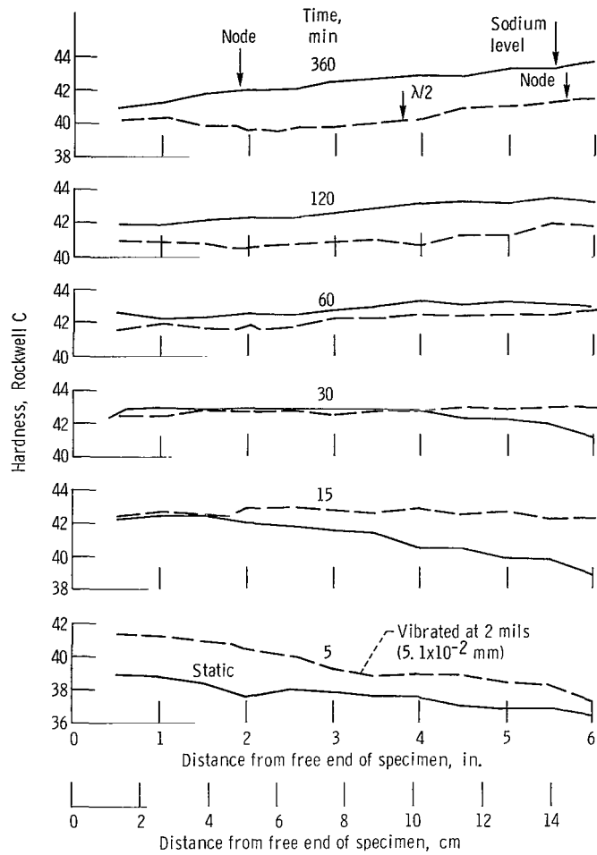
Figure 12. - Comparison of hardness results between static aging and ultrasonic vibration aging at various times at 900° F (755 K) for 17-4 PH steel. Heat treating medium, sodium. Hardness at 0 time: RC 31.9 to 32.6.
