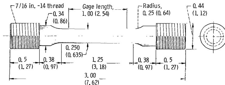
Figure 10. - Standard tensile specimen cut from nodal portion of aged straight bar specimens. (All dimensions in inches (cm).)
