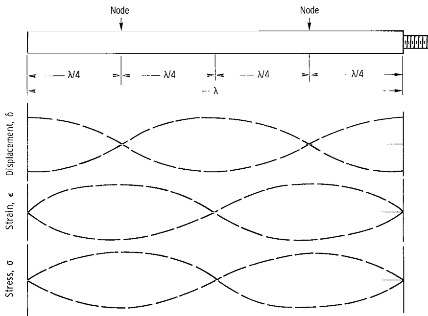
Figure 8. - Specimen displacement, stress, and strain profiles.
