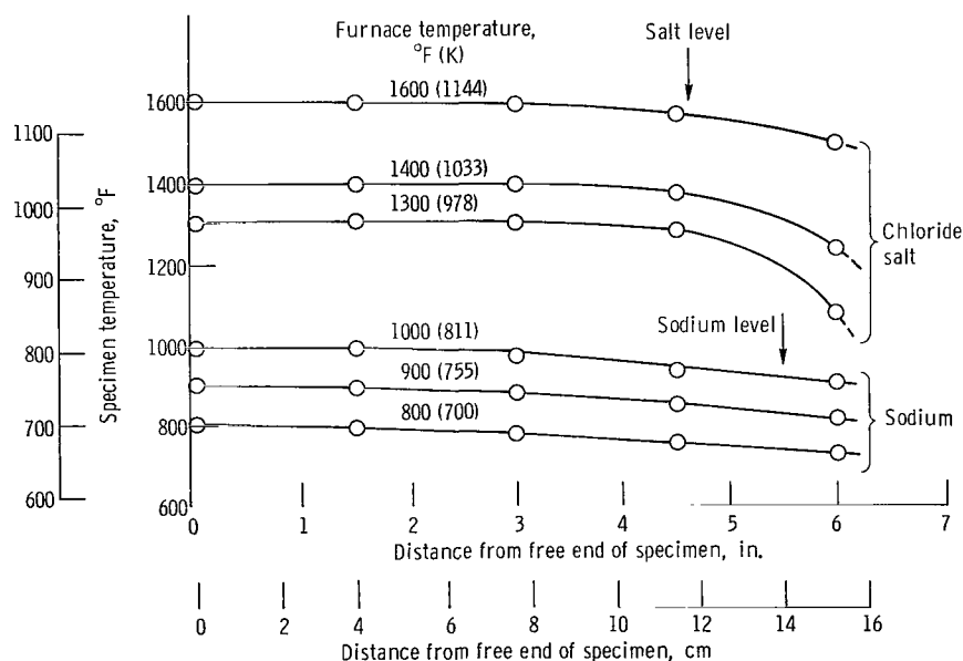
Figure 9. - Typical temperature distributions in static specimens at various furnace chamber temperatures.
