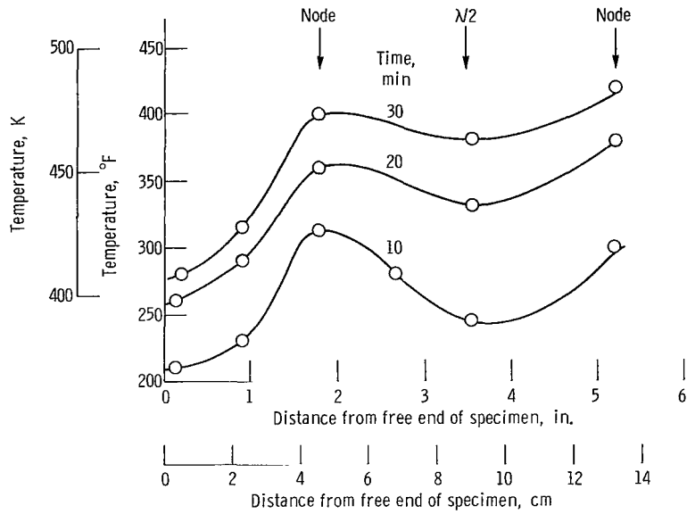
Figure 20. - Temperature profile of 300 grade maraging steel specimen vibrated in air at 25 000 hertz, 2 mils ( 5.1 \times 10^{-2} mm). Temperature measured by infrared pyrometer (lower limit: 200° F or 366 K).
