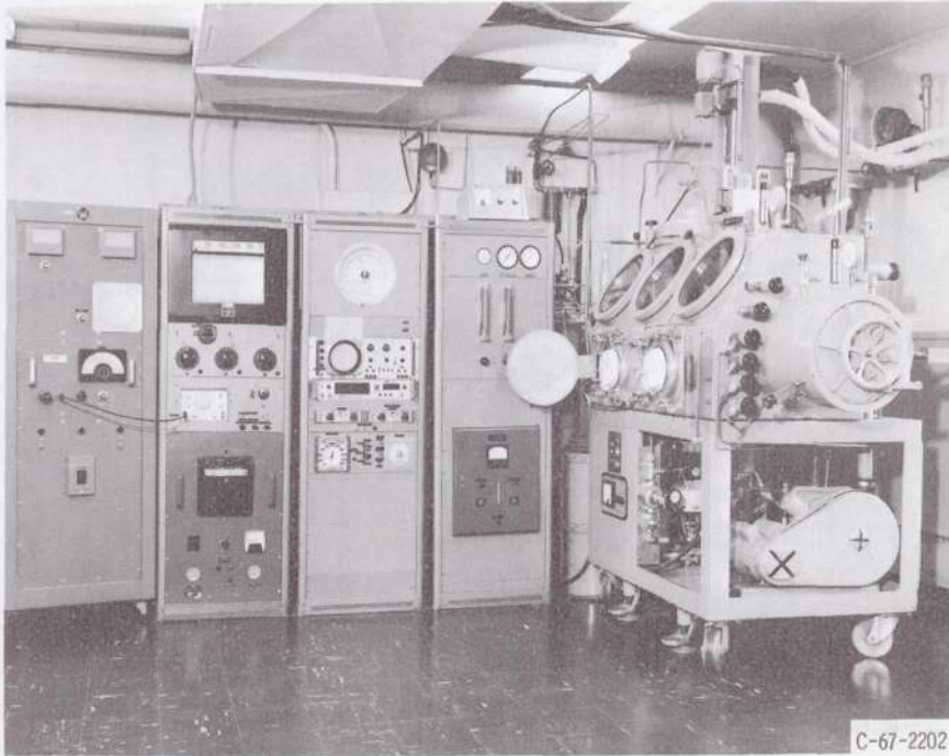
Figure 1. - Ultrasonic vibration heat treating facility.
