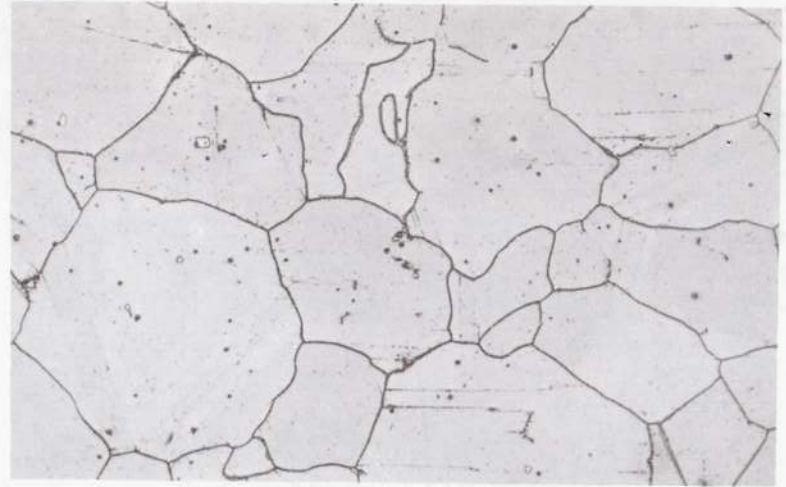
(b) Aged statically at 1600° F (1144 K) for 10 hours.
