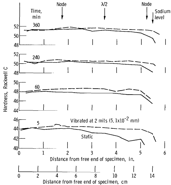
(b) Temperature, 900 o F (755 K). Hardness at 0 time: RC 28.9 to 30.0.
