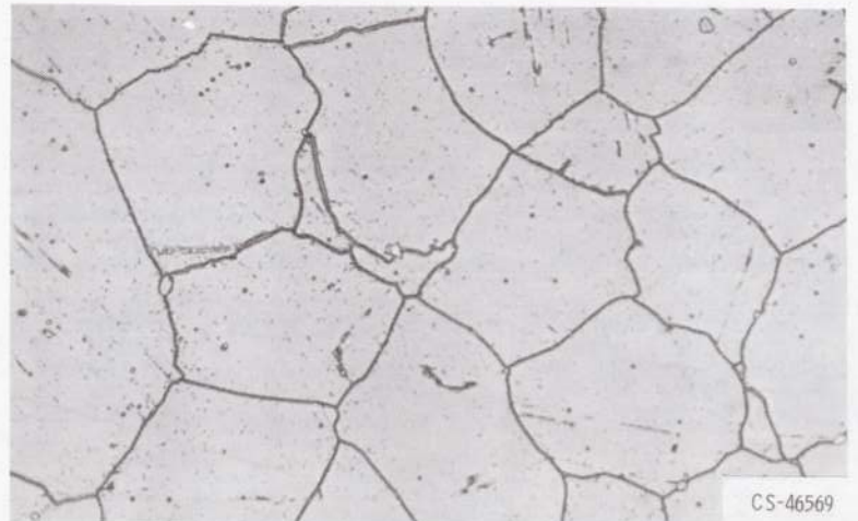
(d) Vibrated at 0.8 mil ( 2.0 \times 10^{-2} mm) at 1600° F (1144 K) for 10 hours.
