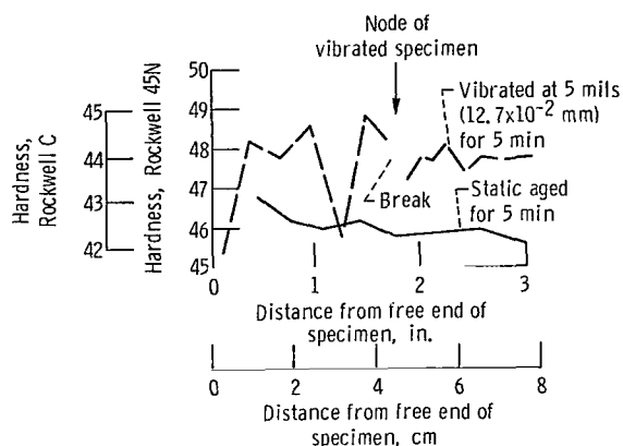
Figure 17. - Hardness results from static aging and ultrasonic aging of tapered specimens of 17-4 PH steel at 900° F (755 K). Heat treating medium, sodium. Hardness at 0 time: Rockwell 45N 38.8 to 39.4.
