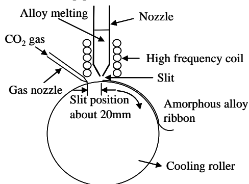
Fig. 1 Scheme diagram of single-roller rapid solidification technique
