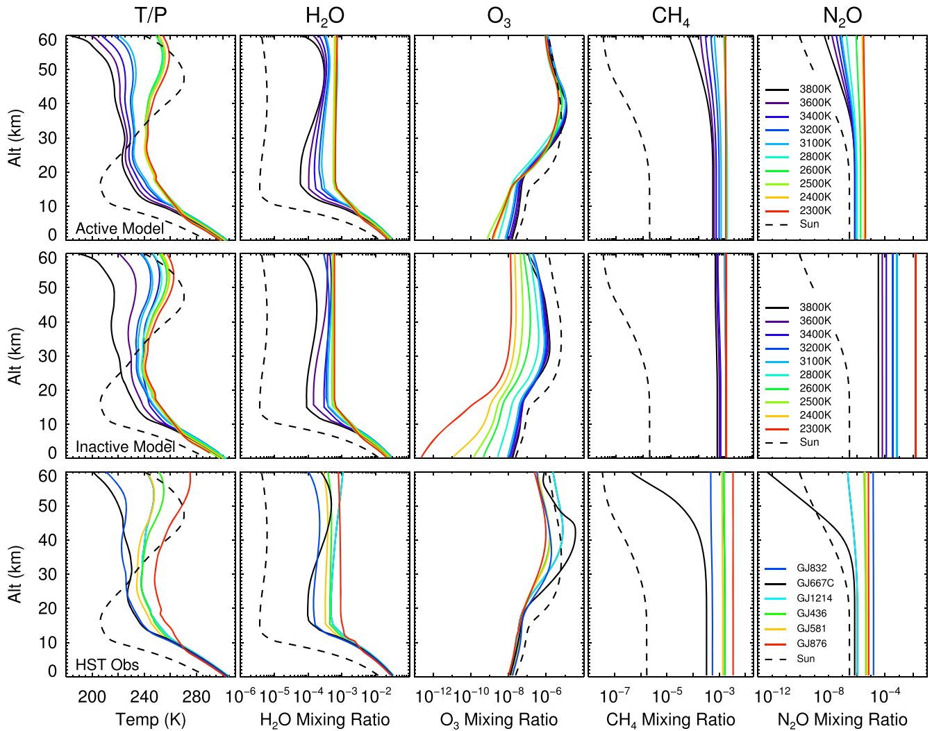
Figure 4. Planetary temperature vs. altitude profiles and mixing ratio profiles for H_2O , O_3 , CH_4 , and N_2O (left to right) for an Earth-like planet orbiting the grid of active stellar models (top), inactive stellar models (middle), and MUSCLES stars (bottom). Earth–Sun profiles are shown for comparison (dashed black lines).
