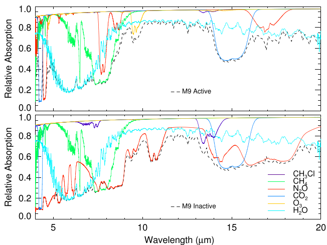
Figure 11. Individual spectral components for \text{H}_2\text{O} , \text{CH}_4 , \text{CO}_2 , \text{CH}_3\text{Cl} , \text{O}_3 , and \text{N}_2\text{O} composing the full IR spectra (shown by a dashed black line) for an Earth-like planet orbiting an M9 active stellar model (top) and M9 inactive stellar model (bottom).
