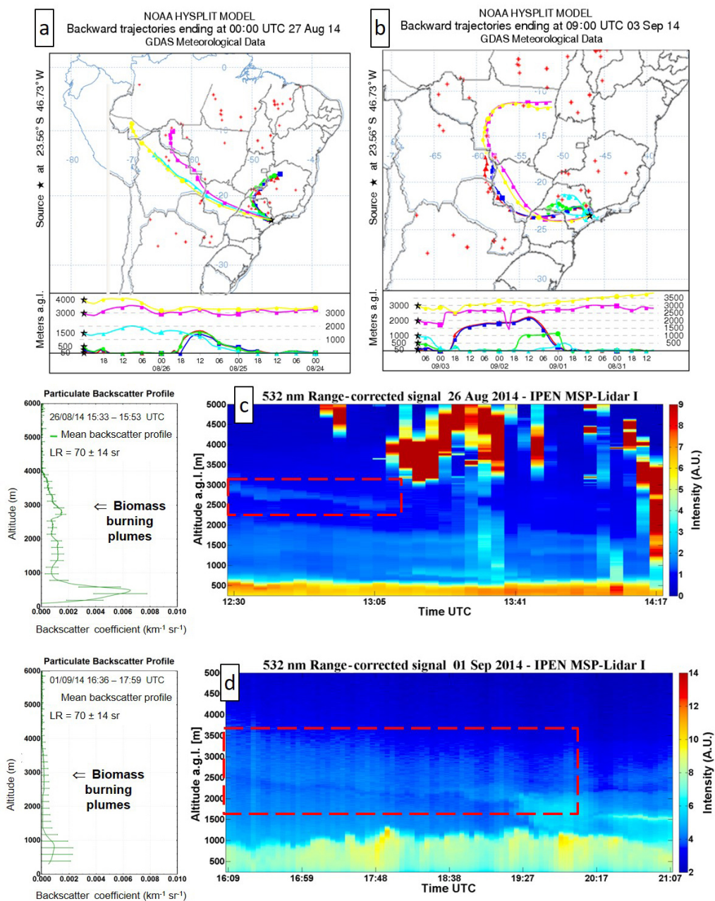
Figure 7. Trajectory and lidar analyses for days with biomass-burning events. (a, b) Hybrid Single Particle Lagrangian Integrated Trajectory (HYSPLIT) trajectory models and biomass-burning events for days 6, 7, 12, 13 and 14. (c, d) The particulate backscatter profile and lidar analyses for days 6 and 12, when the prevailing wind was from the north or northeast, where most biomass-burning events occur. The biomass-burning plumes were detected by lidar and Geostationary Operational Environmental Satellite. NOAA – (United States) National Oceanic and Atmospheric Administration; GDAS – Global Data Assimilation System; a.g.l. – above ground level; IPEN – Instituto de Pesquisas Energéticas e Nucleares ([Brazilian] Nuclear and Energy Research Institute); MSP-Lidar I – Lidar I of the Municipality of São Paulo; LR – lidar ratio.
