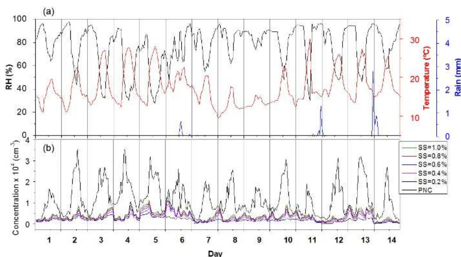
Figure 2. Hourly variability in (a) meteorological parameters such as relative humidity (RH), temperature and rainfall, and also for (b) particle number concentration (PNC) and cloud condensation nuclei (CCN) for the period studied. Note that the PNC corresponds to a size distribution of 9–1000 nm, whereas the CCN correspond to a size distribution of 10–2500 nm.
