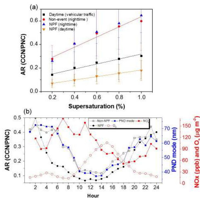
Figure 9. (a) Mean activation ratio (AR) for the daytime (vehicular traffic) and nighttime periods of days with and without new particle formation (NPF) events, by level of supersaturation. (b) Mean hourly AR (at a supersaturation of 0.4 %) on days with and without NPF events, plotted together with particle size mode, nitrogen oxides (NO x ) and O 3 in order to evaluate the effect of vehicular emissions on particle size and AR. The AR values for nighttime and daytime showed clear differences, whereas days with NPF events presented slightly lower values than days without. Two processes contribute to particle size and AR decrease, namely primary aerosol from vehicular traffic (NO x ) and secondary NPF formed in the afternoon. PND – particle number distribution.
