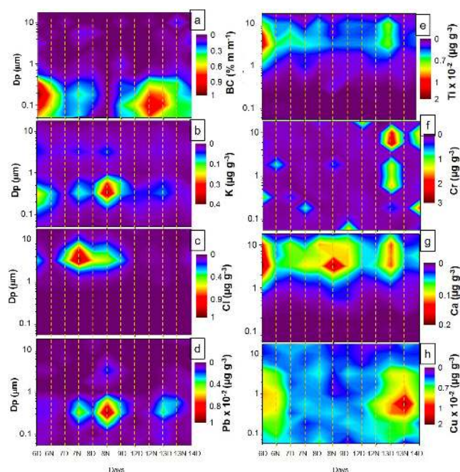
Figure 6. Mass size distribution of elemental concentrations of aerosol samples collected by Micro-orifice Uniform Deposit Impactor (a–h) during the daytime period (07:00–19:00 LT) and nighttime period (19:00–07:00 LT), represented by D and N, respectively. All sampling days were weekdays.
