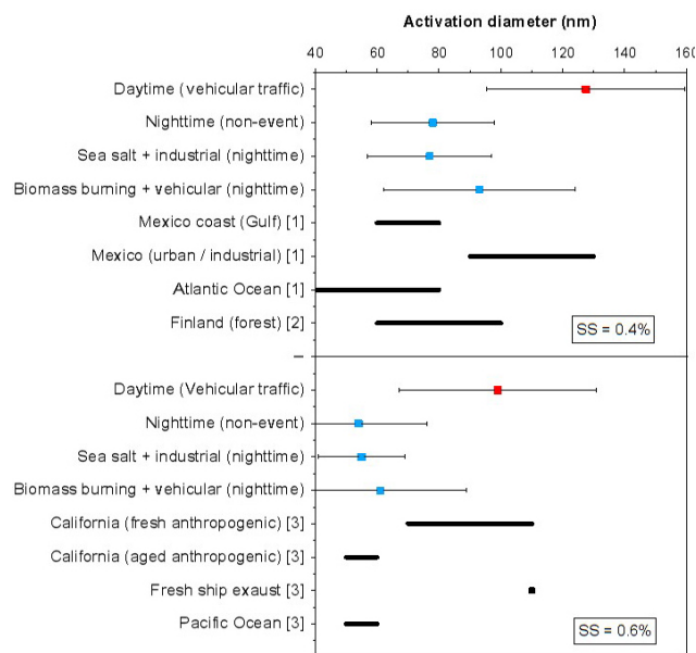
Figure 11. Comparison of apparent activation diameter ( D_{act} ) values obtained in this and previous studies, conducted in urban, coastal and forest environments. Mean values for air masses determined to have been influenced by sea-salt transport and biomass-burning plumes were calculated for nighttime periods. SS – supersaturation; [1] Quinn et al. (2008); [2] Sihto et al. (2011); [3] Furutani et al. (2008).
