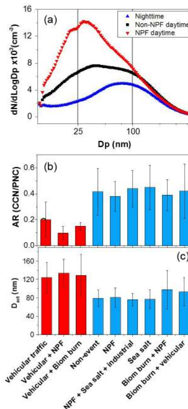
Figure 12. (a) Mean daytime and nighttime particle size. (b) Mean daytime and nighttime activation ratio (AR), during new particle formation (NPF), vehicular traffic, remote source events and non-event periods. (c) Mean daytime and nighttime apparent activation diameter ( D_{\text{act}} ) during NPF, vehicular, remote source events and non-event periods. The AR and D_{\text{act}} were calculated for a supersaturation of 0.4 %. Biom burn – biomass burning; PND – particle number distribution.
