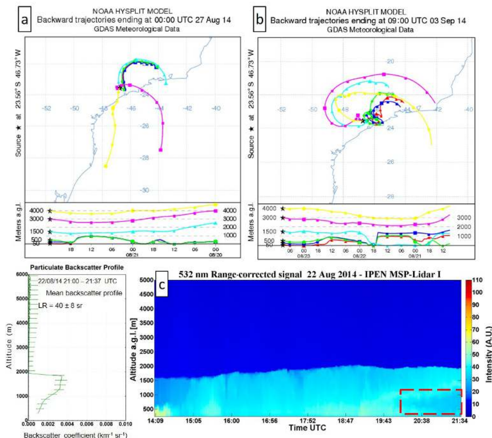
Figure 8. Trajectory and lidar analyses for days with sea-salt apportionment. (a, b) Hybrid Single Particle Lagrangian Integrated Trajectory (HYSPLIT) trajectory models for days 3, 4 and 5. (c) Particulate backscatter profile and lidar analyses for days 3 and 4, when the prevailing wind was from the south, southeast or southwest (i.e., from the Atlantic Ocean and coastal regions). Sea-salt plumes were detected by lidar analysis on day 4, although higher confidence interval concentrations were observed on days 7 and 8. NOAA – (United States) National Oceanic and Atmospheric Administration; GDAS – Global Data Assimilation System; a.g.l. – above ground level; IPEN – Instituto de Pesquisas Energéticas e Nucleares ([Brazilian] Nuclear and Energy Research Institute); MSP-Lidar I – Lidar I of the Municipality of São Paulo; LR – lidar ratio.
