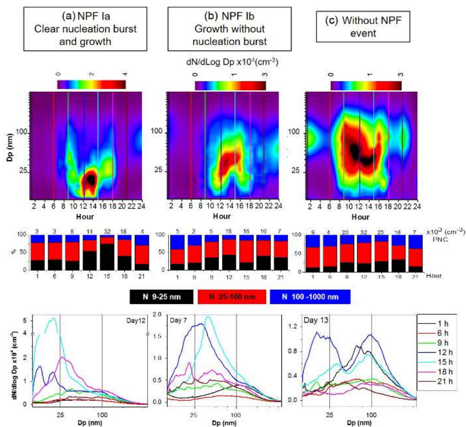
Figure 5. Particle number distribution (PND) contour plots for days with (a) new particle formation (NPF) events categorized as class Ia; (b) class Ib NPF events; and (c) no NPF events. The hourly bars show the proportions of particle number concentrations (PNCs) in three modes (nucleation, Aitken and accumulation) and hourly line graphs show PND distribution. Selected hours were marked on the PND contour plots in order to compare them with the hourly PND line graphs.
