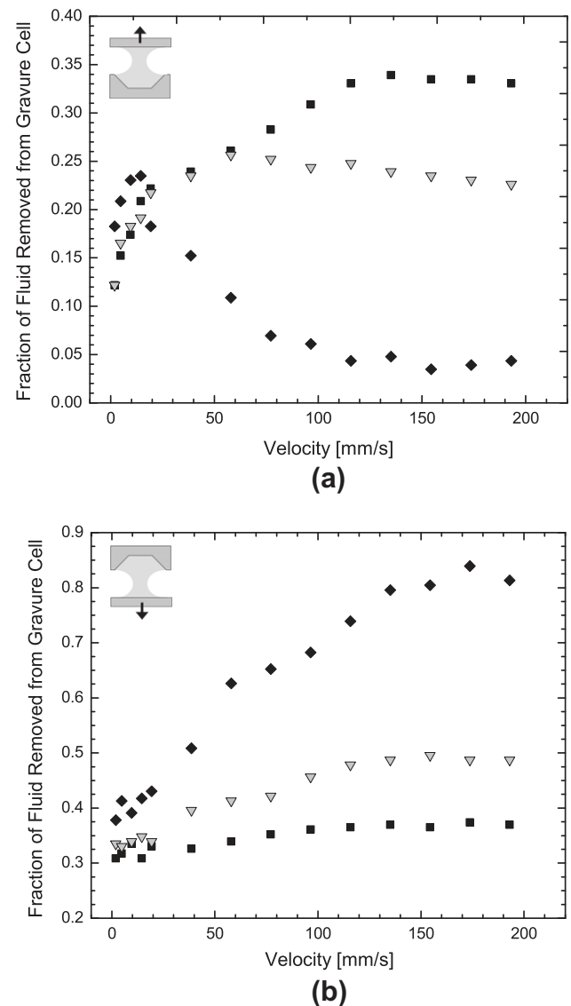
Fig. 15. Fraction of fluid removed from the gravure cell (pickout) as a function of velocity for the shallow ( h/R = 0.1 ) gravure cell. The data include: (■) 20% 20K PEO, (▼) 2M PEO and (◆) 8M PEO for configuration where the gravure cell is placed on (a) the bottom plate and with the top plate moving and (b) the top plate with the bottom plate moving.
