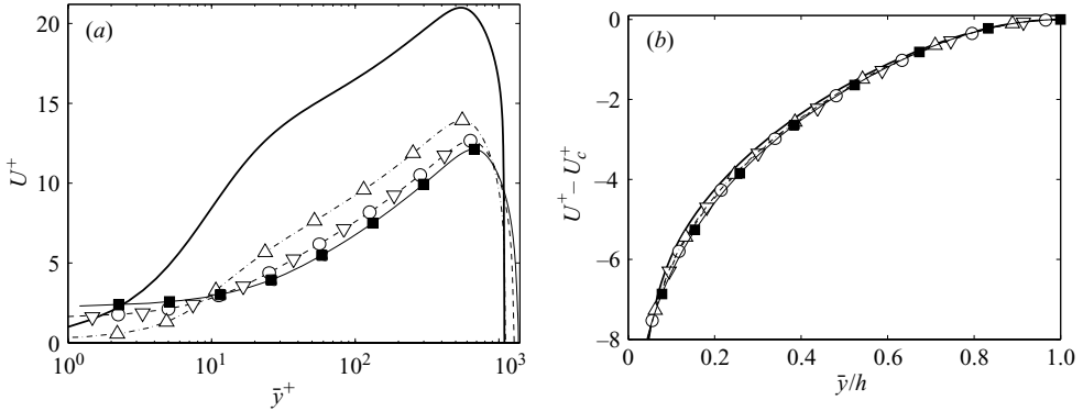
FIGURE 1. (a) Mean streamwise velocity. (b) Streamwise velocity defect law, U_c = U(y = h) . —, S0; \triangle , r1; \nabla , r2; \circ , R2; \blacksquare , r3.
