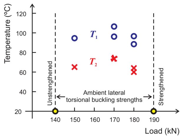
Fig. 6 - The failure temperatures for strengthened beams carrying different loads.
