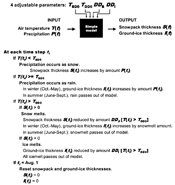
FIGURE 4. Snowpack model schematic.
