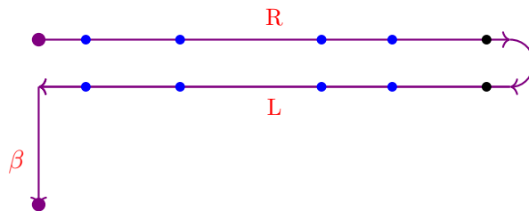
Figure 1. An illustration of the hydrodynamic observables in the Schwinger-Keldysh functional integral phrased in the Keldysh average-difference basis. Response functions are correlators of a sequence of difference operators (the external disturbances, denoted as blue dots) followed by an average operator (the measurement, denoted by the black dots) in the future.
