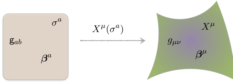
Figure 3. Illustration of the data for hydrodynamic sigma models as described in [2]. The physical degrees of freedom are captured in the target space maps X^\mu(\sigma) which are the hydrodynamic pion fields. The worldvolume geometry is equipped with a reference thermal vector field \beta^a , which pushes forward to the physical thermal vector in spacetime, while the spacetime metric pulls back to the worldvolume metric g_{ab} .
