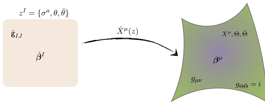
Figure 4. Illustration of the data for hydrodynamic sigma models. The physical degrees of freedom are captured in the target space maps \hat{X}^\mu(\sigma, \theta, \bar{\theta}) , along with the gauge condition which aligns the Grassmann coordinates in target space with their worldvolume counterparts \Theta = \theta and \bar{\Theta} = \bar{\theta} . The worldvolume geometry is equipped with a reference super-vector field \hat{\beta}^I , which pushes forward to the physical thermal vector in spacetime, while the spacetime metric g_{\mu\nu} (with g_{\Theta\bar{\Theta}} = i ) pulls back to the worldvolume metric \hat{g}_{IJ} . The pullbacks and pushforwards are U(1)_\Gamma gauge covariant, since the worldvolume dynamics is constrained by this symmetry.
