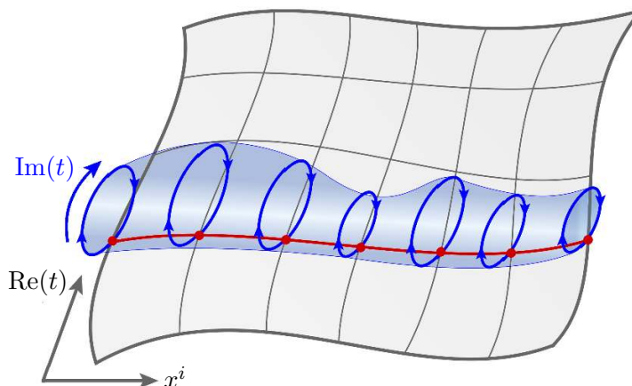
Figure 2. Illustration of the spacetime picture associated with the proposed KMS gauge invariance, with the figure taken from [6]. We upgrade the spacetime manifold (a Lorentzian geometry, depicted in gray, with a typical Cauchy slice indicated in red), on which our quantum system resides to a thermal fibre bundle. We further assume local thermal equilibrium (as in, e.g., hydrodynamics) at each spacetime point which guarantees existence of a thermal vector \beta^\mu . We draw this vector field as a circle fibration with a thermal circle whose size is set by the local temperature. The KMS transformations we seek implement equivariance with respect to thermal translations along this local imaginary time circle. Restricting to a gauge slice corresponds to picking a Lorentzian section of this fibration. Note that the size of the thermal circle is exaggerated; our arguments assume the high temperature limit where the size of the thermal circle is much smaller than the fluctuation scale.
