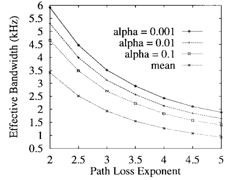
Fig. 3. Effective bandwidths for Type 2 standard mobile ( W = 1 MHz, Chernoff bound: heterogeneous).
