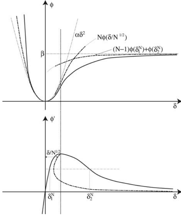
Fig. 1. Example of an interplanar potential of the Lennard-Jones type, which displays only one inflexion point separating convex and concave regions. For this simple case, a straightforward analysis proves the uniform convergence of P_N(\sqrt{N}\delta) and its derivative with respect to \delta to the universal form \min\{\alpha\delta^2, \beta\} , for \delta \geq 0 , and its derivative, respectively. A sketch of P_N(\sqrt{N}\delta) for a particular value of N is shown in the top figure. Also shown is a graphical representation of the solution of equation (1). Given a value of \delta/\sqrt{N} , the values of \delta_1^N and \delta_2^N are determined by finding the horizontal line that leaves the point(s) in the dashed curve at a distance \delta/\sqrt{N} from the \delta = 0 axis.
