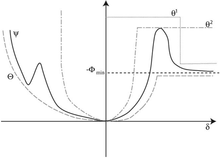
Fig. 2. Schematic representation of the construction of upper and lower potentials. A typical interplanar potential is shown in a solid line. Note the asymptotic behavior as \delta \rightarrow +\infty and the possibility of having multiple inflexion points, local minima and maxima. Possible choices of upper and lower potentials are shown in dashed lines.
