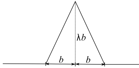
Figure 1: A spike function.
