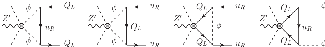
Figure 5. Representative Feynman diagrams contributing to the mixing of the operators O_Q^{ij} , O_u^{ij} , O_d^{ij} and O_\phi . These graphs must be supplemented by external-leg corrections (not shown).
