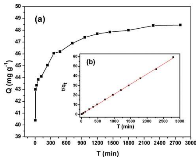
Fig. 6 Kinetics of Cr(vi) adsorption onto the \beta -CCWB450 at 298.15 K. (a) Cr(vi) sorption kinetics data, (b) pseudo-second-order model for Cr(vi) adsorption (initial Cr(vi) concentration 100 \text{mg L}^{-1} ; pH = 2.0).
