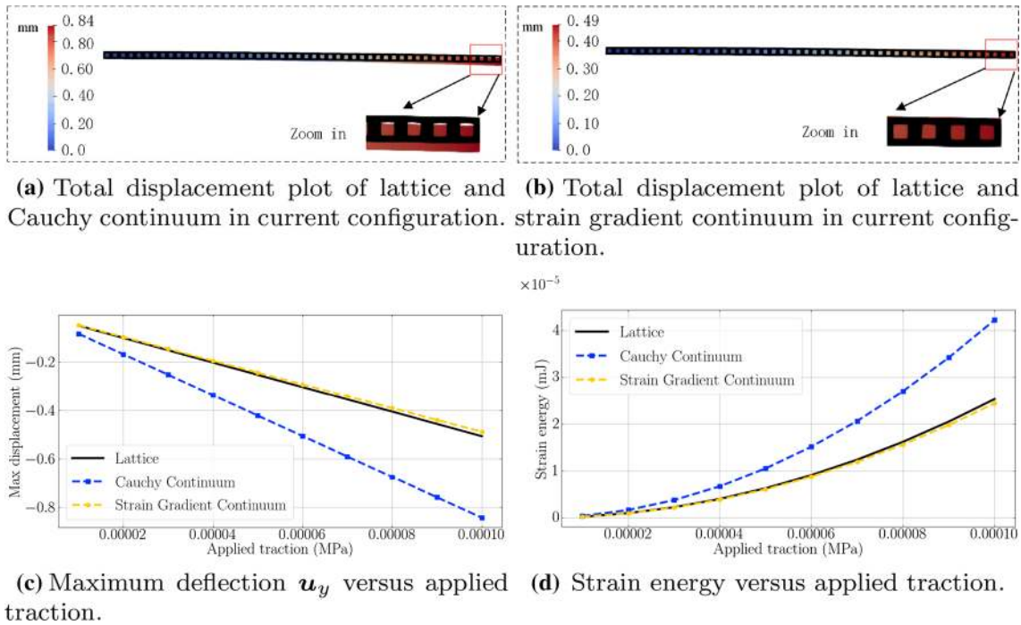
Fig. 10 Comparisons of lattice, Cauchy continuum, and strain gradient continuum for RVE with volume ratio 75%
