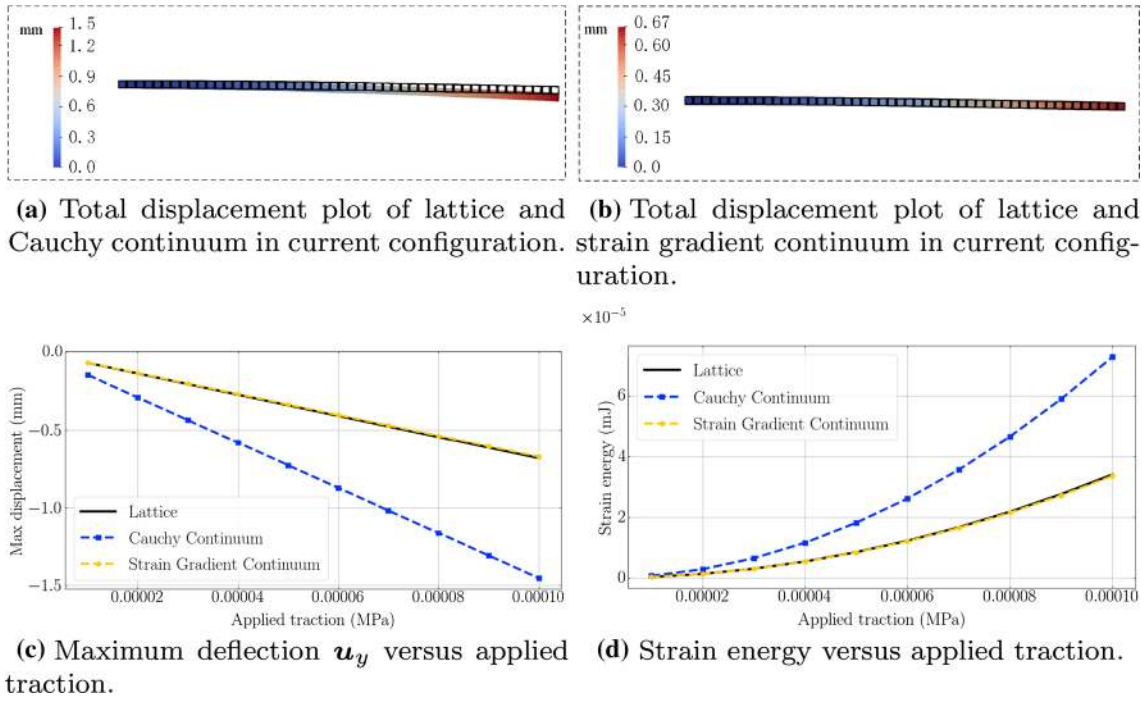
Fig. 9 Comparisons of lattice, Cauchy continuum, and strain gradient continuum for RVE with volume ratio 51%
