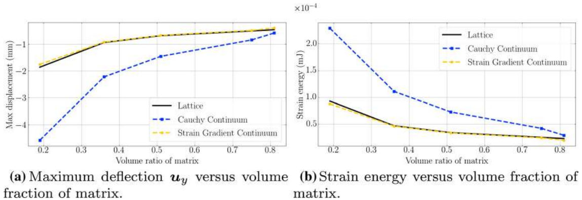
Fig. 12 Comparisons of maximum deflection u_y and strain energy versus volume fraction of matrix
