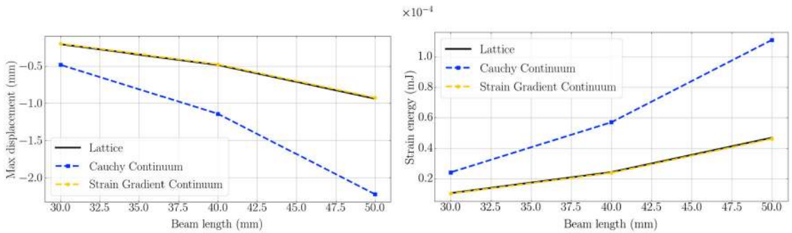
(a) Maximum deflection u_y versus macro length of the beam. (b) Strain energy versus macro length of the beam.
