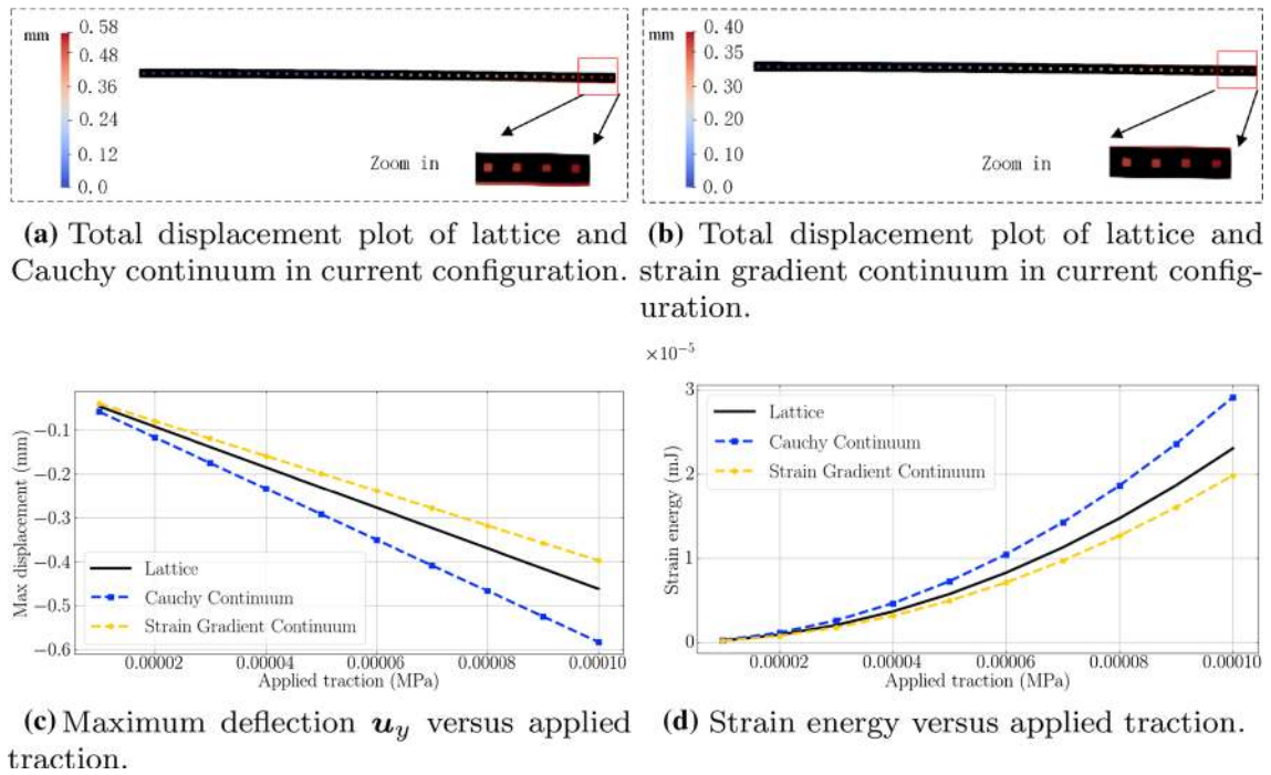
Fig. 11 Comparisons of lattice, Cauchy continuum, and strain gradient continuum for RVE with volume ratio 91%
