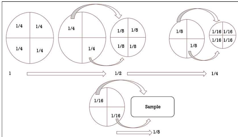
Figure 9. Coning and quartering procedure of 800 kg sample
