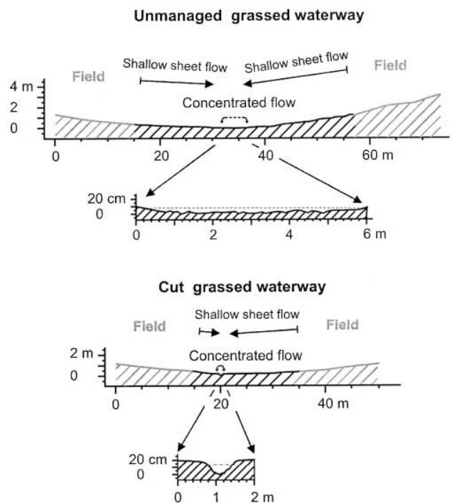
Fig. 2. Representative cross-sections of both grassed waterways; y axes twice inflated; dashed line represents water depth where concentrated flow occurs for a runoff rate of 6 L s -1 in both grassed waterways.
