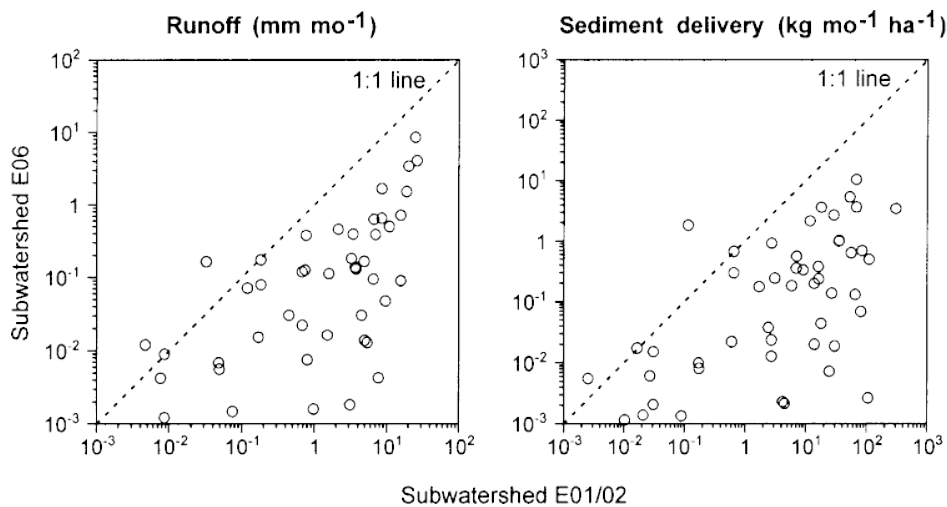
Fig. 5. Comparison of monthly runoff and sediment delivery of the upper subwatersheds between 1994 and 2000 (E06 with an unmanaged grassed waterway, E01/02 without).
