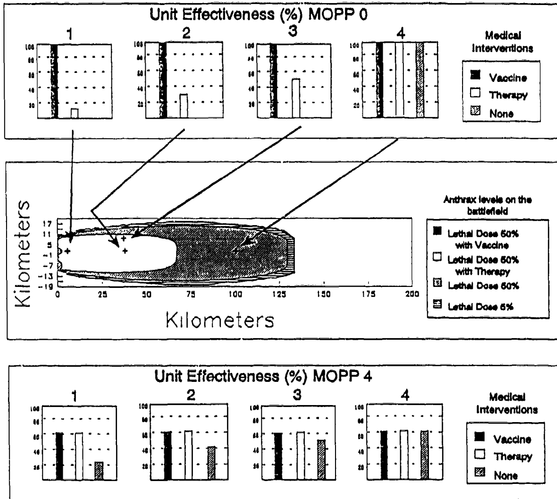
Figure C.16 TBM with Submunitions in Central Europe at 0500 Hours: Artillery Unit 100 Times Normal Toxicity Level, No Decay First Two Hours
