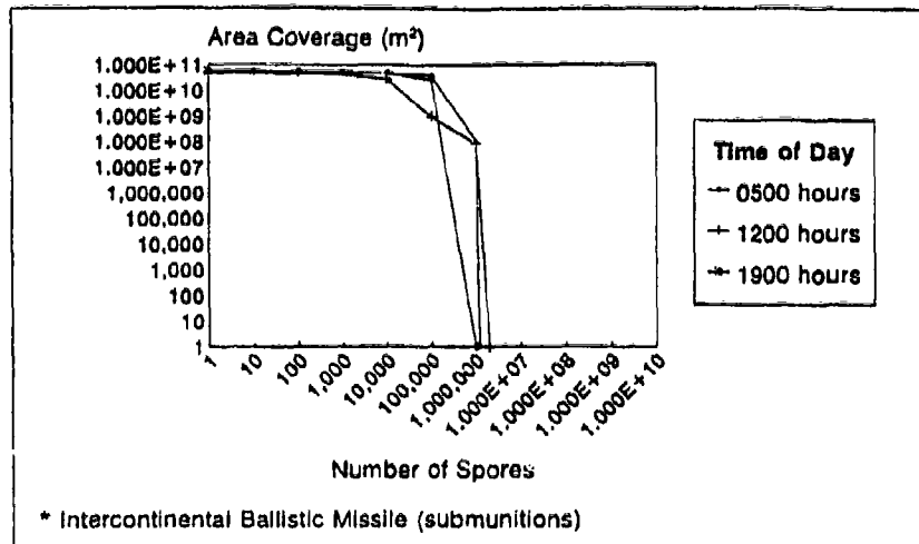
Figure 128. ICBM in Southeast Asia: Spore Area Coverage
