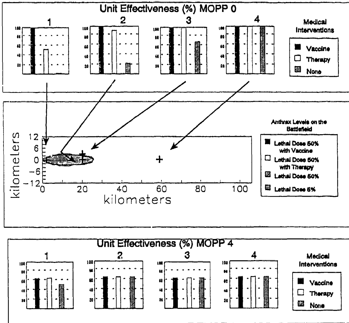
Figure 88. MRL in Central Europe at 1200 Hours: Artillery Unit Effectiveness with Medical Interventions
