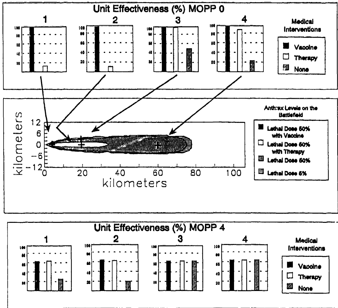
Figure 81. MRL in Southwest Asia at 0500 Hours: Artillery Unit Effectiveness with Medical Interventions
