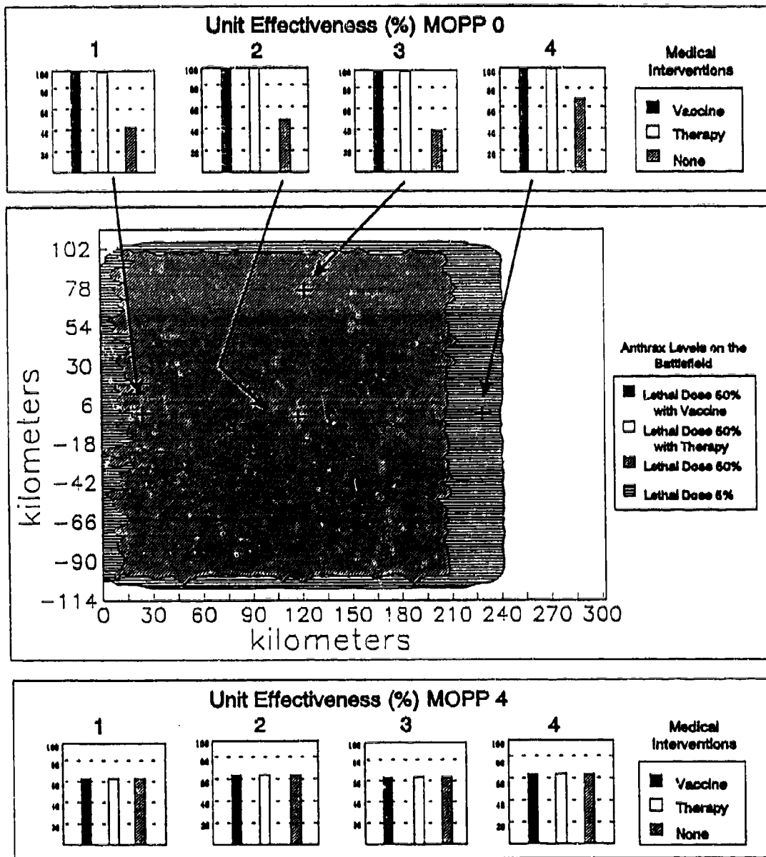
Figure 119. ICBM in Southeast Asia at 1200 Hours: Artillery Unit Effectiveness with Medical Interventions
