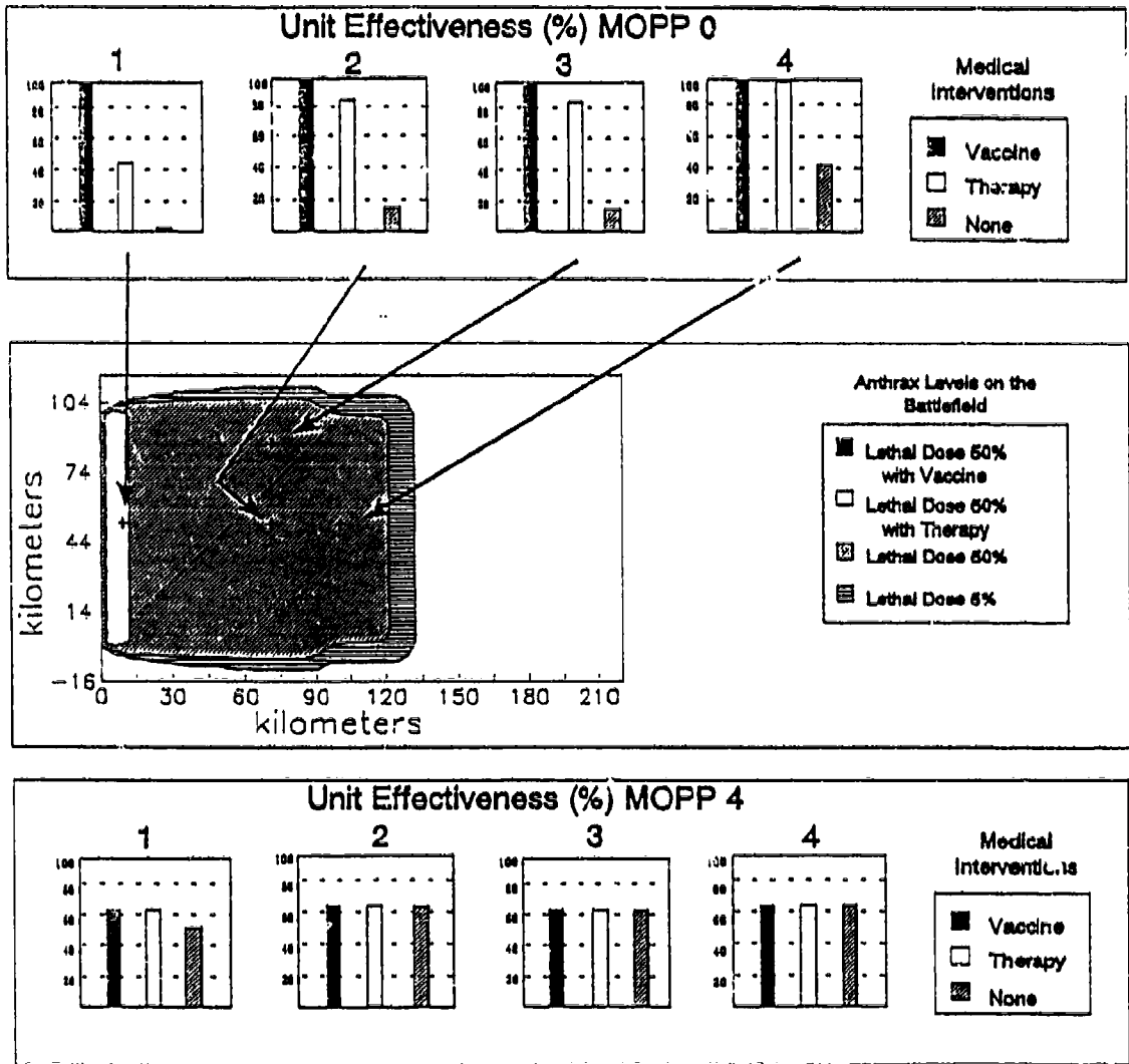
Figure 108. Aerial Spray in South Korea at 1200 Hours: Artillery Unit Effectiveness with Medical Interventions
