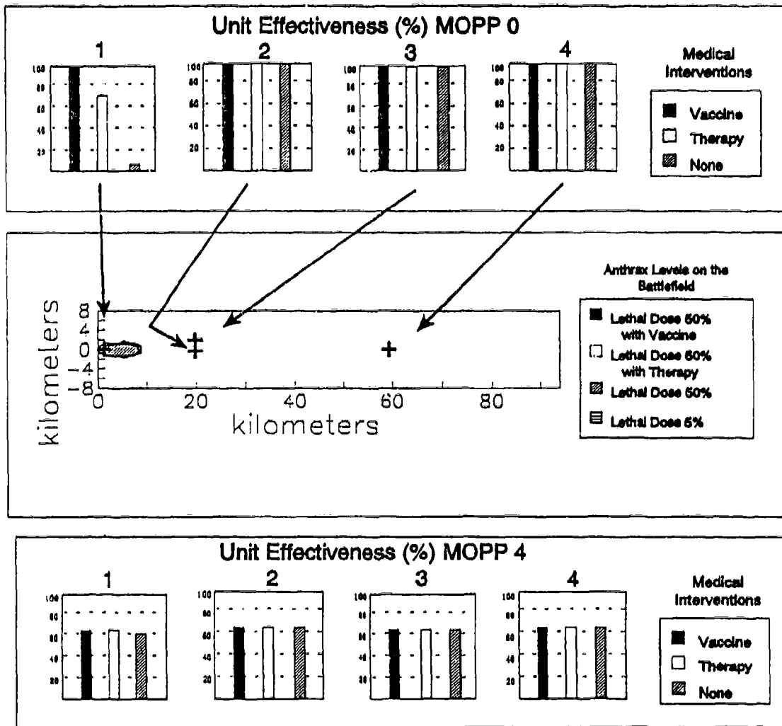
Figure 71. Artillery in Central Europe at 1200 Hours: Artillery Unit Effectiveness with Medical Interventions
