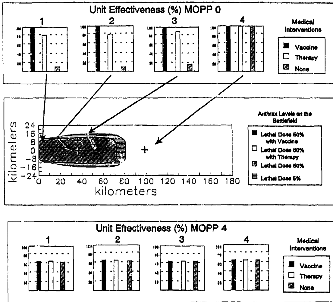
Figure 4. TBM with Submunitions in Central Europe at 1900 Hours: Artillery Unit Effectiveness with Medical Interventions (LD 50 = 3,689 spores)
