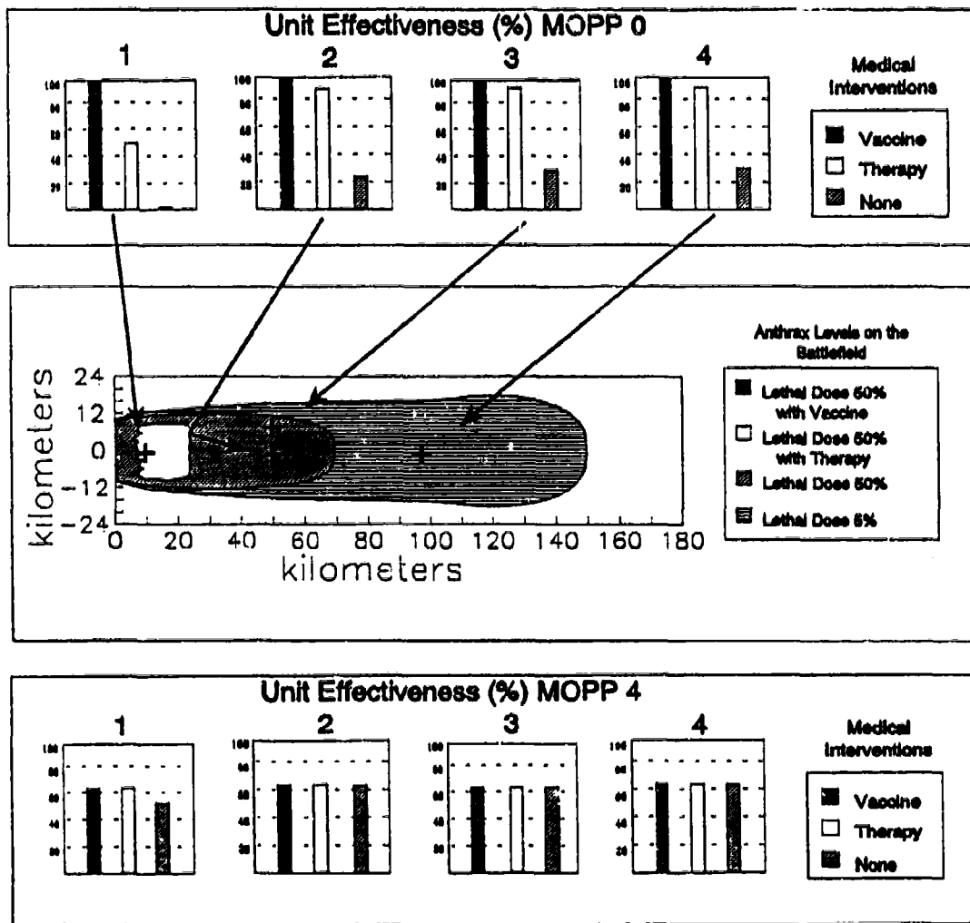
Figure 39. TBM with Submunitions in South Korea at 0500 Hours: Artillery Unit Effectiveness with Medical Interventions
