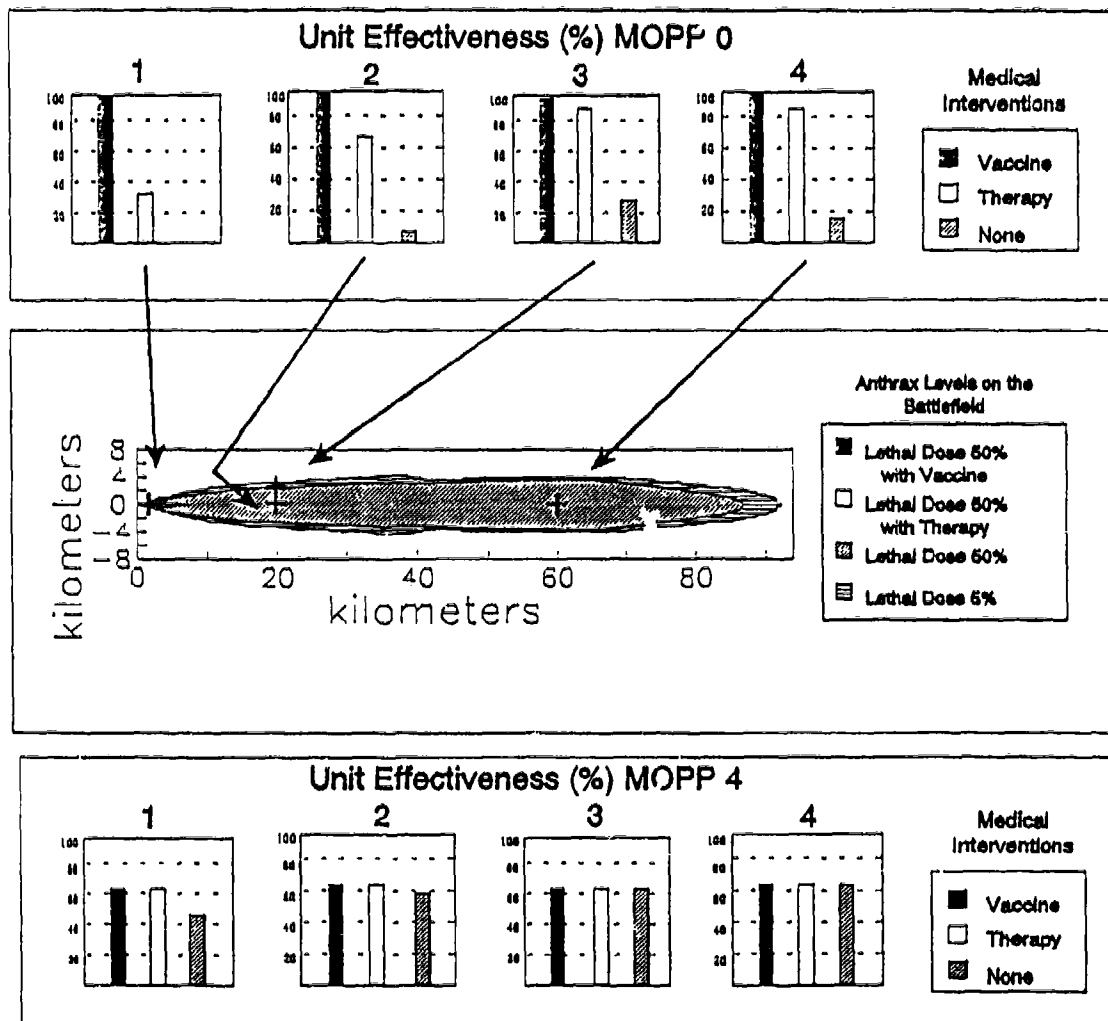
Figure 70. Artillery in Central Europe at 0500 Hours: Artillery Unit Effectiveness with Medical Interventions
