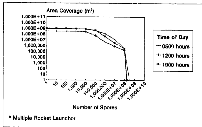
Figure 94. MRL in Southeast Asia: Spore Area Coverage
