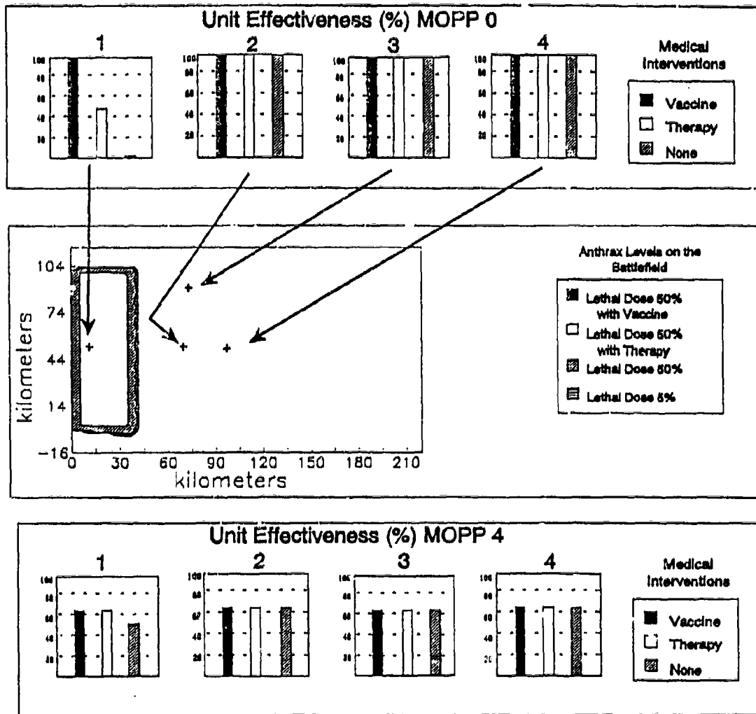
Figure 109. Aerial Spray in South Korea at 1900 Hours: Artillery Unit Effectiveness with Medical Interventions
