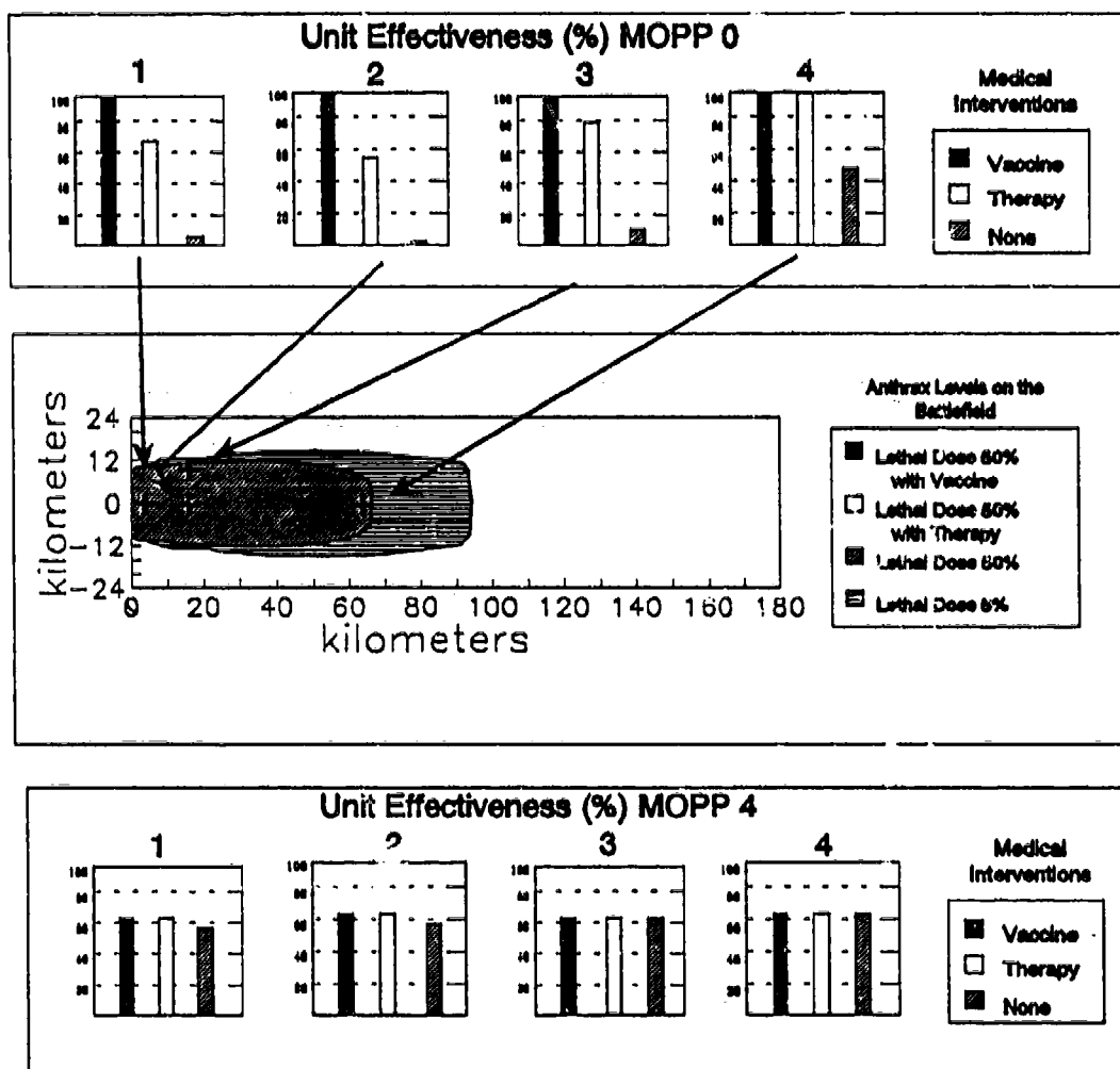
Figure 28. TBM with Submunitions in Southwest Asia at 0500 Hours: Artillery Unit Effectiveness with Medical Interventions
