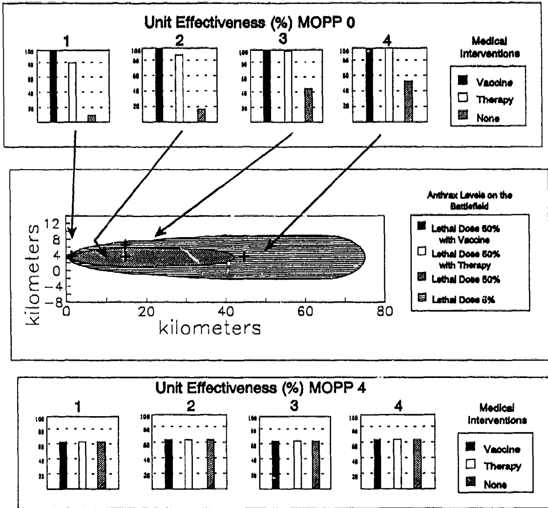
Figure 53. Terrorist Device in Central Europe at 0500 Hours: Artillery Unit Effectiveness with Medical Interventions
