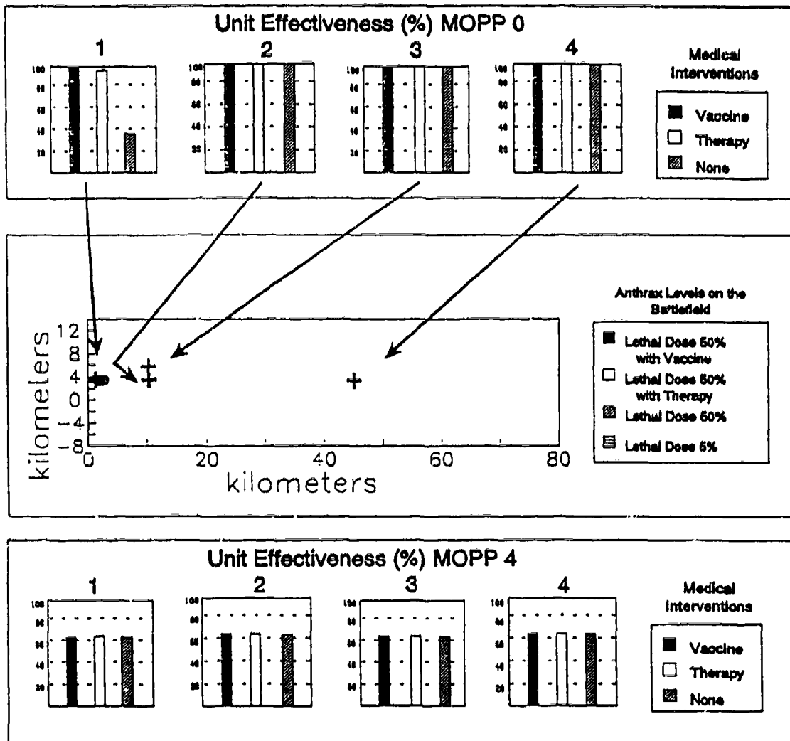
Figure 48. Terrorist Device in Southwest Asia at 1200 Hours: Artillery Unit Effectiveness with Medical Interventions
