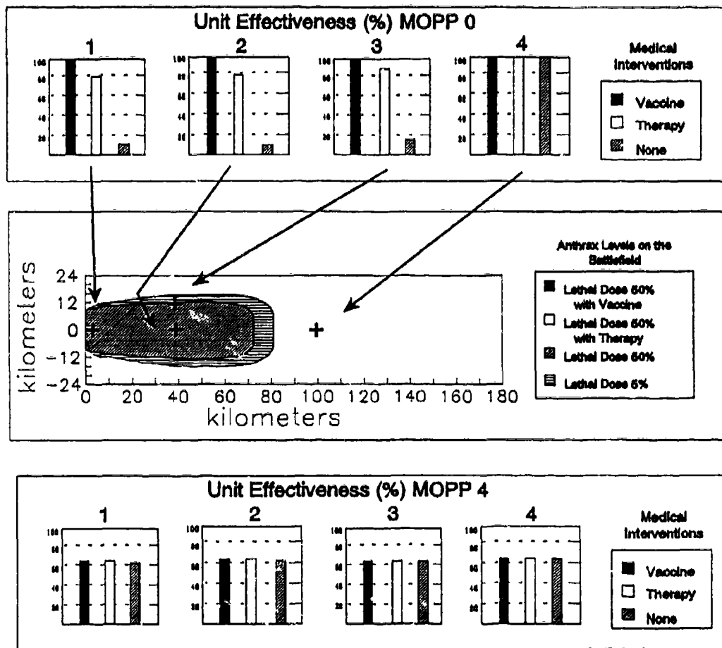
Figure 11. TBM with Submunitions in Central Europe at 1900 Hours: Artillery Unit Effectiveness with Medical Interventions (USAMRDC Decay Rates)
