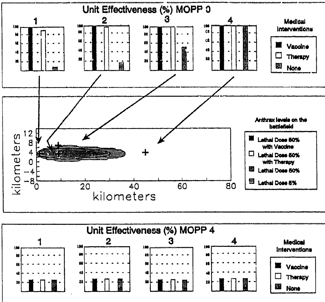
Figure 14. Terrorist Device in Southwest Asia at 0500 Hours: Ammunition Supply Point Unit Effectiveness with Medical Interventions
