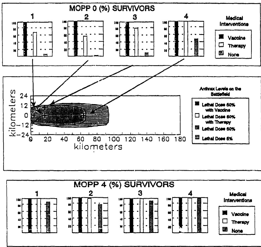
Figure 27. TBM with Submunitions in Southwest Asia at 0500 Hours: Artillery Unit % Survivors with Medical Interventions
