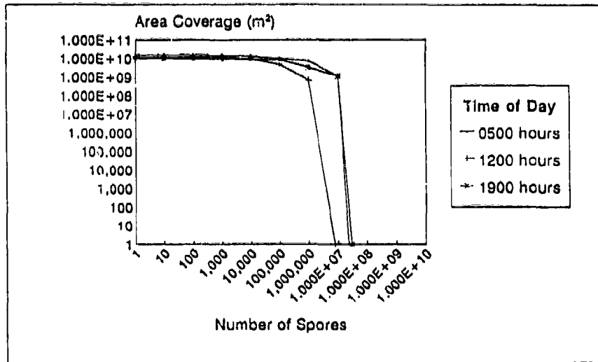
Figure 110. Aerial Spray in Southwest Asia: Spore Area Coverage
