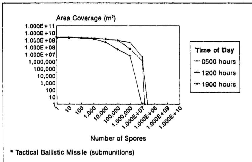
Figure 42. TBM in Southwest Asia: Spore Area Coverage
