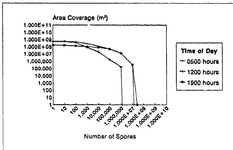
Figure 62. Terrorist Device in South Korea: Spore Area Coverage
