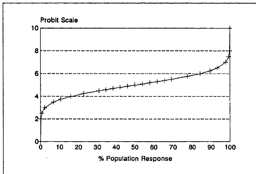
Figure 1. Probit Score vs. Population Response
