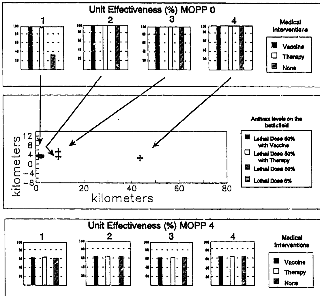
Figure 20. Terrorist Device in Southwest Asia at 1200 Hours: Infantry Anti-Armor Unit Effectiveness with Medical Interventions
