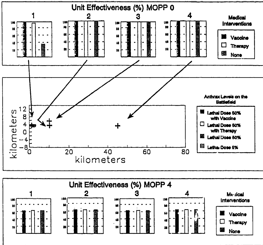
Figure 17. Terrorist Device in Southwest Asia at 1200 Hours: Artillery Unit Effectiveness with Medical Interventions
