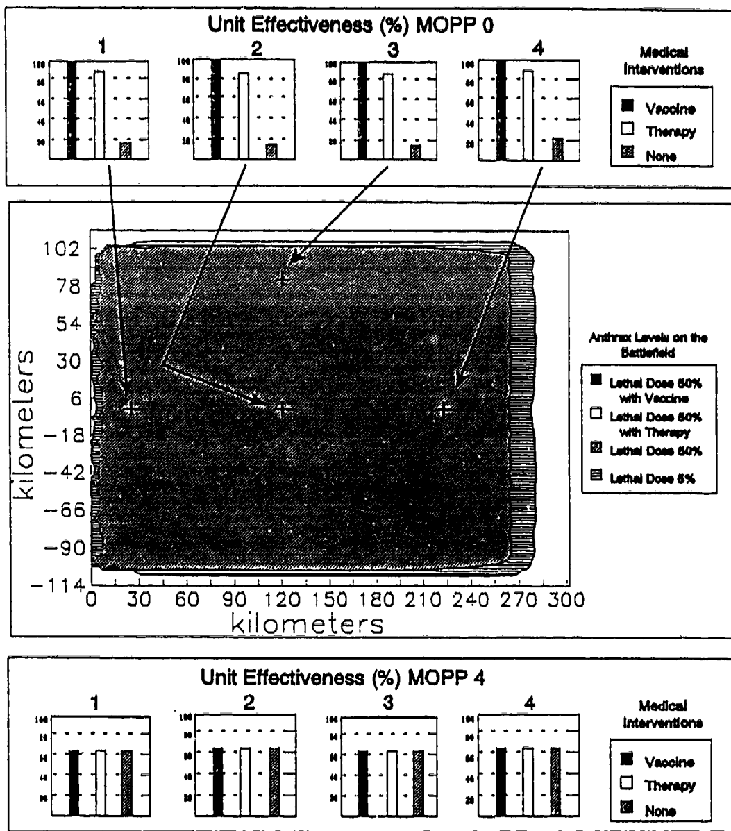
Figure 117. ICBM in Southwest Asia at 1900 Hours: Artillery Unit Effectiveness with Medical Interventions
