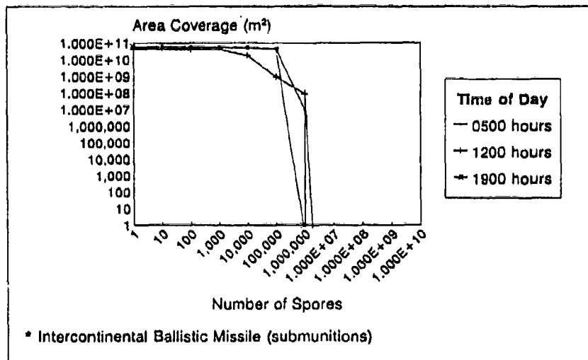
Figure 129. ICBM in Central Europe: Spore Area Coverage
