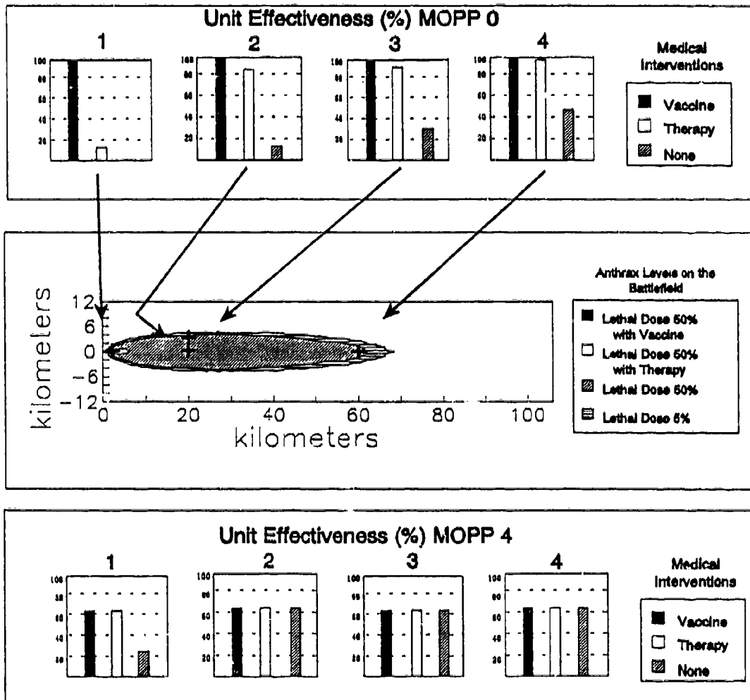
Figure 91. MRL in South Korea at 1200 Hours: Artillery Unit Effectiveness with Medical Interventions
