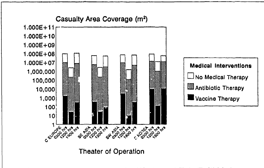
Figure 63. Terrorist Device: Casualty Area Coverage
