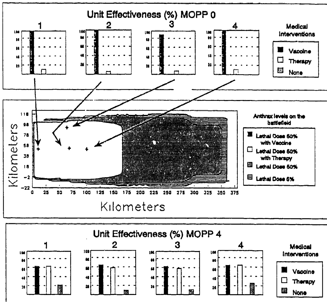
Figure C.22 Aerial Spray in Central Europe at 0500 Hours: Artillery Unit 100 Times Normal Toxicity Level, No Decay First Two Hours
