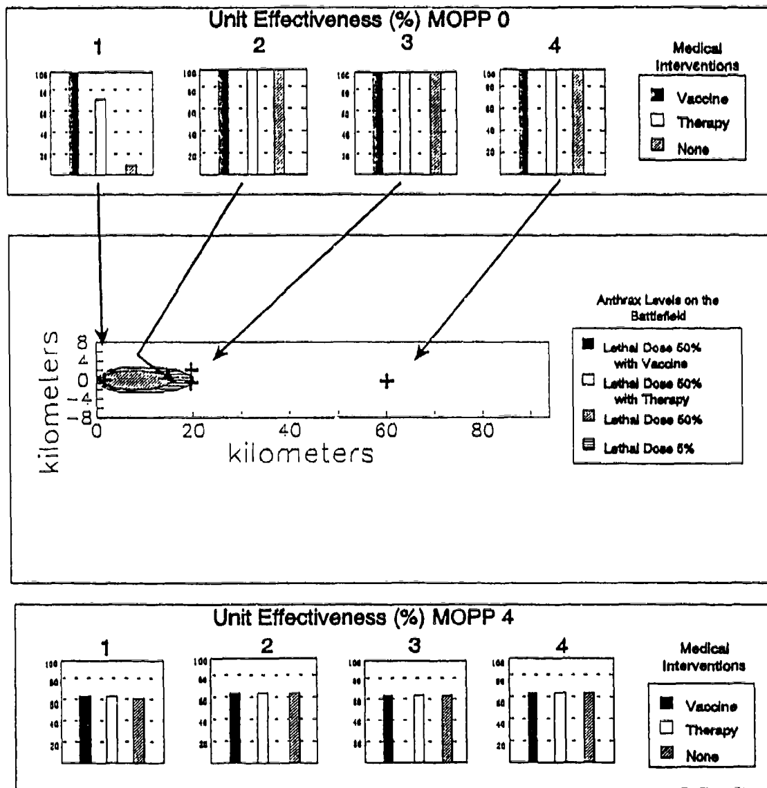
Figure 68. Artillery in Southeast Asia at 1200 Hours: Artillery Unit Effectiveness with Medical Interventions
