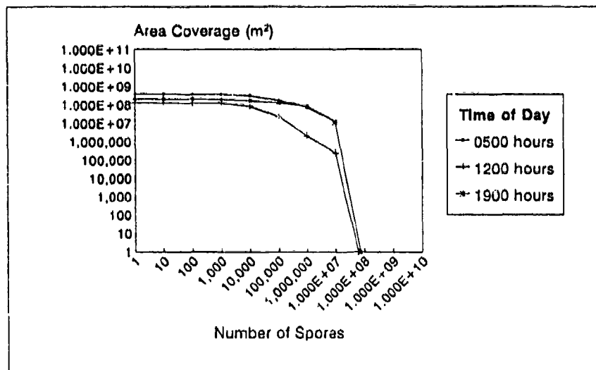
Figure 79. Artillery in South Korea: Spore Area Coverage
