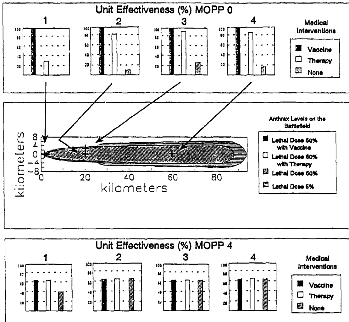
Figure 72. Artillery in Central Europe at 1900 Hours: Artillery Unit Effectiveness with Medical Interventions
