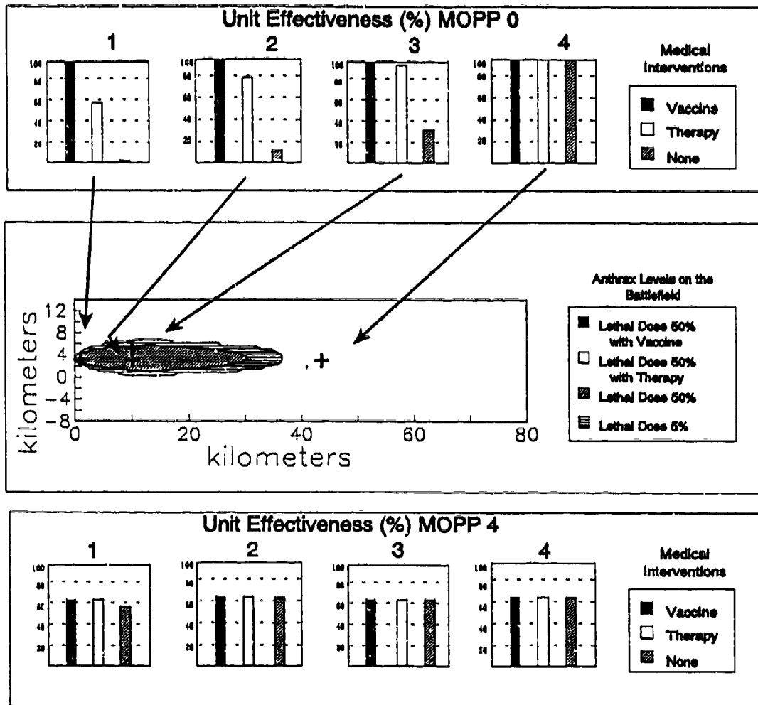
Figure 47. Terrorist Device in Southwest Asia at 0500 Hours: Artillery Unit Effectiveness with Medical Interventions
