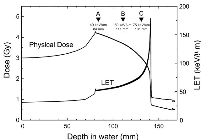
Fig. 1. SOBP and the different positions for cell irradiation.
