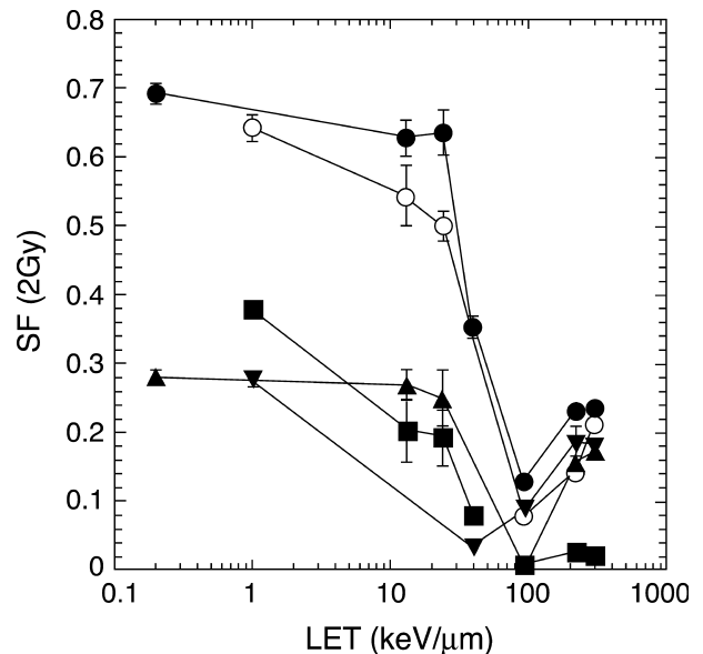
Fig. 3. SF(2 Gy) versus LET for all cell lines and monoenergetic carbon-ions. (●)SQ20B; (■)M10; (▲)SCC25; (▼)HF19; (○)V79.
