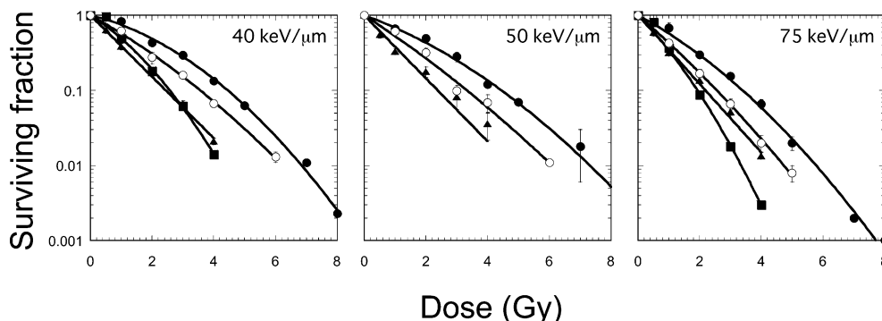
Fig. 4. Cell inactivation by 290 MeV/SOBP carbon-ions. (●)SQ20B; (■)M10; (▲)SCC25; (○)V79.
