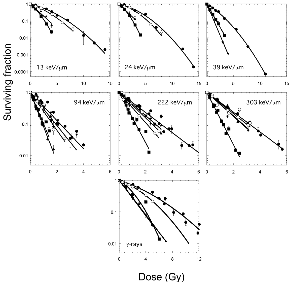
Fig. 2. Cell inactivation by \gamma -rays and monoenergetic carbon-ions at different LET values. (●)SQ20B; (■)M10; (▲)SCC25; (▼)HF19; (○) V79.
