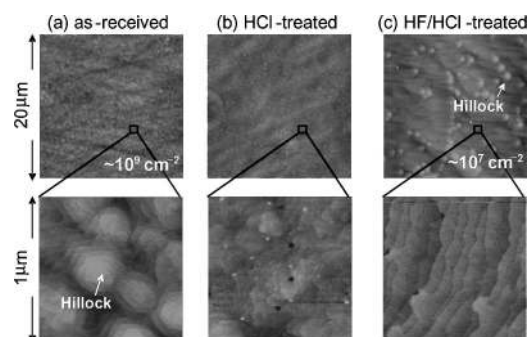
FIG. 4. AFM images of GaN layers grown on 6H-SiC substrates with three different pretreatments: (a) the as-received substrate, (b) the HCl-treated substrate and (c) the HCl/HF-treated substrate. Spiral growth hillocks are observed in (a) and (c), whereas no clear structure is observed in (b). The density of the hillocks in (c) is two orders of magnitude smaller than that in (a).
