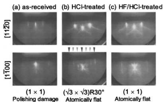
FIG. 1. RHEED patterns of 6H-SiC substrates after thermal cleaning. (a) As-received substrate, (b) HCl-treated substrate and (c) HF/HCl-treated substrate. Intense streaky patterns with Kikuchi lines are observed in (b) and (c), indicating an atomically flat surface. No reconstruction is observed in (a) and (c), whereas (\sqrt{3} \times \sqrt{3})R30^\circ reconstruction is observed in (b).
