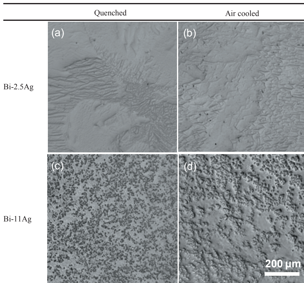
Fig. 3 Microstructure of Bi-Ag solder alloys of (a) quenched Bi-2.5Ag, (b) air-cooled Bi-2.5Ag, (c) quenched Bi-11Ag, (d) air-cooled Bi-11Ag.
