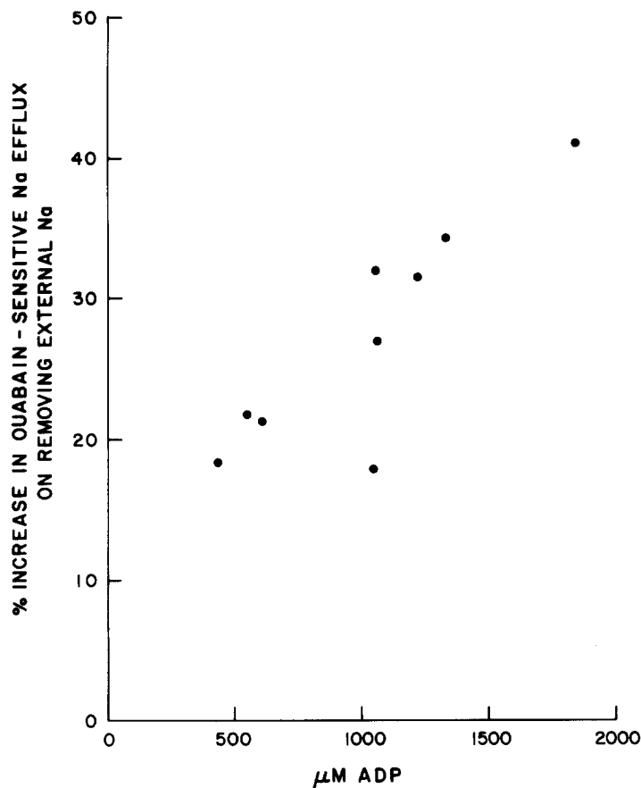
FIGURE 6. The percent stimulation of ouabain-sensitive Na efflux caused by removal of external Na, as internal ADP is increased. The ouabain-sensitive efflux rate constant for Na, {}^{\circ}k_{\text{Na}} , was determined at 37°C in the presence and absence of external Na, as described in Materials and Methods. The Na-containing medium (A) contained 135 mM NaCl, 15 mM KCl, and 10 mM HEPES (pH 7.4). The Na-free medium (B) contained 135 mM choline Cl, 15 mM KCl, and 10 mM HEPES (pH 7.4). Each point represents the percent change in the ouabain-sensitive Na flux components calculated according to the equation:
