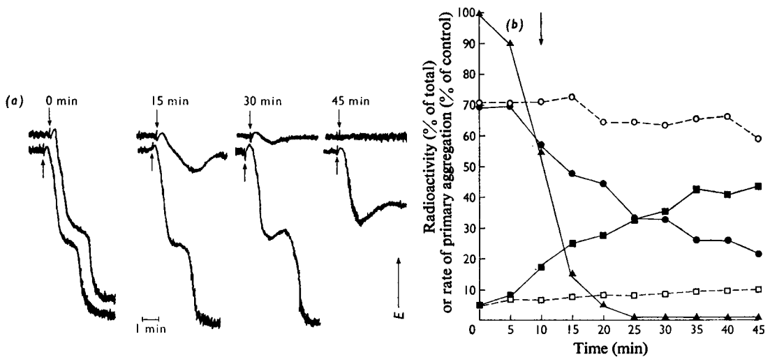
Fig. 5. Incubation of [^3\text{H}]\text{adenine} -labelled platelet-rich plasma at 37^\circ\text{C} with antimycin A and 2-deoxyglucose and concomitant determination of the rate of ADP-induced platelet aggregation
