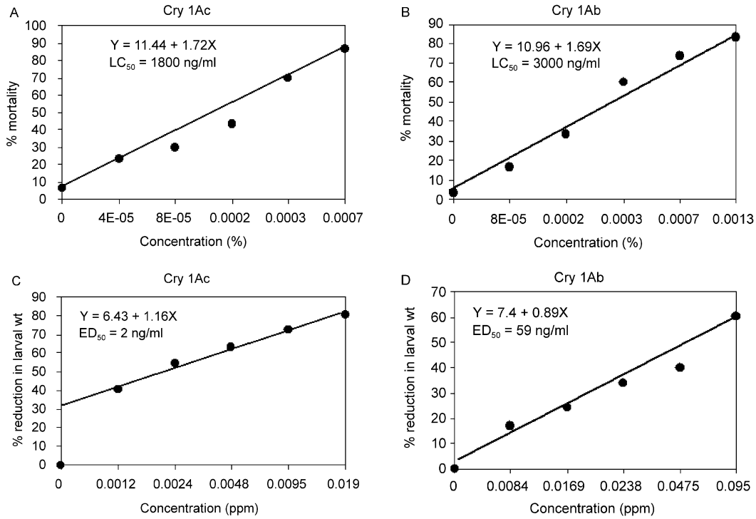
Figure 1 The LC 50 (effective concentration to kill 50% of the neonate Helicoverpa armigera larvae) [(A) Cry1Ac and (B) Cry1Ab] and ED 50 (effective concentration to cause a 50% reduction in larval weight) [(C) Cry1Ac and (D) Cry1Ab] of Bacillus thuringiensis δ-endotoxins against neonate H. armigera larvae.
