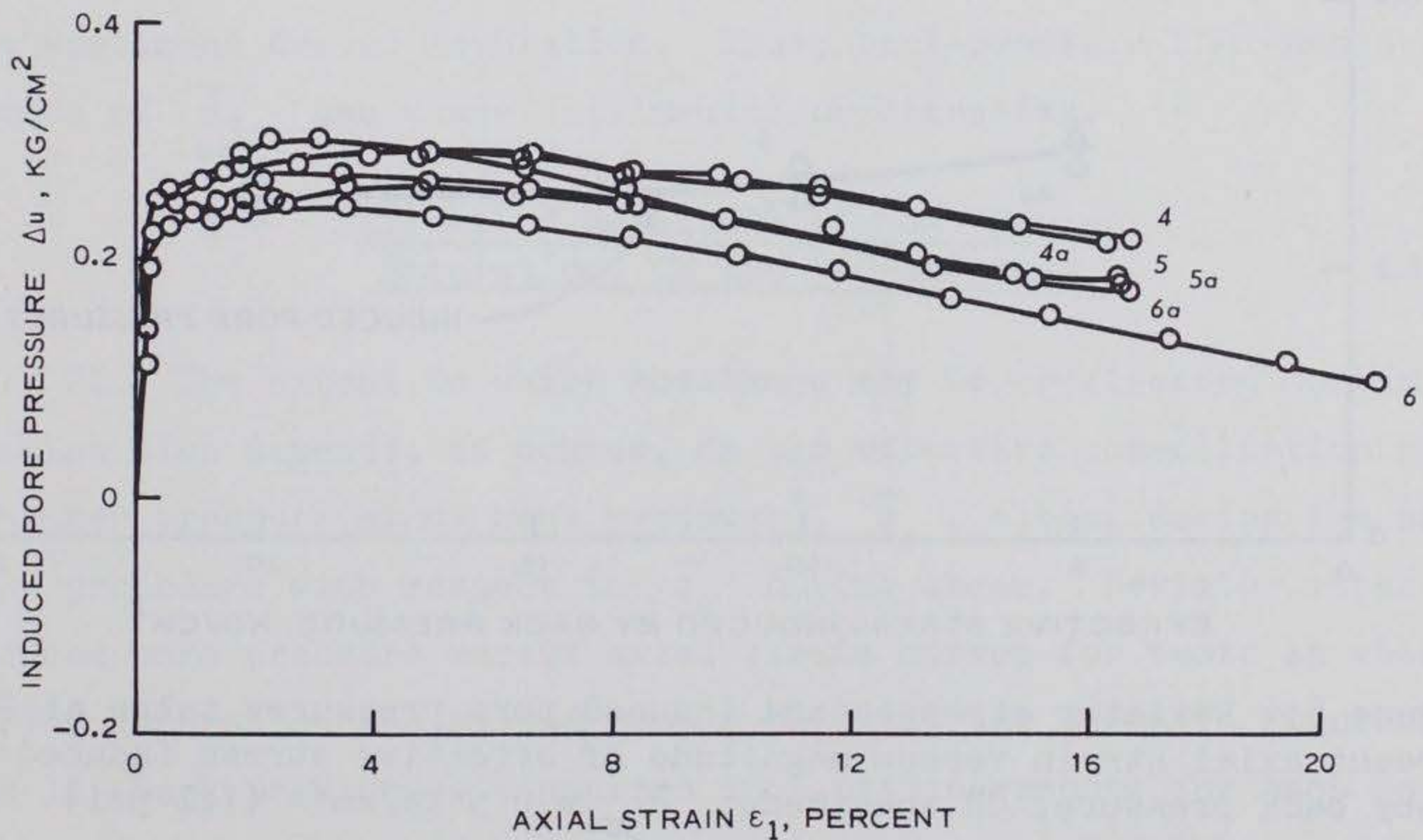
Figure 7. Deviator stress and induced pore pressure versus axial strain curves for tests in which the magnitude of effective stresses induced by back pressure was varied, CH specimens
