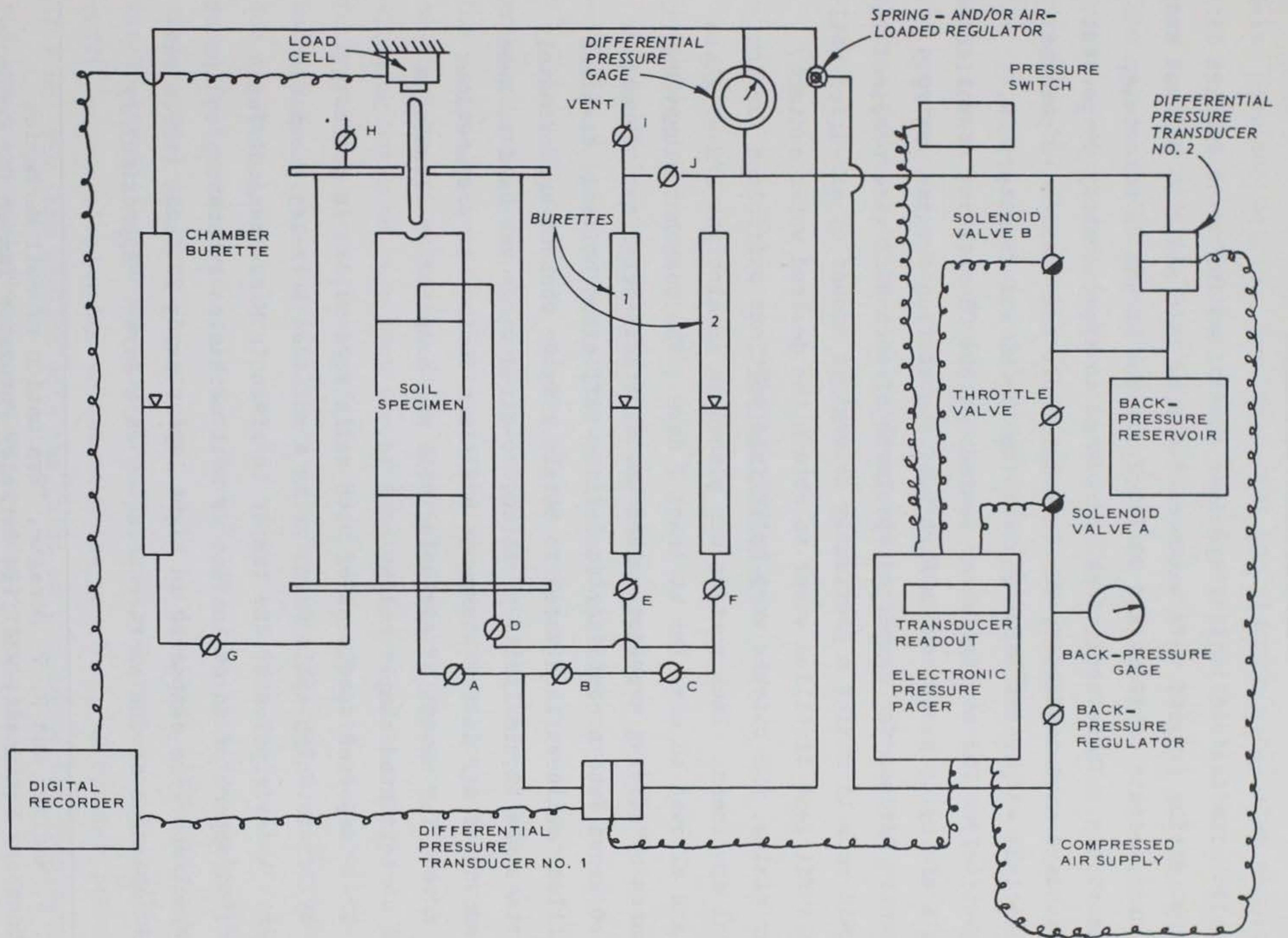
Figure 2. Schematic diagram of testing apparatus
