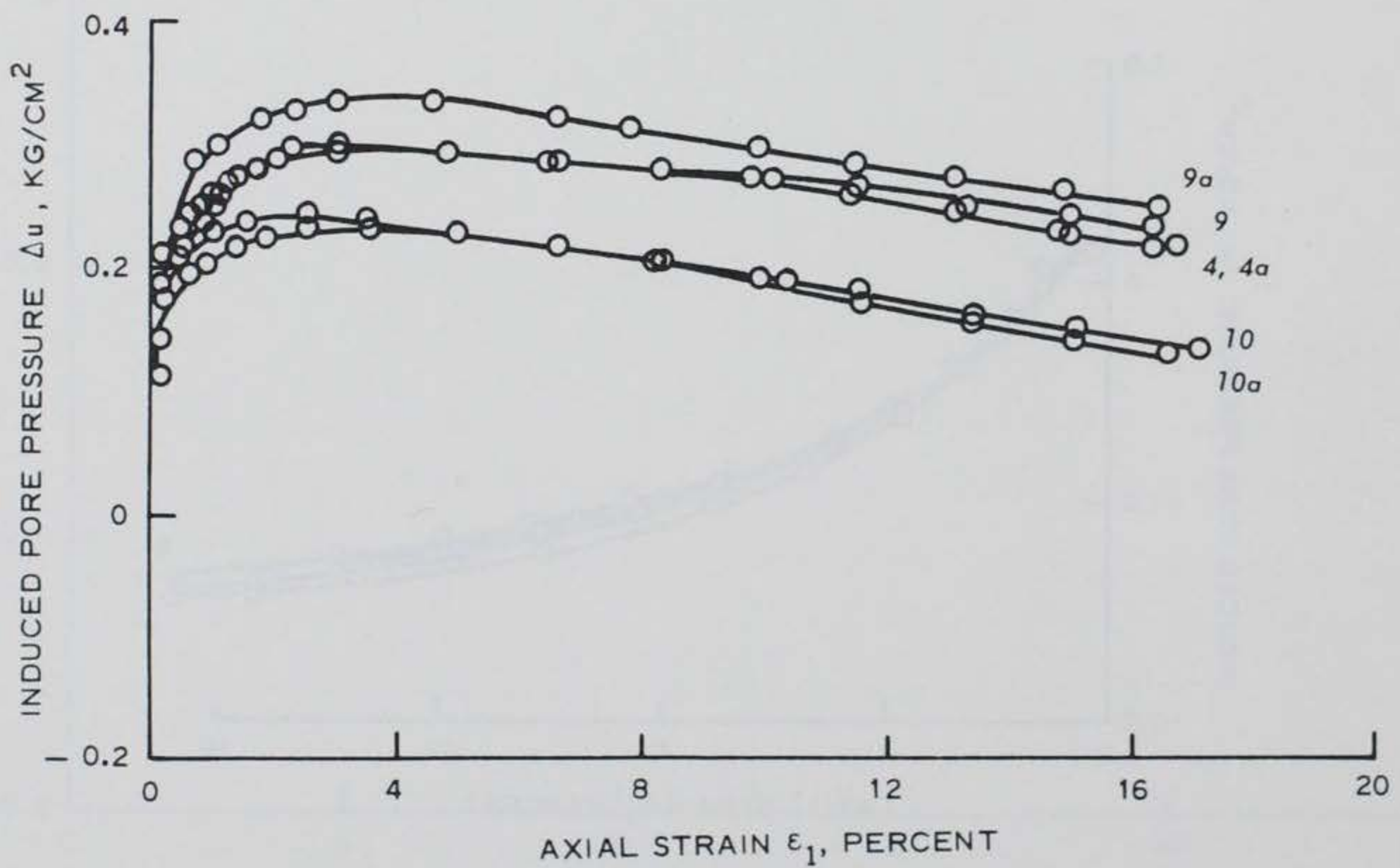
Figure 11. Deviator stress and induced pore pressure versus axial strain curves for tests in which the magnitude of the effective consolidation stress during saturation was varied, CH specimens
