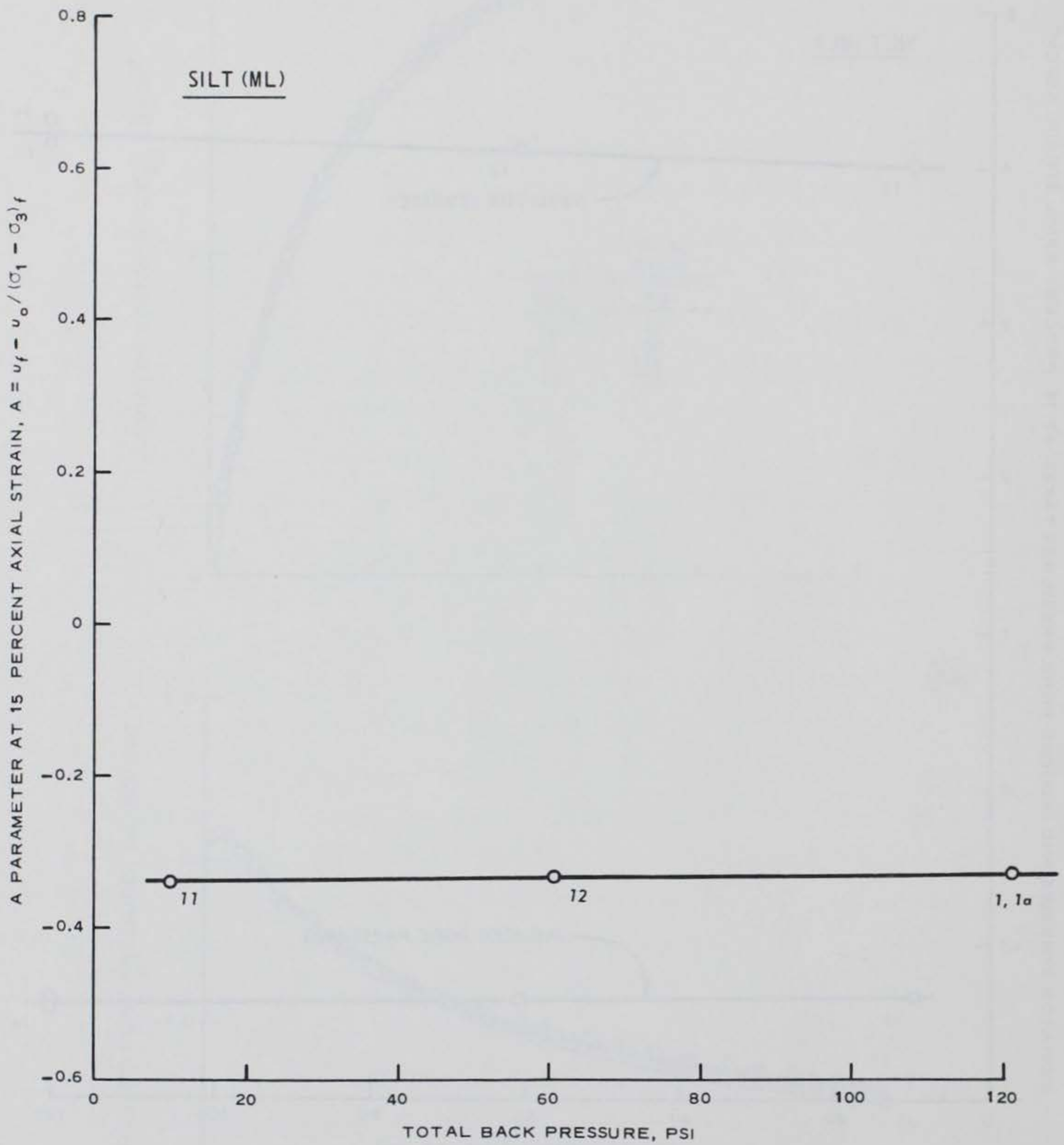
Figure 17. A parameter at 15 percent axial strain versus total back pressure, ML specimens, \bar{\sigma}_c = 0.5 \text{ kg/cm}^2 (7.1 psi)
