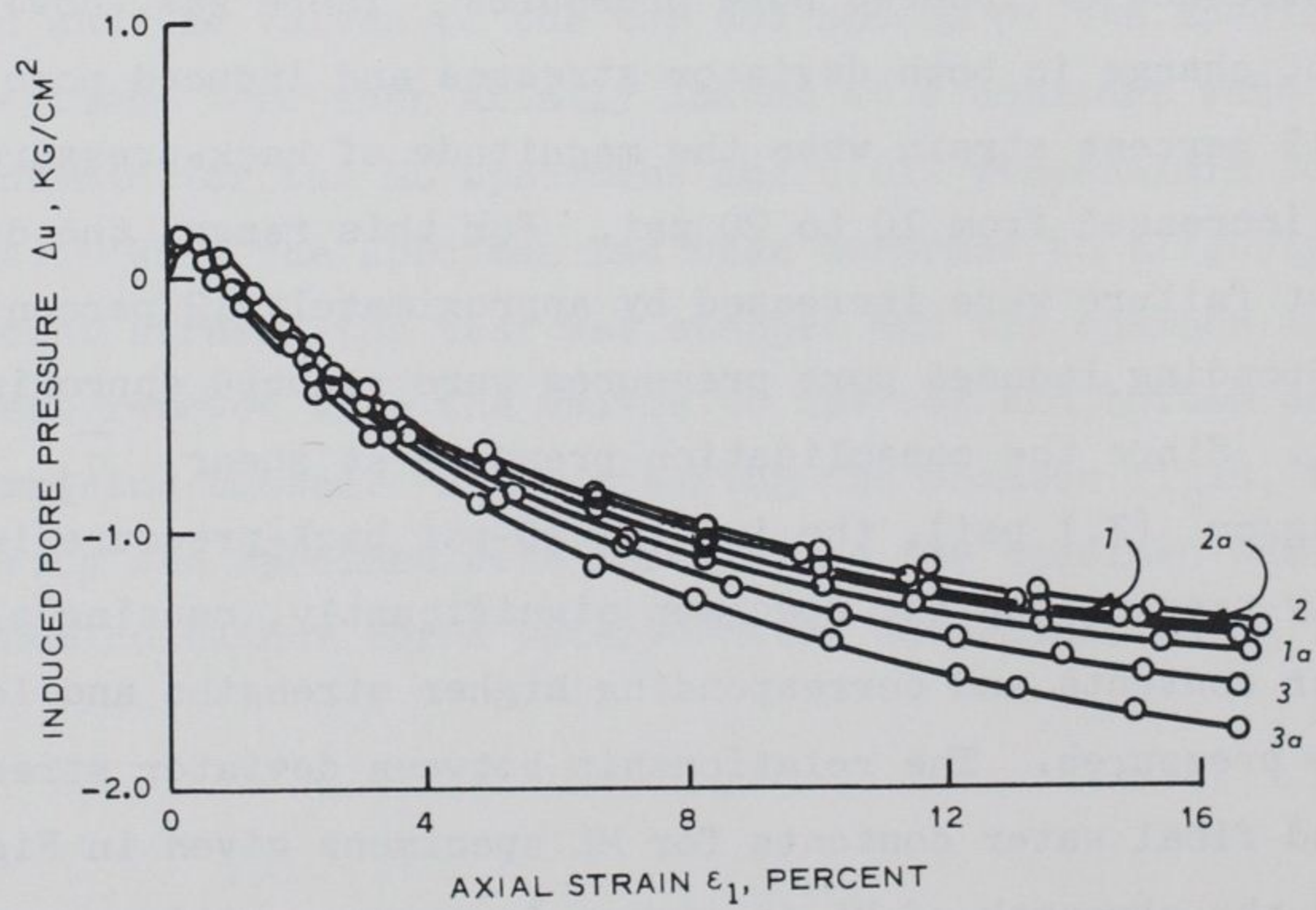
Figure 3. Deviator stress and induced pore pressure versus axial strain curves for tests in which the magnitude of back-pressure increments was varied, ML specimens
