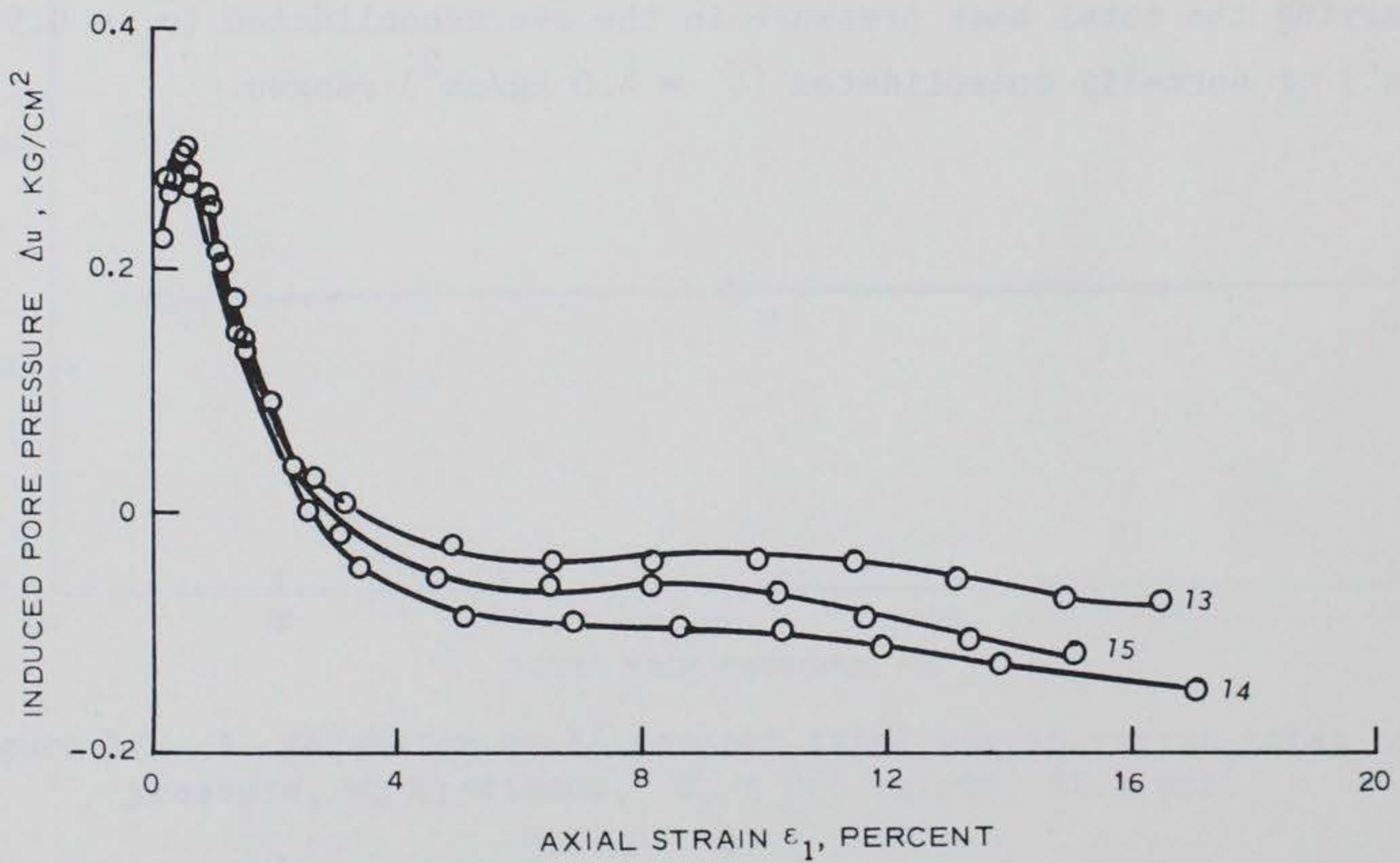
Figure 18. Deviator stress and induced pore pressure versus axial strain curves for tests 13, 14, and 15 in which the magnitude of the total back pressure was varied, CH specimens consolidated from a slurry
