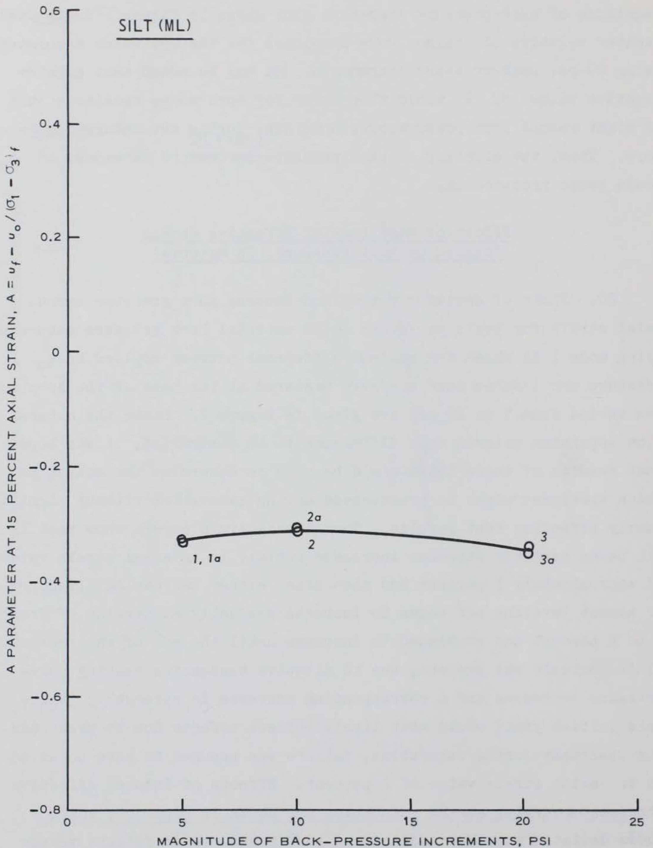
Figure 6. A parameter at 15 percent axial strain versus magnitude of back-pressure increments, ML specimens, \bar{\sigma}_{3c} = 0.5 \text{ kg/cm}^2 (7.1 psi)
