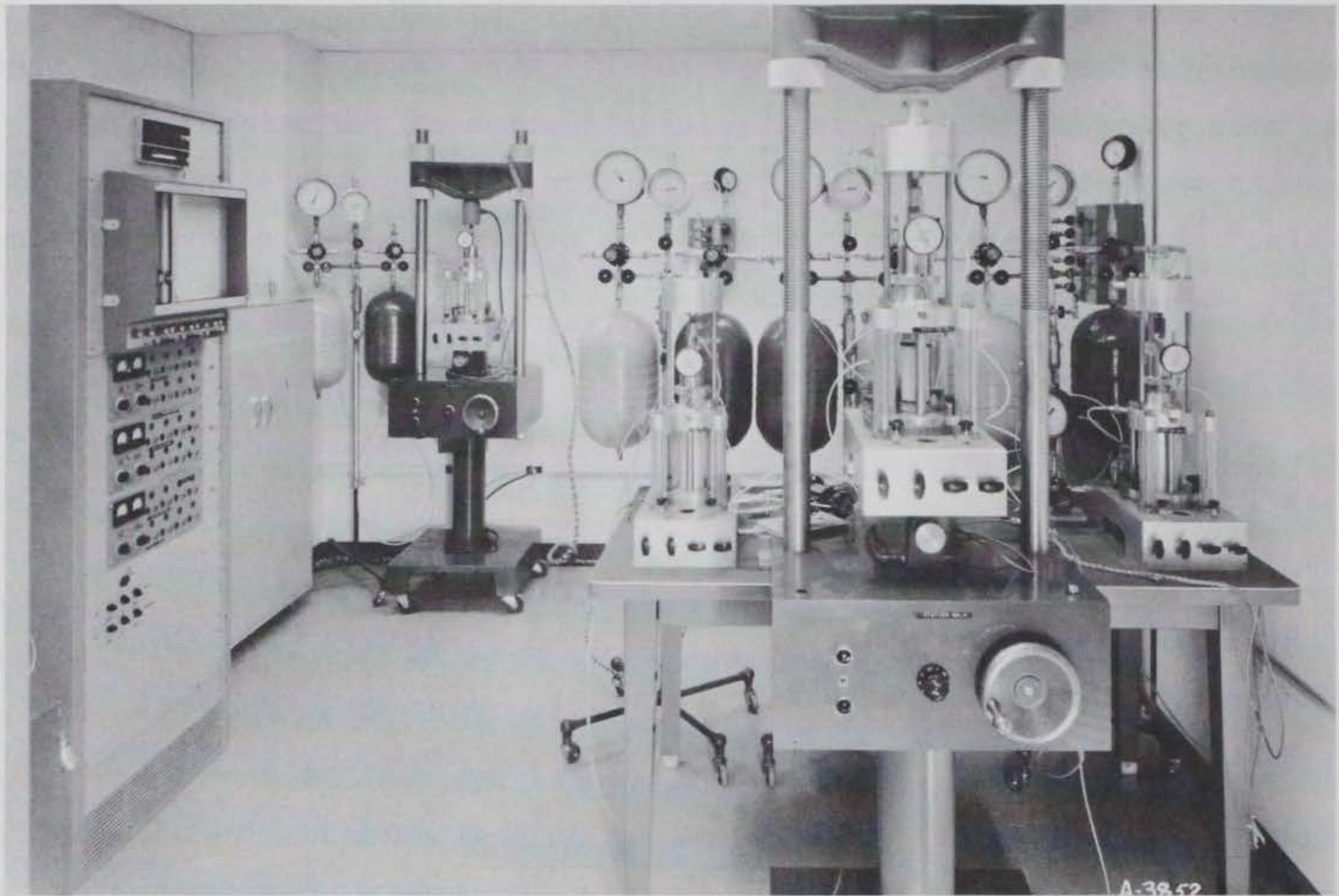
Figure 1. Triaxial testing facility
