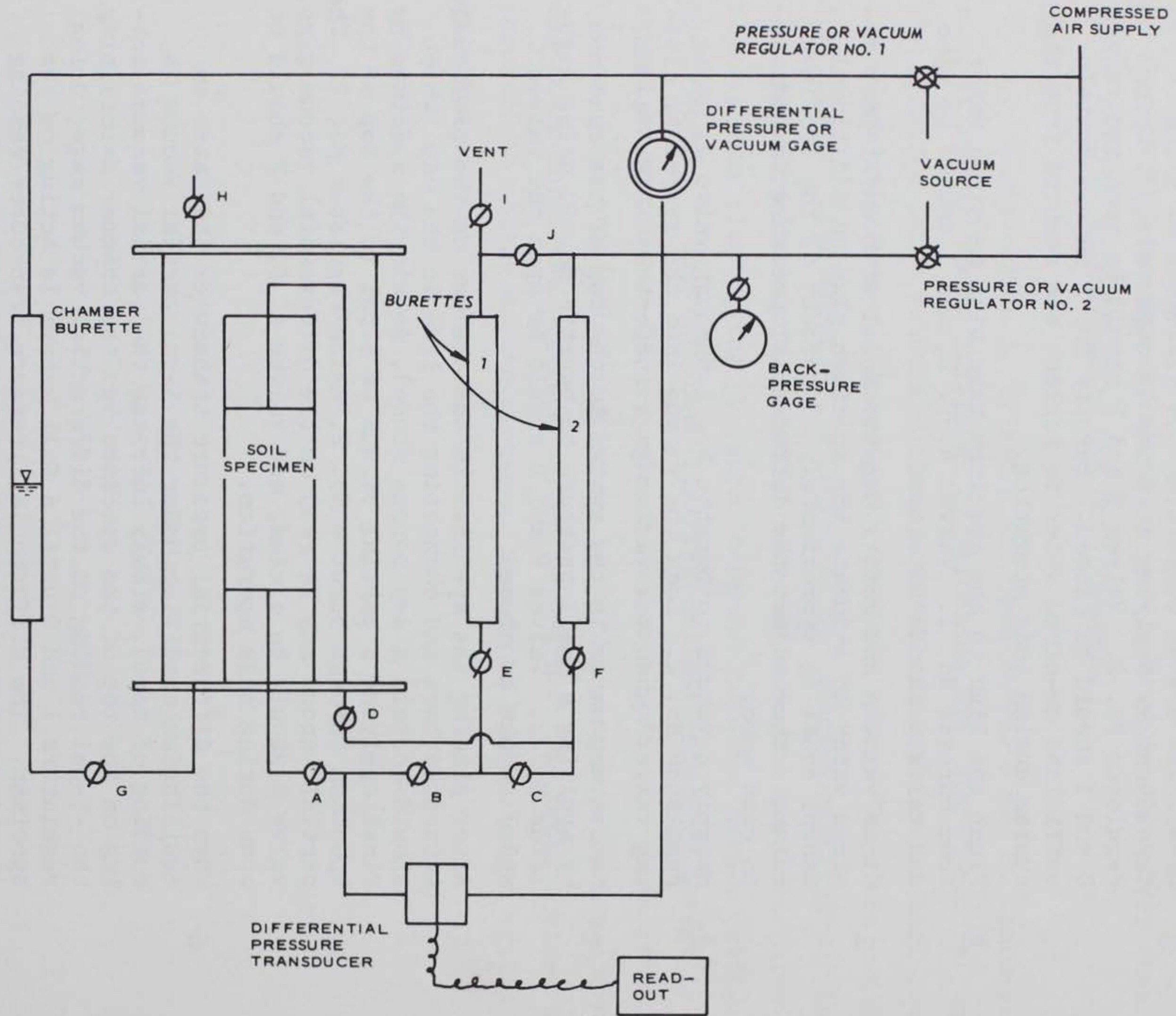
Figure C1. Schematic diagram of the differential vacuum saturation apparatus and pressure control system
