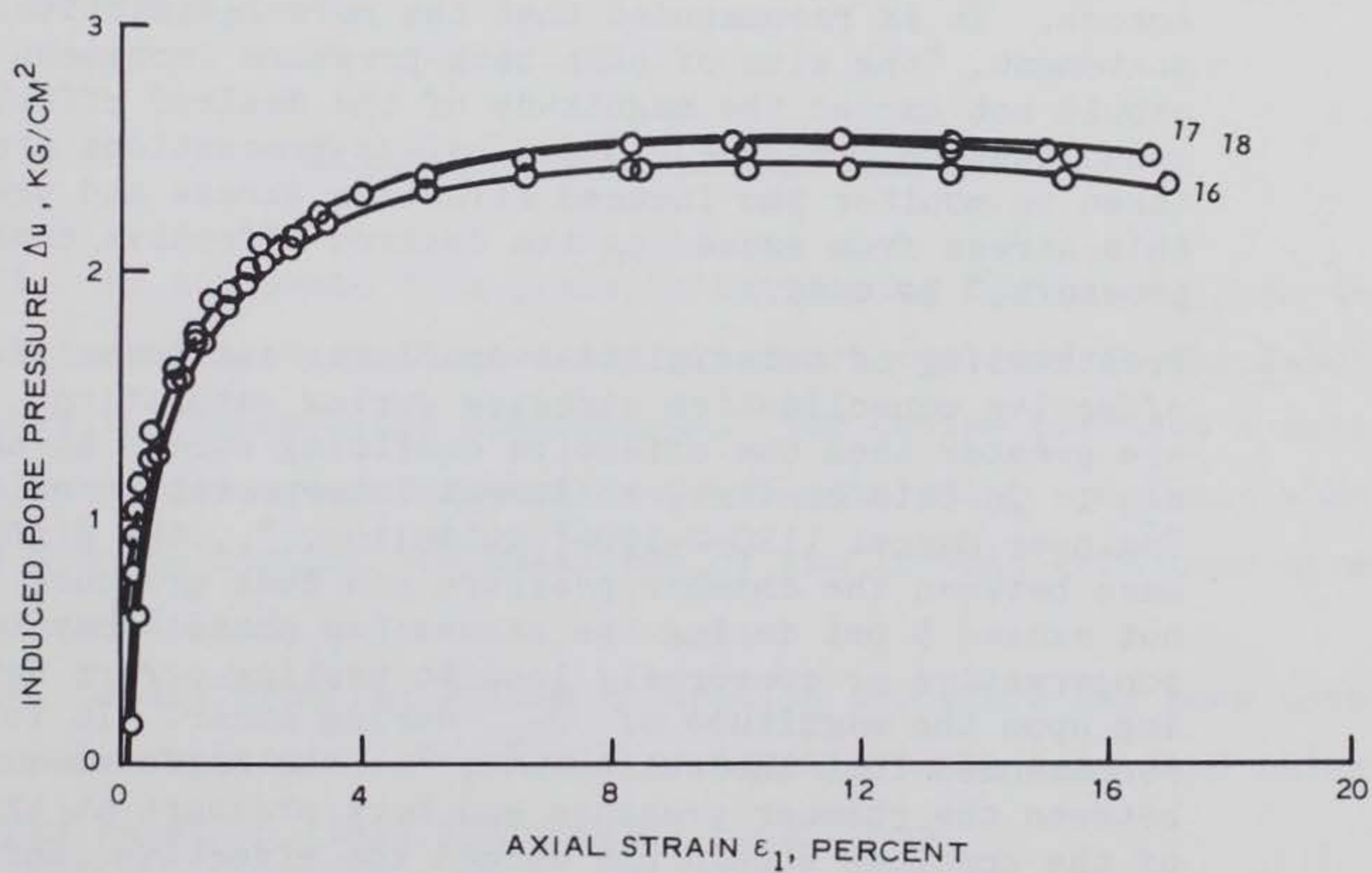
Figure 19. Deviator stress and induced pore pressure versus axial strain curves for tests 16, 17, and 18 in which the magnitude of the total back pressure was varied, CH specimens consolidated from a slurry
