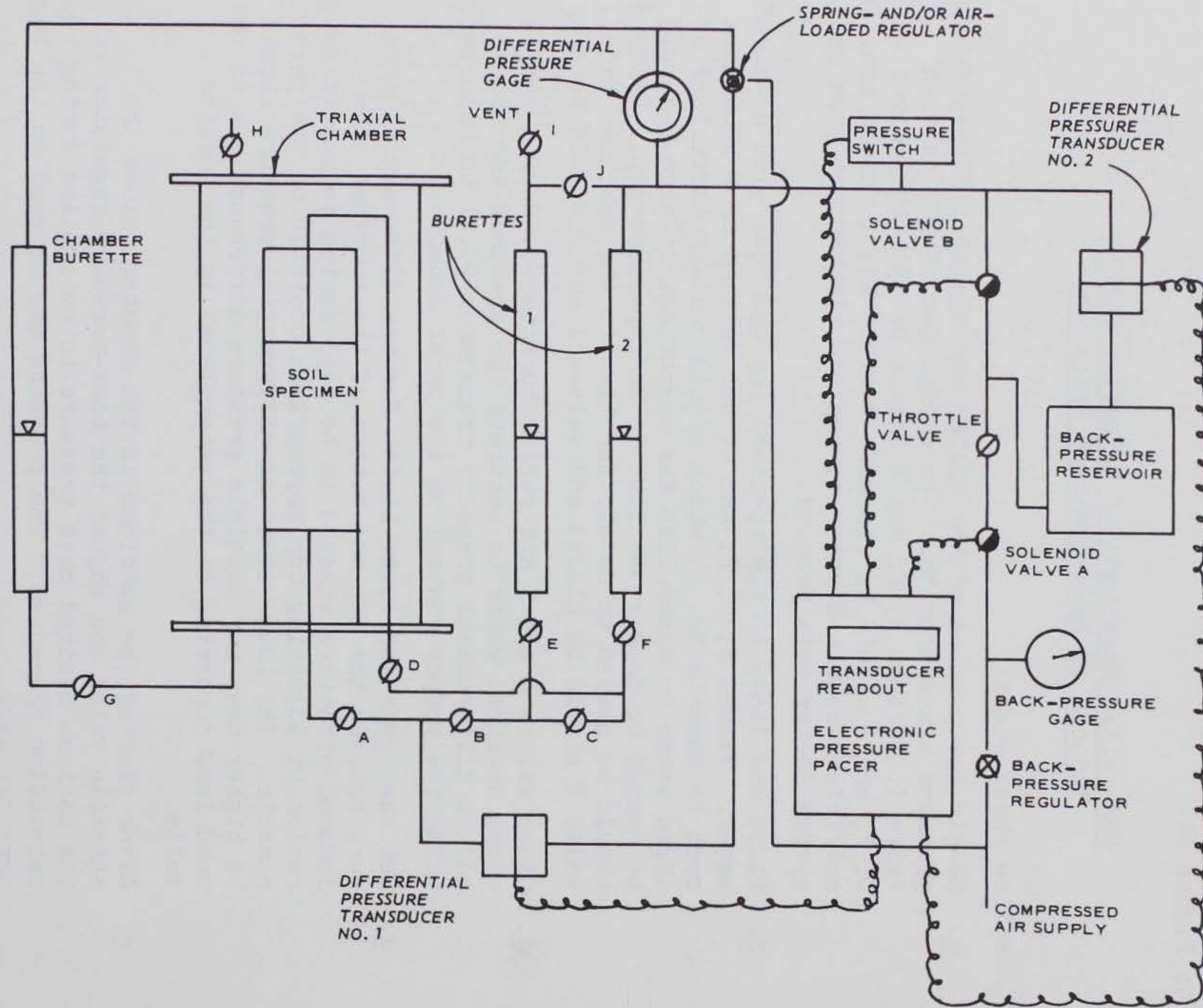
Figure B1. Schematic diagram of the back pressure saturation apparatus and pressure control
