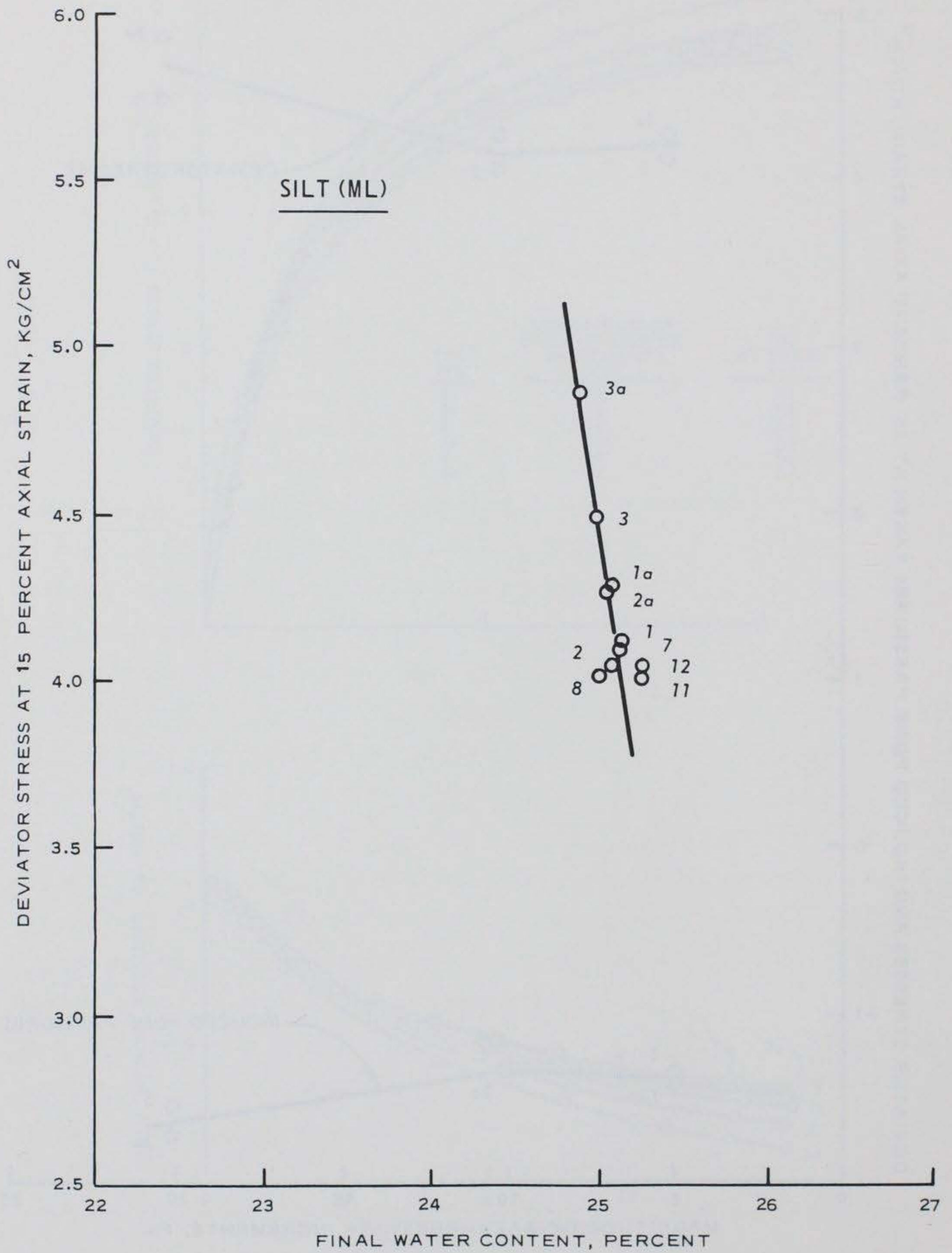
Figure 5. Deviator stress at 15 percent axial strain versus final water content, ML specimens
