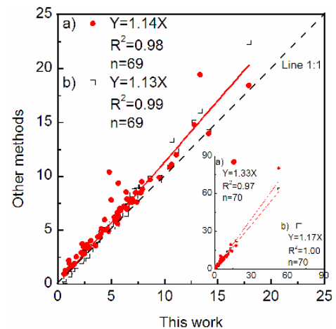
Fig. 3. Comparison of the estimated fine soil concentrations ( \mu\text{g m}^{-3} ) between Eq. (4) (this work) and a) Eq. (5) and b) Eq. (6), respectively.
