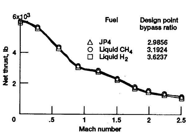
Figure 14.—Net thrust for two-spool, mixed-flow turbofan engine with CEC at 4160 °R.
