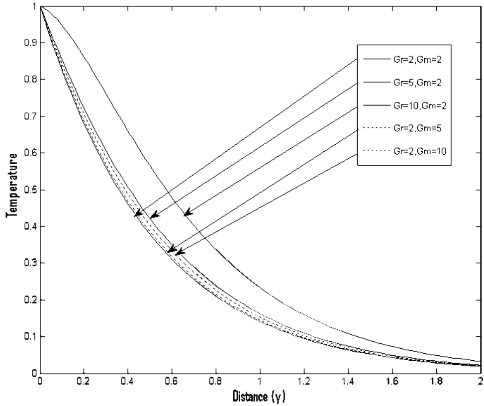
Figure 6. Effect of Gr and Gm on Temperature profile when E=0.05 , Pr=2 , Sc=2 , K=2 , h=1 , R=2 and M=2
