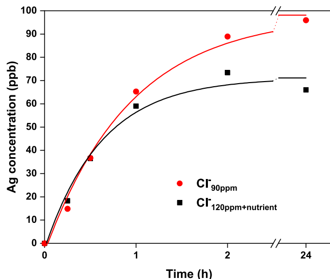
Figure 6. Silver release from cCNFAg composite (4 g/L) in Cl - 90ppm and Cl - 120ppm+nutrient simulated freshwaters. Exponential decay curves (increasing form) have been plotted to the data to guide the eye.
