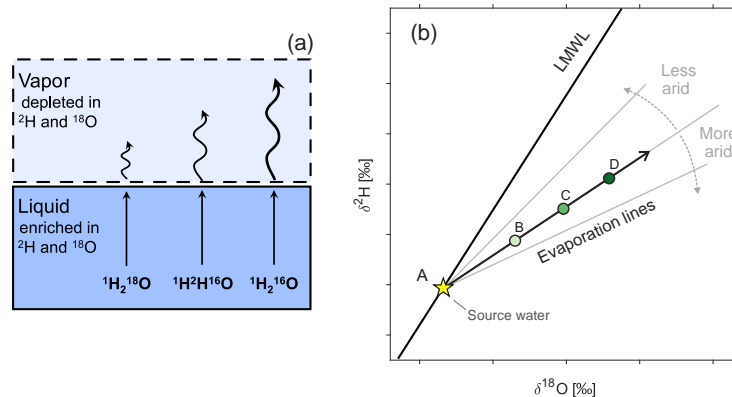
Figure 1. Fractionation effects during evaporation from an open water body. (a) Heavier water molecules ( ^1\text{H}_2^{\text{H}^{16}\text{O}} , ^1\text{H}_2^{\text{H}^{18}\text{O}} ) break their bonds and evaporate less readily than lighter water molecules ( ^1\text{H}_2^{\text{H}^{16}\text{O}} ), and thus have lower saturation vapor pressures. Heavier molecules also diffuse away from the evaporating surface less rapidly. As a consequence, during evaporation, lighter water molecules vaporize faster than heavier water molecules. The ratios between the evaporation rates of the different water isotopologues (net of any condensation) determine the slope of the evaporation line describing the progressive isotopic enrichment of the liquid water that is left behind. (b) Progressive enrichment (dots B–D) of a water source (yellow star A). The evaporation line typically lies below the local meteoric water line (LMWL), at an angle that depends on the aridity and the isotopic composition of the atmosphere (and thus on the relative rates of re-condensation of each isotopologue). (a) was adapted from Leibundgut et al. (2009).
