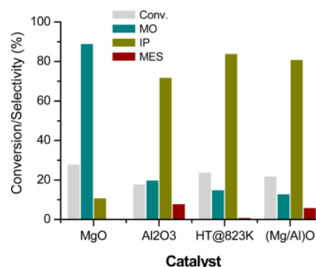
Figure 6. Comparison of different catalysts in the gas-phase condensation reaction of propan-2-one. Reaction conditions: T = 473 K, \text{WHSV} = 0.4 \text{ h}^{-1} , M_{\text{Cat}} = 0.1 \text{ g} , Q_{\text{tot}} = 150 \text{ cm}^3 \text{ min}^{-1} .
