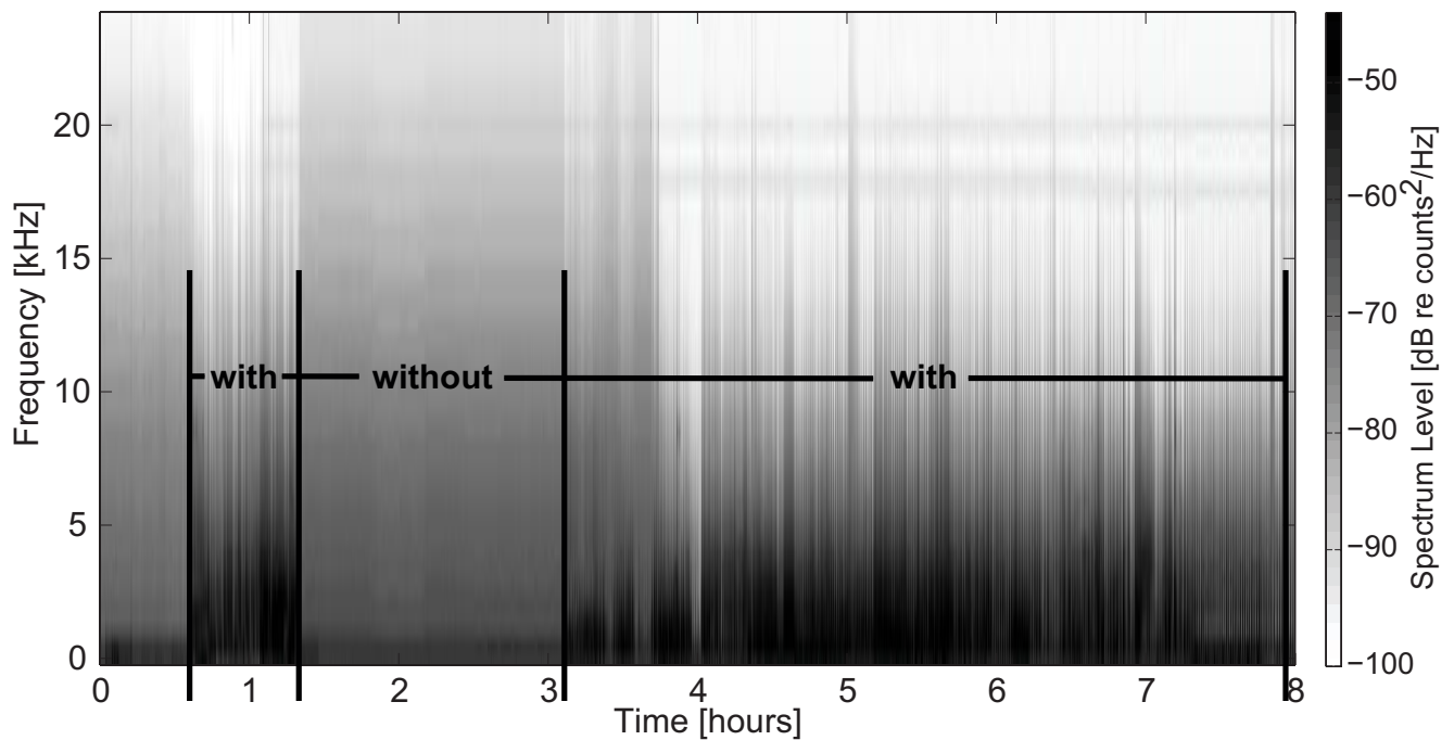
Figure 2. A long-term spectral average (LTSA) for 20 August 2009. The LTSA provides an overall picture of acoustic activity at the Marine Terminal Redevelopment Project on a daily basis. Example times “with” and “without” construction activity are marked.
