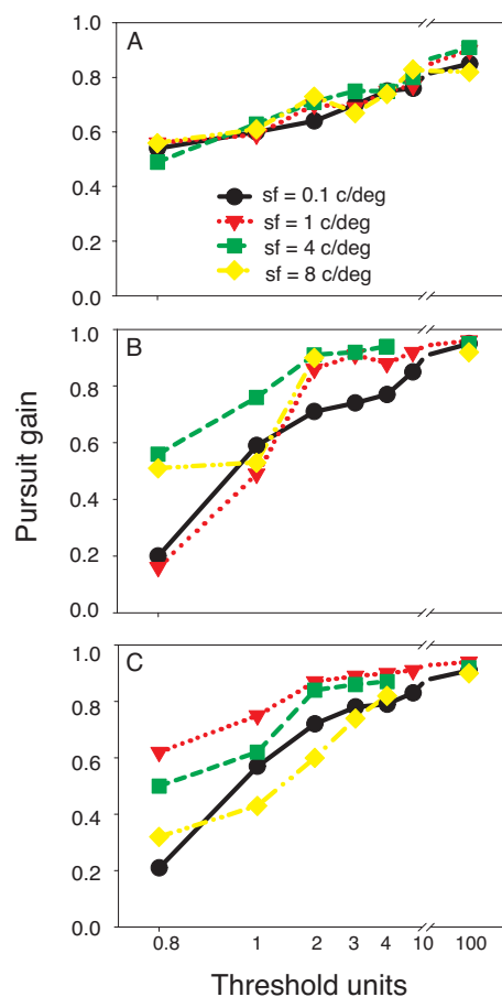
Figure 5. Means for smooth pursuit gain for three stimulus velocities (from a to c: 1, 8, and 15 deg/s) and seven threshold units. Different line colors indicate the four spatial frequencies.
