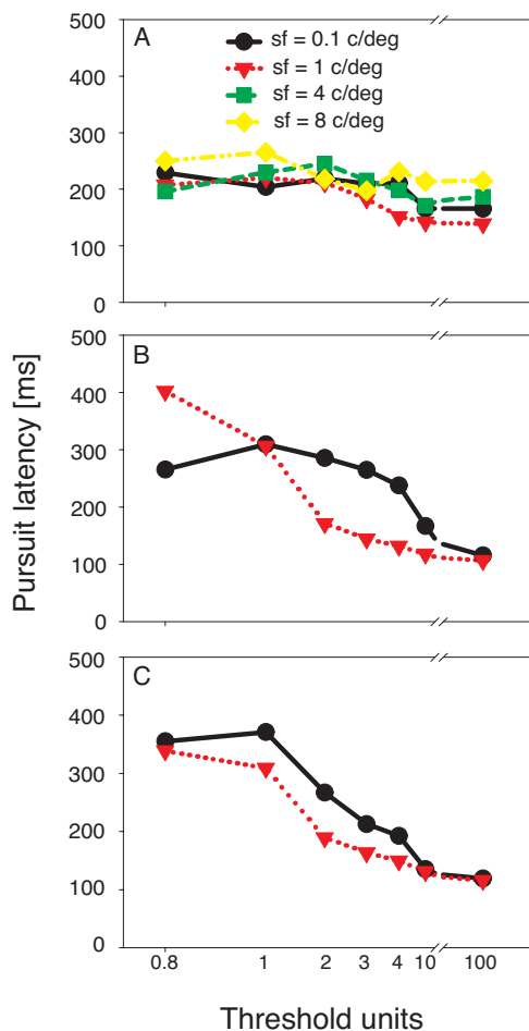
Figure 6. Means for smooth pursuit latency for three stimulus velocities (from a to c: 1, 8, and 15 deg/s) and seven threshold units. Different line colors indicate the four spatial frequencies.
