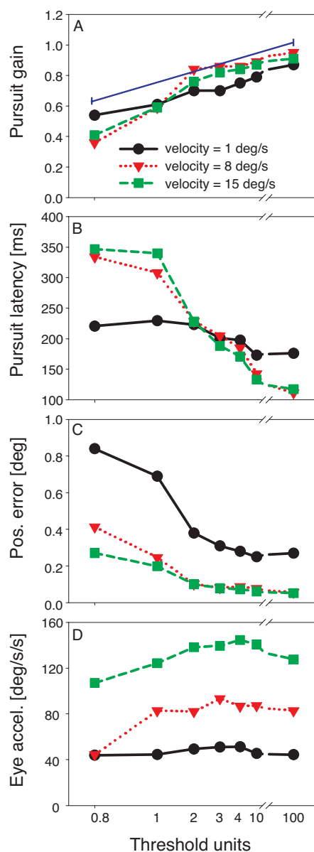
Figure 9. Means for smooth pursuit gain (a), latency (b), position error (c), and initial acceleration (d) for three stimulus velocities (1, 8, and 15 deg/s), as indicated by the line colors, and seven threshold units. The blue regression line in Figure 9a indicates perceptual data from a previous study by Gegenfurtner and Hawken (1996). Depicted is the fitted regression line to mean values (four subjects) for effects of contrast on perceived velocity of gratings moving at 1 Hz.
