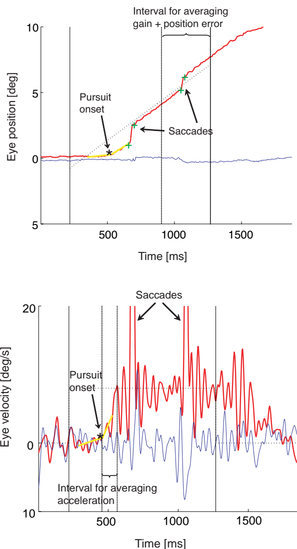
Figure 3. Example position (top) and velocity trace (bottom) to demonstrate time intervals during the stimulus duration that were used for analyzing pursuit characteristics.
