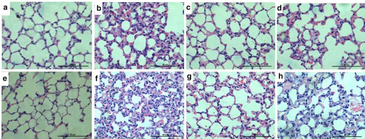
Fig. 1 Left lung tissue paraffin section with HE staining ( \times 400 ). a Control group days 15 after irradiation. b RT group days 15 after irradiation. c CpG group days 15 after irradiation. d RT+CpG group days 15 after irradiation; e Control group days 30 after irradiation. f RT group days 30 after irradiation. g CpG group days 30 after irradiation; h RT+CpG group days 30 after irradiation
