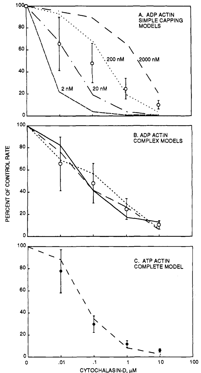
FIGURE 5: Theoretical curves for the dependence of the elongation rate at the barbed end of actin filaments upon the concentration of cytochalasin D. The experimental data \pm 1 standard deviation are reproduced from Figure 1. (A) Attempts to fit the data for ADP-actin with the simple capping mechanism (model 1 in the text) with a range of equilibrium constants K 2 for CD binding to the barbed end. The four theoretical curves from left to right correspond to K 2 = 2, 20, 200, and 2000 nM. (B) Theoretical curves for elongation by ADP-actin calculated by using three different mechanisms: the solid line is the incomplete capping (model 2 in the text); the dotted line is capping by two CD's (model 3 in the text); and the dashed line is incomplete capping with monomer inactivation (model 4 in the text). The details of these mechanisms are discussed in the text. The rate and equilibrium constants are given in Table II and in the text. (C) Comparison of experimental data for elongation by ATP-actin with a theoretical curve calculated by kinetic stimulation using model 5, a mechanism that includes rapid hydrolysis of ATP by CD-actin dimers and partial capping of barbed ends. The rate and equilibrium constants are given in Table II.
