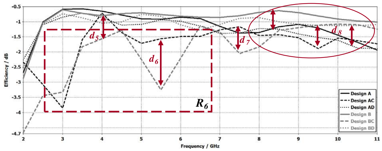
Figure 11. Simulated efficiency for Design A and Design B with waveguide and DWS.
