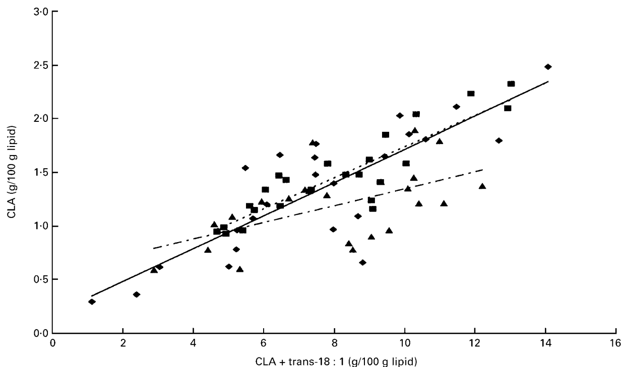
Fig. 1. Effect of breed of sheep on the relationship of muscle conjugated linoleic acid (CLA) (g/100 g lipid) to CLA + trans-18:1 (g/100 g lipid). For details of diets and procedures, see Table 1 and p. 698. (---■---), Soay lambs; (---◆---), Friesland lambs; (---▲---), Suffolk lambs.
