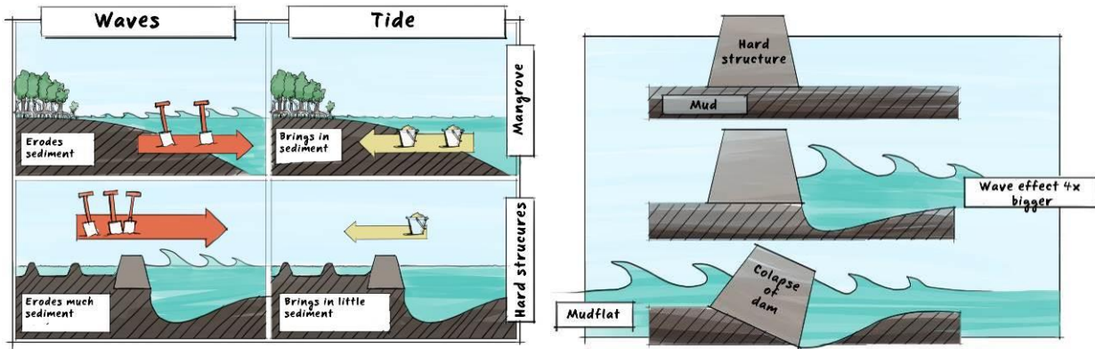
Figure 14: Graphical illustration of the sediment balance and wave height increase due to hard structures, such as concrete aquaculture dykes. Inspired by Winterwerp et al. (2013). Illustrations by Joost Fluitsma, JAM visual thinking.
