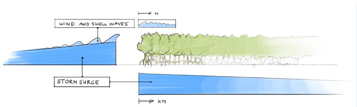
Figure 3: Mangroves significantly reduce height of wind and swell waves already within hundreds of meters, while storm surge height reduction requires mangroves with a width of several kilometres. Illustration by Joost Fluitsma, JAM visual thinking.
