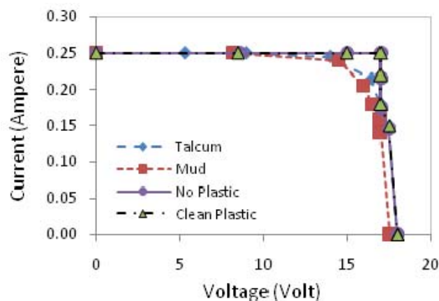
Fig. 7 I-V characteristics for irradiation of 255 W/m 2
