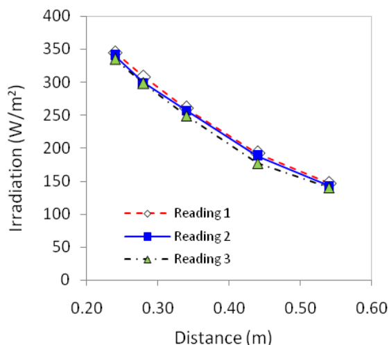
Fig. 6 Irradiation versus distance for two spotlights
