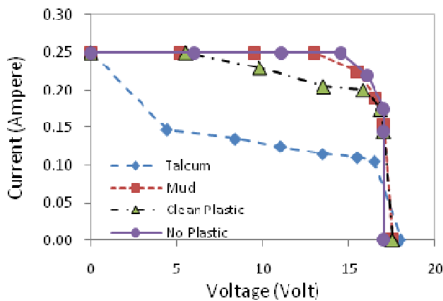
Fig. 9 I-V characteristics for irradiation of 340 W/m 2
