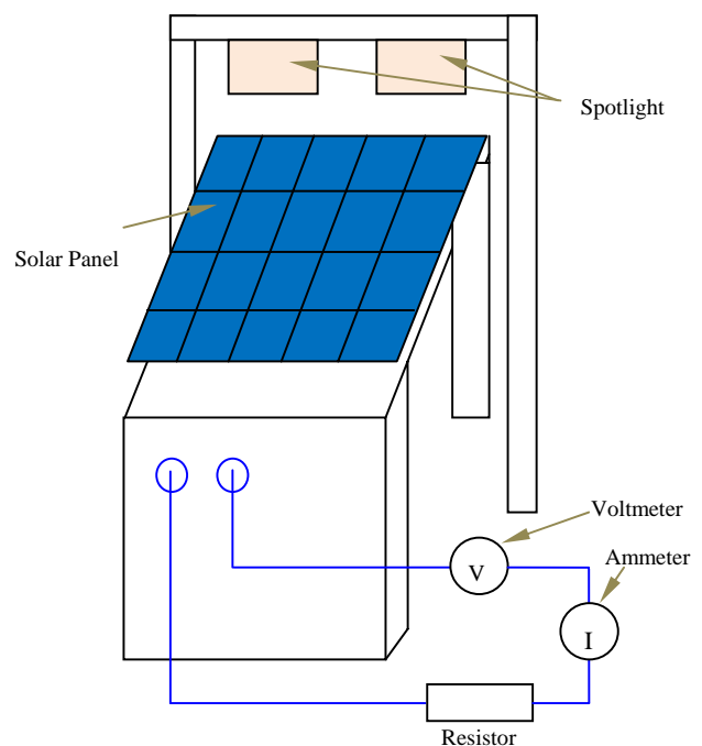
Fig. 1 Schematic of the system
