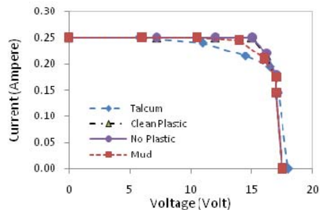
Fig. 8 I-V characteristics for irradiation of 301 W/m 2
