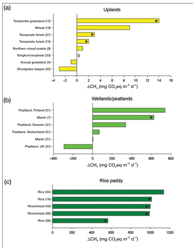
Figure 3. Effects of elevated \text{CO}_2 on net \text{CH}_4 emissions in (a) uplands, (b) wetlands/peatlands, and (c) rice paddy fields. Effects of elevated \text{CO}_2 are expressed in \text{mg CO}_2\text{eq m}^{-2} \text{d}^{-1} ( \Delta\text{CH}_4 = absolute difference in the \text{CH}_4 flux between elevated and ambient \text{CO}_2 ). Bars with asterisks indicate that the effect of elevated \text{CO}_2 was significant ( P < 0.05 ). If other treatments were included in the study, effects of elevated \text{CO}_2 were calculated across those treatments. Numbers in parentheses after the ecosystem type refer to reference numbers in WebTable 1.
