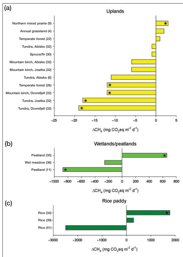
Figure 5. Effects of elevated temperature on net \text{CH}_4 emissions in (a) uplands, (b) wetlands/peatlands, and (c) rice paddy fields. Effects of warming are expressed in \text{mg CO}_2\text{eq m}^{-2} \text{d}^{-1} ( \Delta\text{CH}_4 = absolute difference in the \text{CH}_4 flux between elevated and ambient temperature). Bars with asterisks indicate that the effect of warming was significant ( P < 0.05 ). If other treatments were included in the study, effects of warming were calculated across those treatments. Numbers in parentheses after the ecosystem type refer to reference numbers in WebTable 1.
