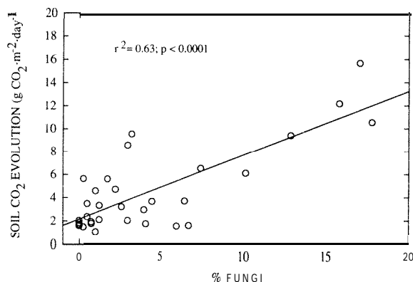
Fig. 3. Relationship between percent fungi (percent occurrence in minirhizotron frames) and soil CO 2 evolution across all treatments and sampling periods. Analyses were performed on mean values ( n = 3 for all treatments except chamberless, where n = 2 ).
