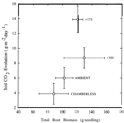
Fig. 1. Total root biomass versus soil CO 2 evolution in October 1993. Data are means (averaged across N) and standard errors.
