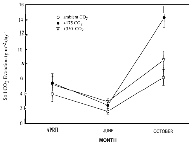
Fig. 2. Seasonal variation in mean soil CO 2 evolution by CO 2 treatment. Data are means (averaged across N) and standard errors.
