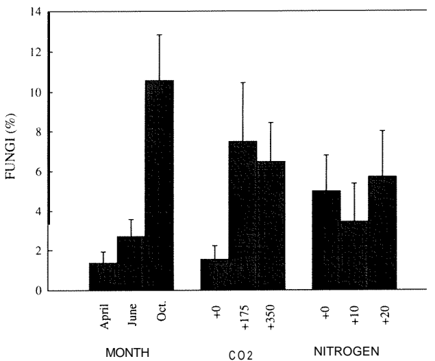
Fig. 4. Variation in percent fungi (percent of occurrence in minirhizotron frames) by month (averaged across CO 2 and N), CO 2 treatment (averaged across months and N), and N (averaged across months and CO 2 ). Data are means and standard errors.
