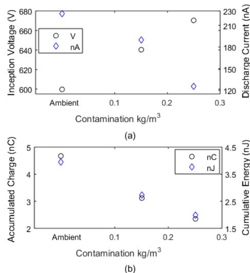
FIGURE 15. PD quantities measured for different contamination levels at 90% RH, ambient pressure and temperature (a) inception voltage and discharge current, (b) accumulated charge and cumulative energy.
