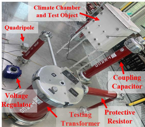
FIGURE 5. PD measurement set-up established in the laboratory.
