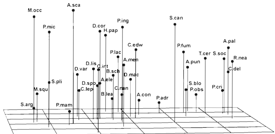
Fig. 3. Three-dimensional MDS configuration of species similarity matrix (stress = 0.09). Values of Ascidella aspersa and Molgula bleizeii were removed previous to analyses. Species names are abbreviated from Table 1
