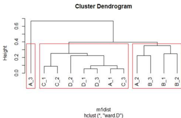
Fig. 3 Cluster analysis results (cluster dendrogram)
