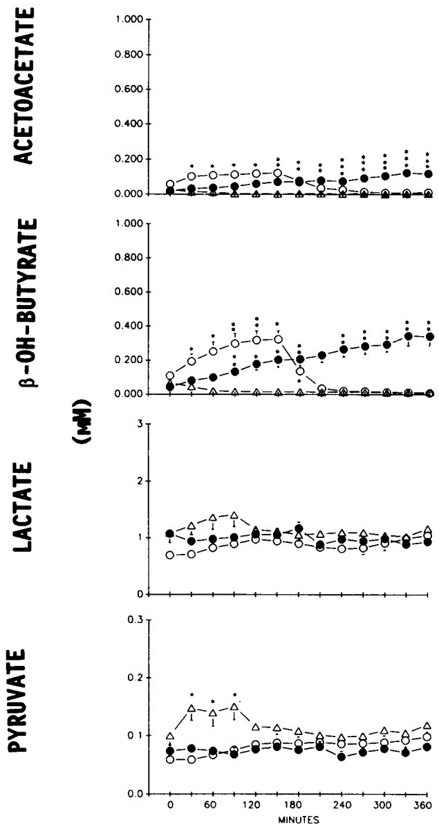
Figure 2. Acetoacetate, \beta -OH-butyrate, lactate, and pyruvate concentrations in studies 1–3. In study 1, lipid/heparin was infused from 0 to 360 min. In study 2, saline was infused from 0 to 360 min. In study 3, lipid/heparin was infused from 0 to 120 min and saline from 120 to 360 min. Symbols and numbers of experiments as in Fig. 1. All studies were performed under euglycemic hyperinsulinemic conditions. Mean \pm SE. * P < 0.05 , ** P < 0.05 , *** P < 0.005 comparing studies 1 with 2 and 3 with 2.
