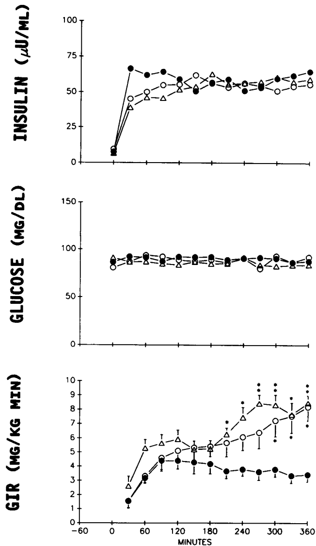
Figure 1. Peripheral venous insulin and glucose concentrations and (GIR) in healthy men during study 1 (lipid infusion during euglycemic hyperinsulinemia, ●, n = 6 ), study 2 (saline infusion during euglycemic hyperinsulinemia, ▲, n = 6 ), and study 3 (euglycemic hyperinsulinemia plus lipid from 0 to 2 h and saline from 2 to 4 h, ○, n = 6 ). * P < 0.05 , ** P < 0.01 comparing studies 2 with 1 and 3 with 1.
