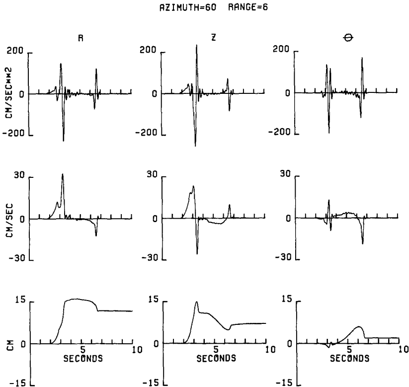
FIG. 5 Synthetic three-component ground motion for a receiver at 60^\circ and epicentral range of 6 km \nu = 0.9\beta , 0.0 \text{ Hz} \leq f \leq 5.0 \text{ Hz} .
