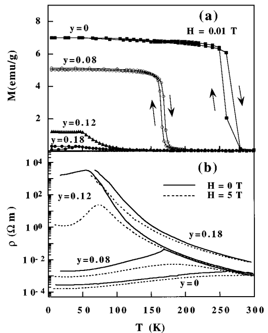
FIG. 1. Temperature dependence of (a) magnetization M in a 0.01 T field, and (b) resistivity \rho in zero (solid curves) and 5 T (dashed curves) magnetic field, for \text{La}_{0.63}\text{Ca}_{0.37}\text{Mn}_{1-y}\text{Fe}_y\text{O}_3 with y=0, 0.08, 0.12 , and 0.18 .
