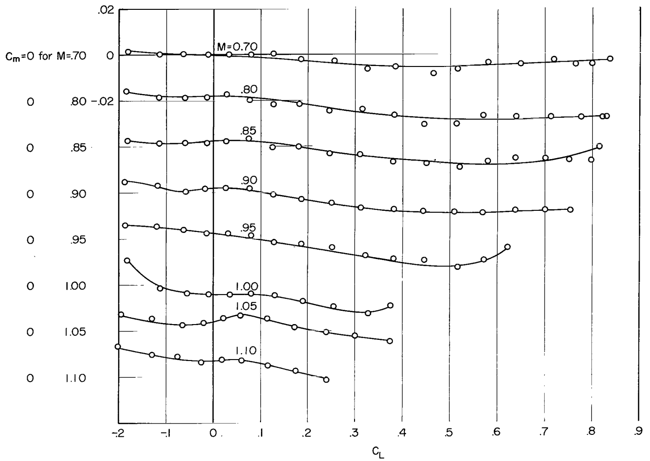
(c) Model CR. Reynolds number per meter \approx 10.5 \times 10^6 .
