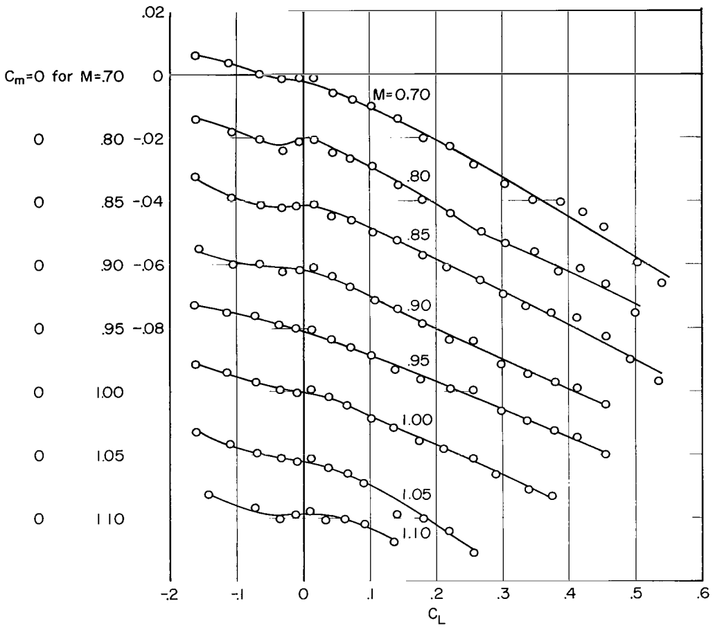
(b) Model BR. Reynolds number per meter \approx 10.5 \times 10^6 .
