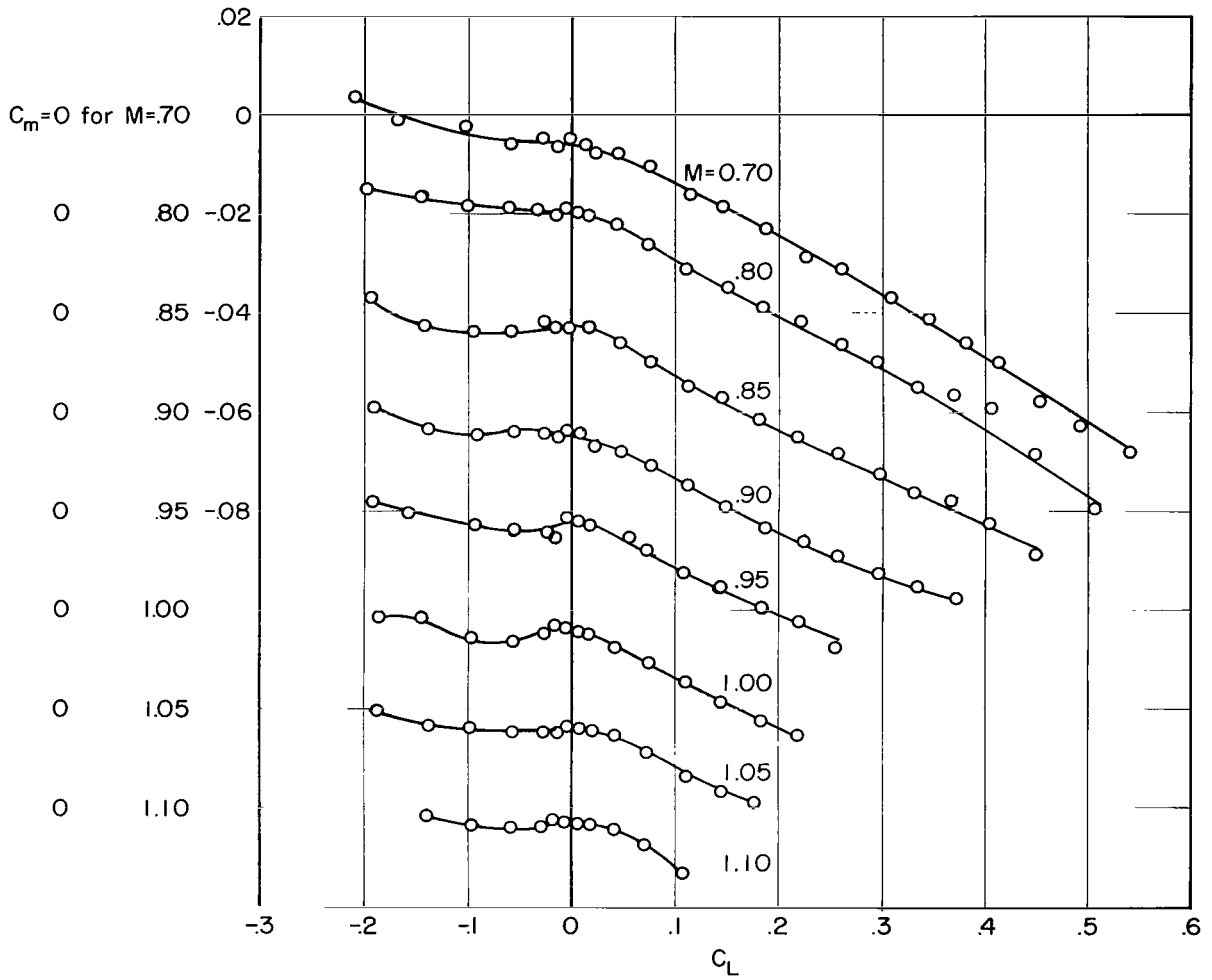
(c) Model BF. Reynolds number per meter \approx 10.5 \times 10^6 .
