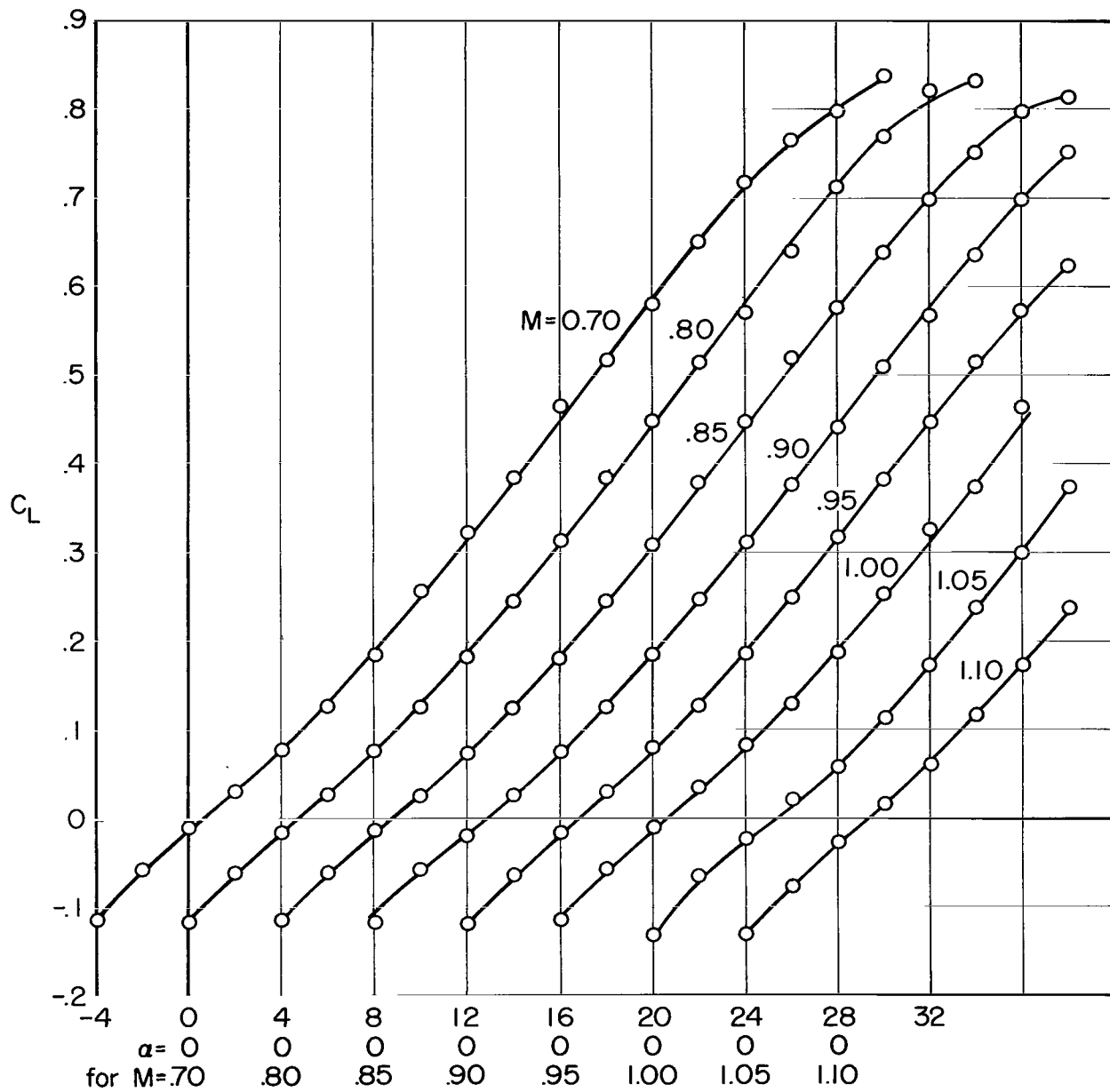
(c) Model CR. Reynolds number per meter \approx 10.5 \times 10^6 .
