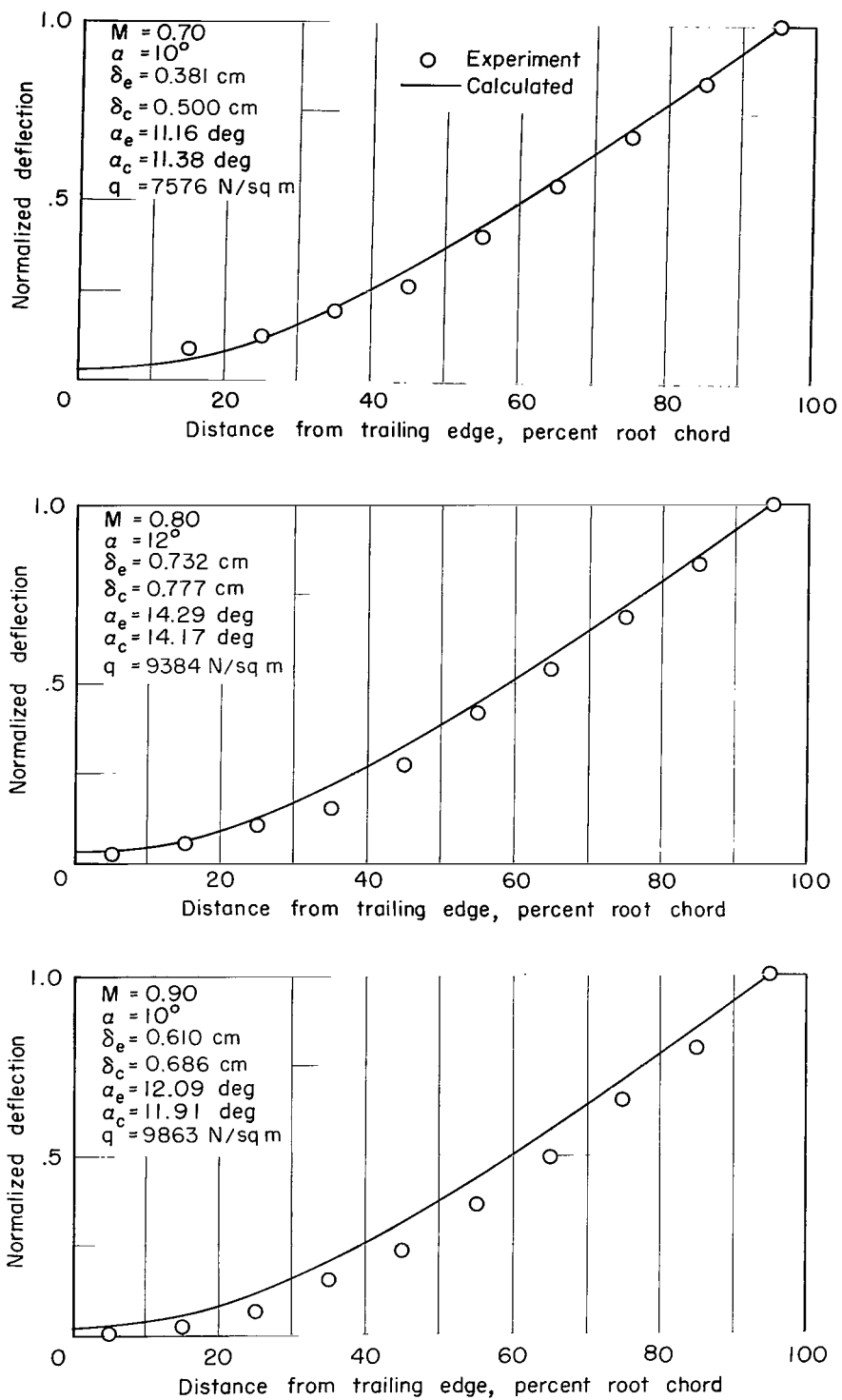
Figure 18.- Comparison of calculated and measured normalized deflection shapes for model AF-1. Reynolds number per meter \approx 10.5 \times 10^6 .
