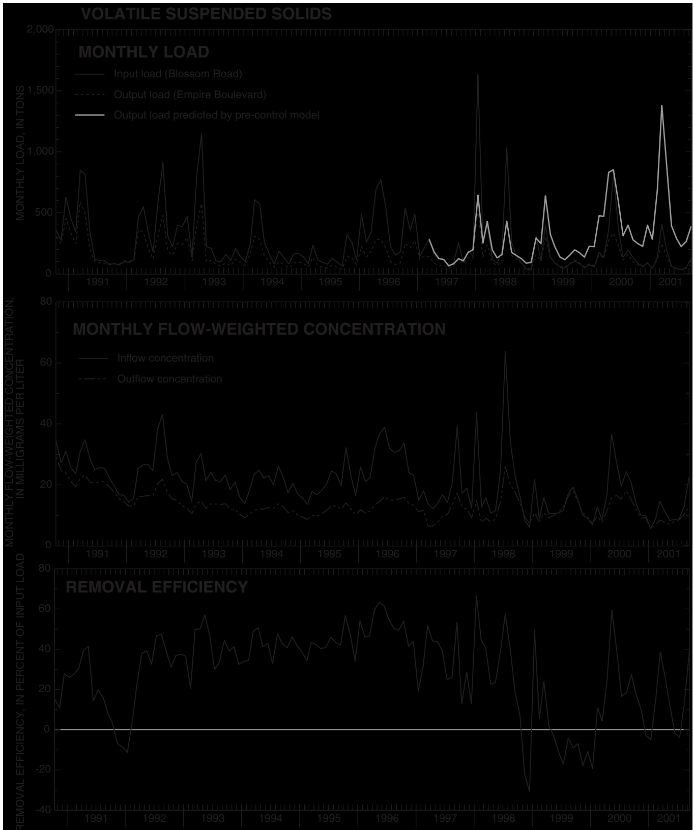
Figure 19. Monthly loads and flow-weighted concentrations, and wetland's removal efficiency for volatile suspended solids, Ellison Park wetland, Monroe County, N.Y., 1990-2001
