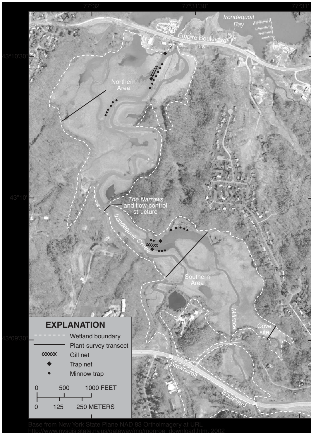
Figure 7. Locations of data-collection sites for plant and fish surveys in Ellison Park wetland, Monroe County, N.Y., 1991-2001
