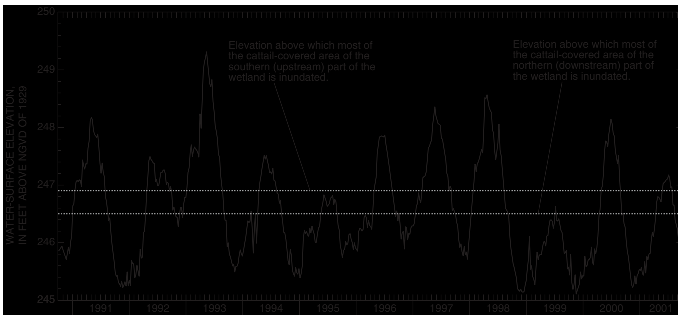
Figure 4. Daily mean water-surface elevation of Ellison Park wetland, Monroe County, N.Y., as measured at wetland outlet (Empire Boulevard), 1990-2001. (Location is shown in fig. 2.)
