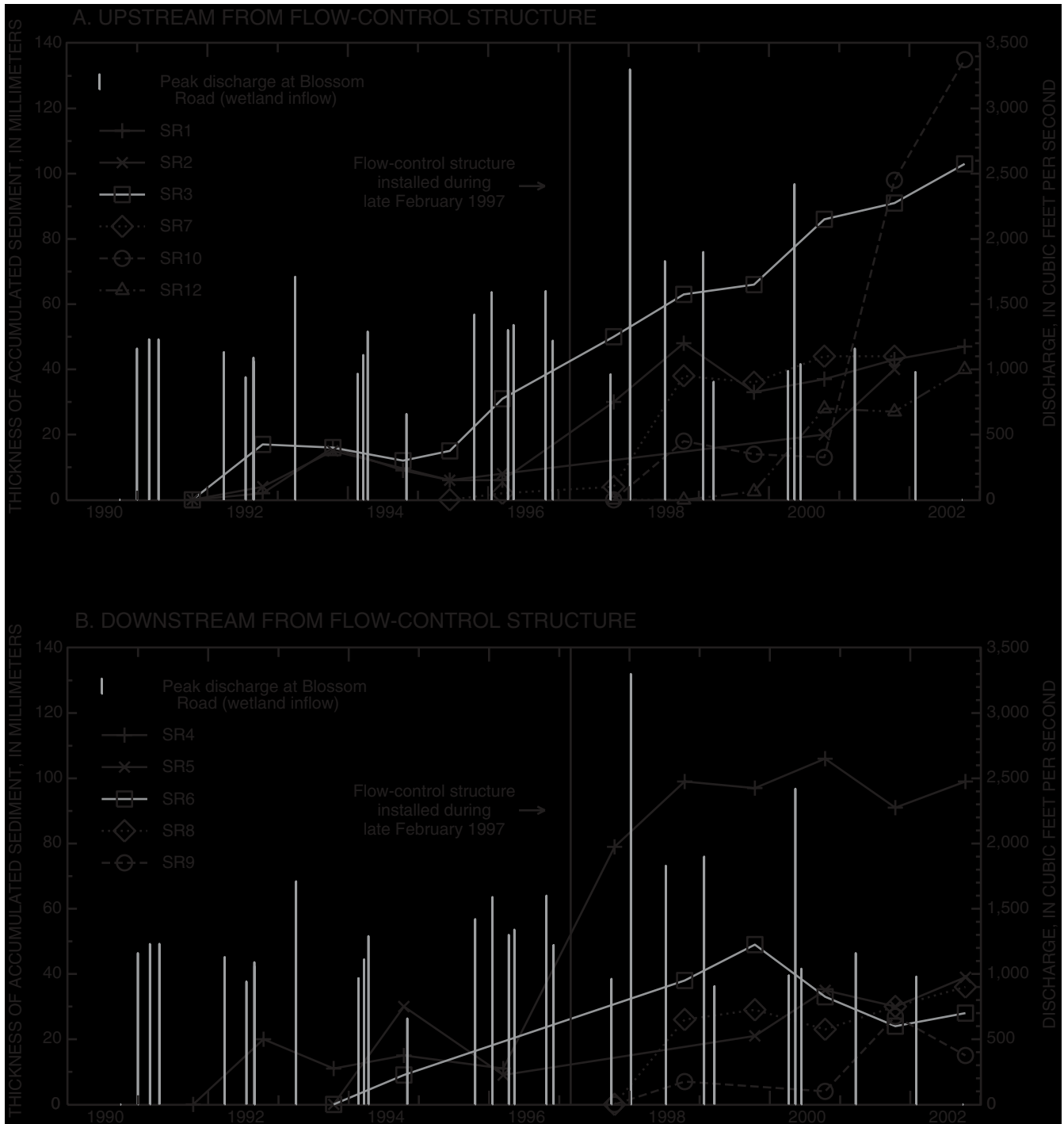
Figure 11. Thickness of accumulated sediment at sedimentation-rate-measurement sites in Ellison Park wetland, Monroe County, N.Y., 1991-2002: A. Upstream from flow control structure. B. Downstream from flow-control structure.
