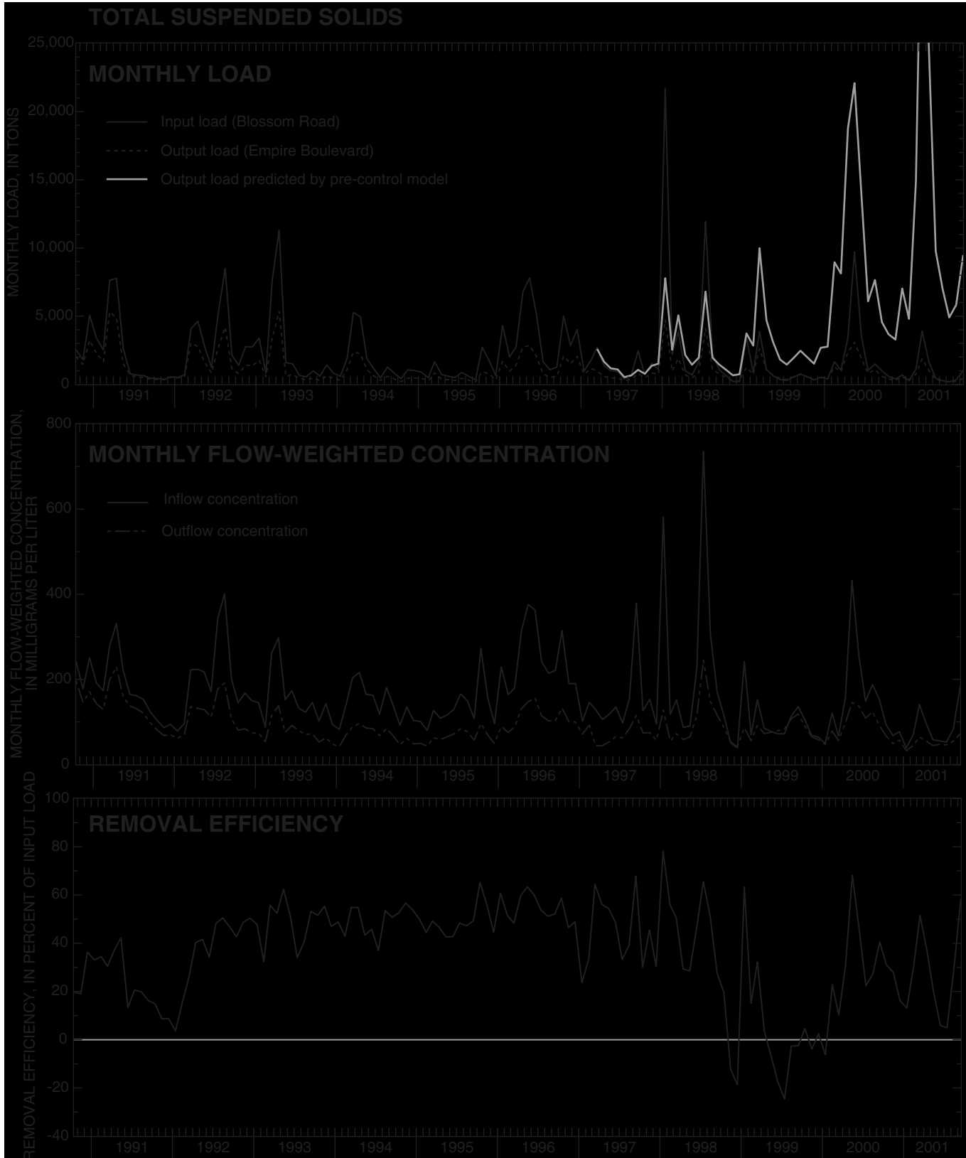
Figure 18. Monthly loads and flow-weighted concentrations, and wetland's removal efficiency for total suspended solids, Ellison Park wetland, Monroe County, N.Y., 1990-2001
