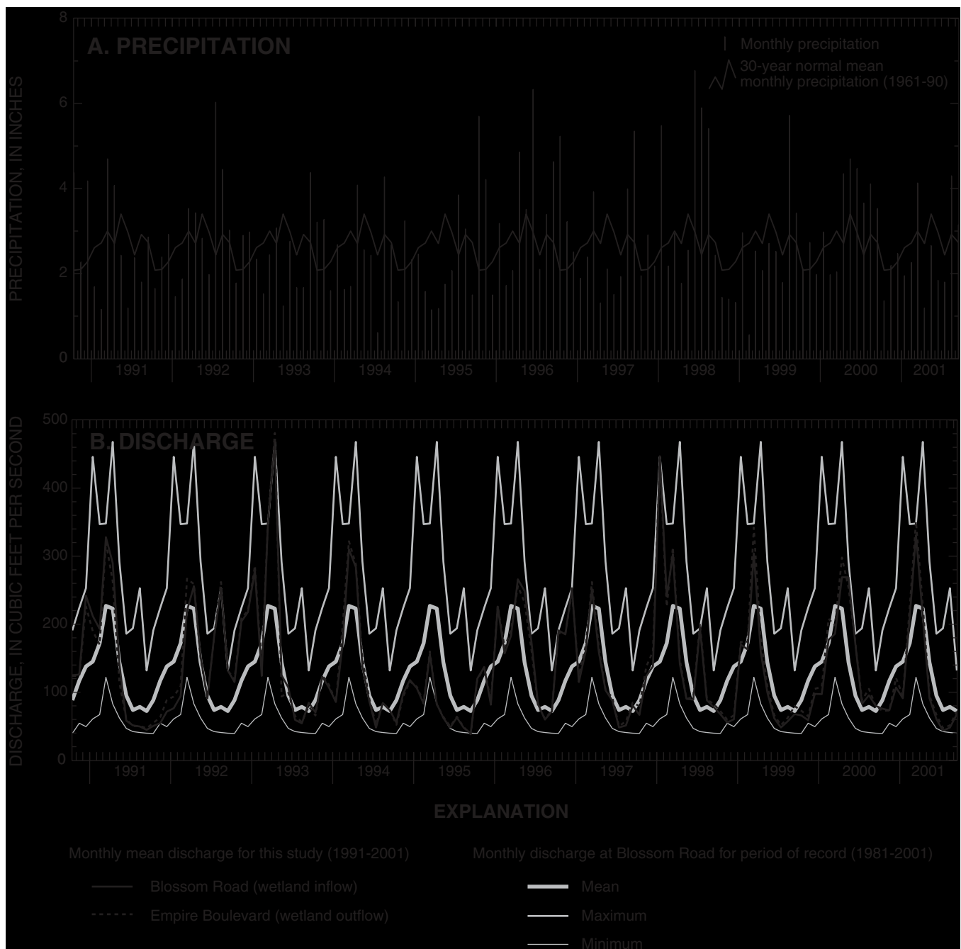
Figure 3 . A. Monthly precipitation (1990-2001) and normal mean monthly precipitation (1961-90) recorded at Greater Rochester International Airport, Rochester, N.Y. B. Monthly mean discharges of Irondequoit Creek above Blossom Road and at Empire Boulevard, Monroe County, N.Y. (1990-2001), with monthly maximum, mean, and minimum discharges for period of record at Blossom Road (1981-2001) (Locations are shown in figs. 1 and 2.)
