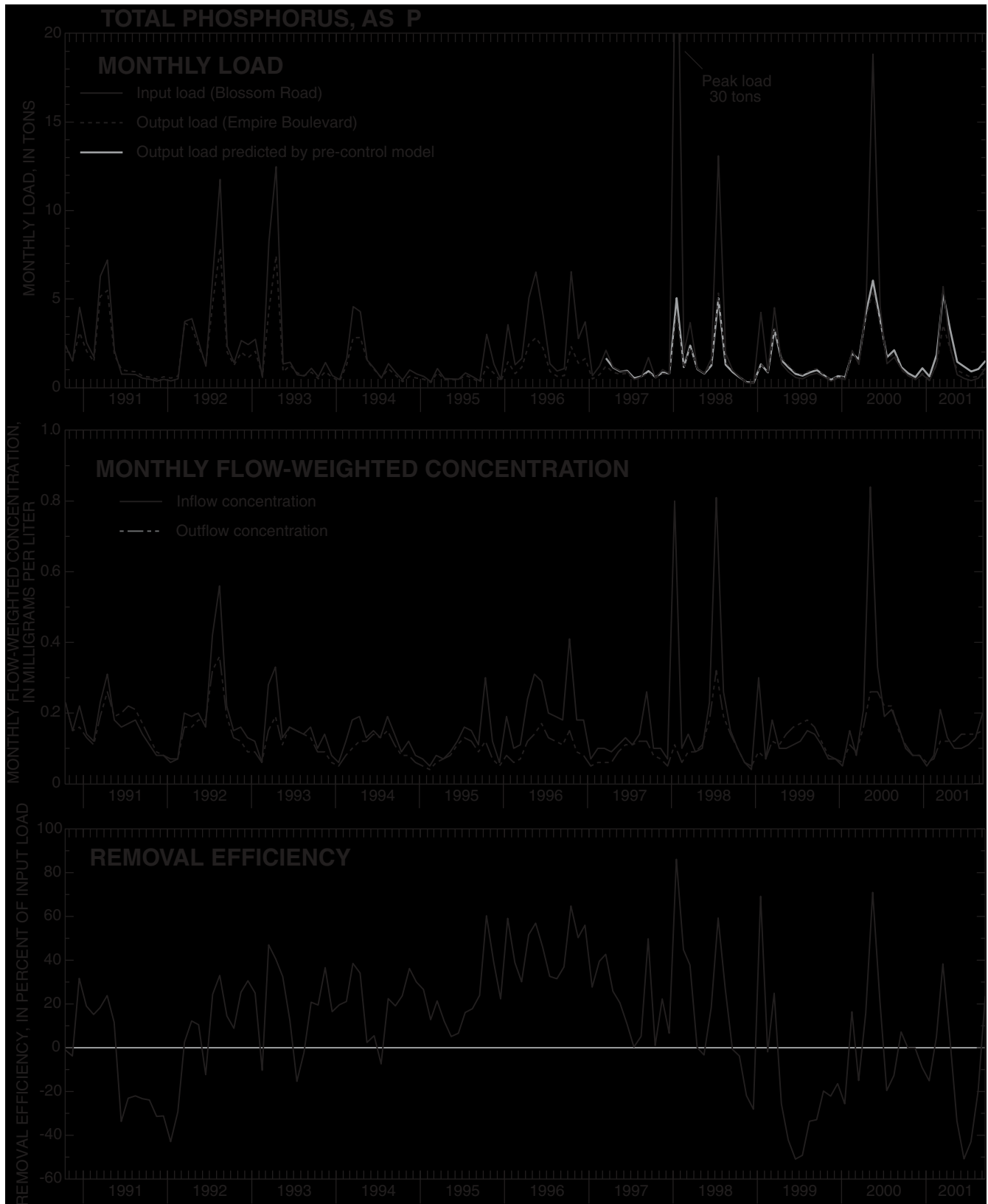
Figure 13. Monthly loads and flow-weighted concentrations, and wetland’s removal efficiency for total phosphorus, Ellison Park wetland, Monroe County, N.Y., 1990-2001
