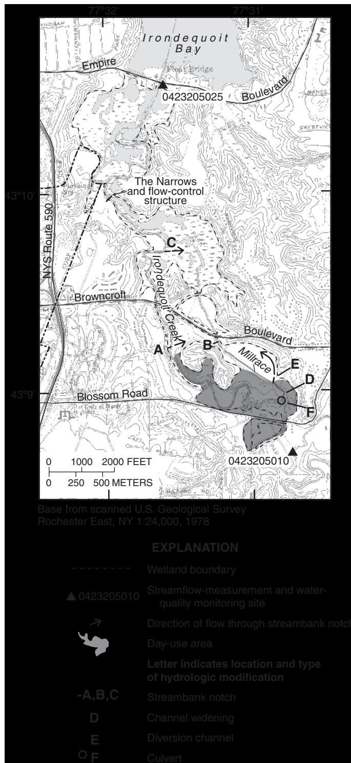
Figure 6. Locations of flow modifications to Irondequoit Creek and the Millrace, Ellison Park wetland, Monroe County, N.Y., 1997-98.
